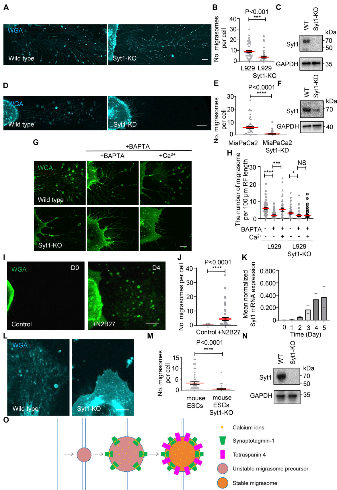
Figure 4. Syt1 is necessary for migrasome biogenesis. (A) Confocal images of migrasomes of cells derived from WT and Syt1 knockout L929. Cells are labeled with WGA (cyan). Scale bar, 10 \mu m. (B) Quantification of the number of migrasomes in WT and Syt1 knockout L929 shown in A. Data represent the
