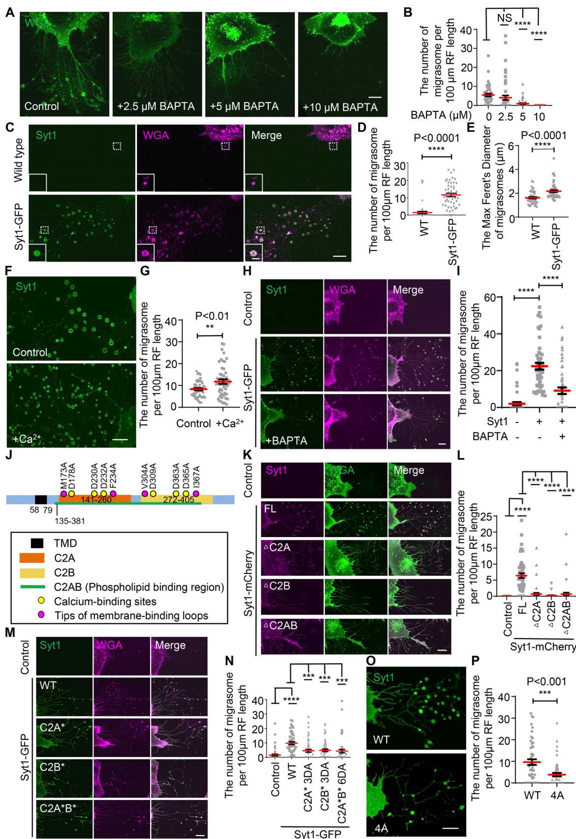
Figure 1. Ca 2+ -binding Syt1 is required for migrasome formation. (A) Confocal image of migrasomes of L929 cells treated with 0, 2.5, 5, and 10 \mu M BAPTA and cell migrate on chamber overnight for 12 h. L929 are labeled with wheat germ agglutinin (WGA) (green). Scale bar, 10 \mu m. (B) The number of migrasomes per 100 \mu m RF length per cell from images like those shown in A was quantified. Data shown represent the mean \pm SEM; P values were calculated using a two-
