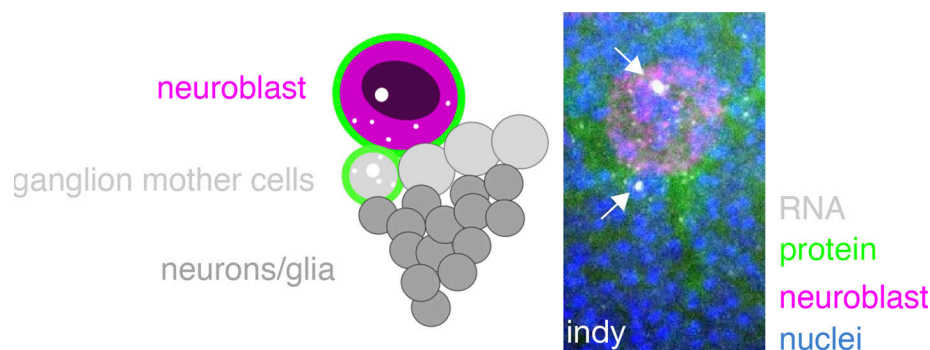
Figure S3. Rare example of highly developmental stage-specific gene expression in the neuroblast lineage. Indy , a plasma membrane transporter for Kreb's cycle intermediates, is highly transcribed (note arrows pointing to large, white punctae) in the neuroblast and a single ganglion mother cell (GMC). Indy mRNA and protein are found at low levels in older GMCs, but not in the differentiating neurons/glia.
