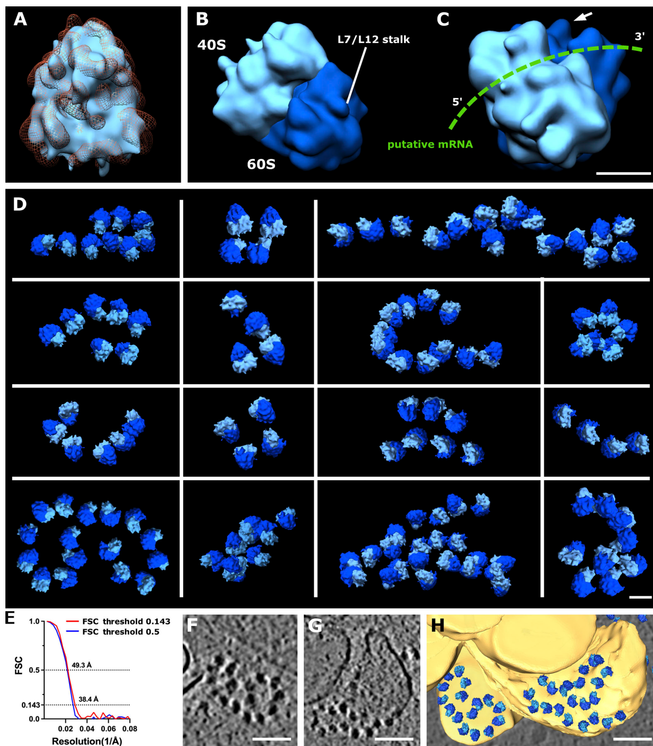
Figure 5. Ribosome reconstruction and polysome orientation. (A) Reconstructed ribosome (light blue) fitted into the 80S ribosome volume from EMD-3420 (orange mesh). (B) Reconstructed ribosome volume with depicted 40S (light blue) and 60S (dark blue) subunits and L7/L12 stalk. (C) Rotated view of ribosome from B. Putative path of mRNA depicted in green; white arrow shows L7/L12 stalk. (D) Polysomes found in various tomograms. (E) Estimation of reconstructed ribosome resolution, FSC curve. (F and G) Slices from tomogram of ribosomes on the surface of ER. (H) Segmented view of F and G. Scale bars: 10 nm (A–C); 25 nm (D); 100 nm (F–H).
