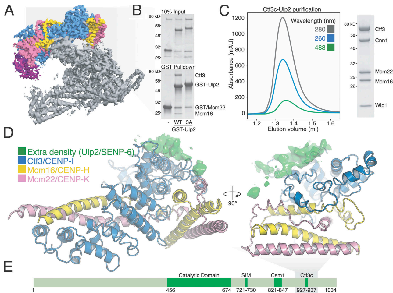
Figure 1. Reconstitution and structure of the Ctf3c-Ulp2 complex. (A) Model of the assembled Ctf3c-Ulp2 complex (Ctf3, blue; Ulp2, pink; Cnn1/Wip1, purple; Chl4, Iml3, Ctf19, Mcm21, Ame1, Okp1, Nkp1, Nkp2, gray; and EMD-0523, EMD-21910; Hinshaw and Harrison, 2019; Hinshaw and Harrison, 2020). (B) The Ctf3c binds the Ulp2-KIM but not the Ulp2-KIM-3A peptide. Purified Ctf3c and GST-Ulp2-KIM were mixed and subjected to pulldown on glutathione beads. Input and pulldown samples were analyzed by SDS-PAGE. (C) Purification of the Ctf3c-Ulp2-KIM complex by size exclusion chromatography. Absorbance wavelengths are indicated (mAU, milli-absorbance units). 488 nm reports on the FITC-Ulp2-KIM peptide. Eluate from the peak fractions were analyzed by SDS-PAGE. (D) Structure of the Ctf3c-Ulp2 complex. Extra density corresponding to Ulp2-KIM is shown as a green surface derived from the final density map. (E) Domain diagram of Ulp2. Regions with known functions are annotated.
