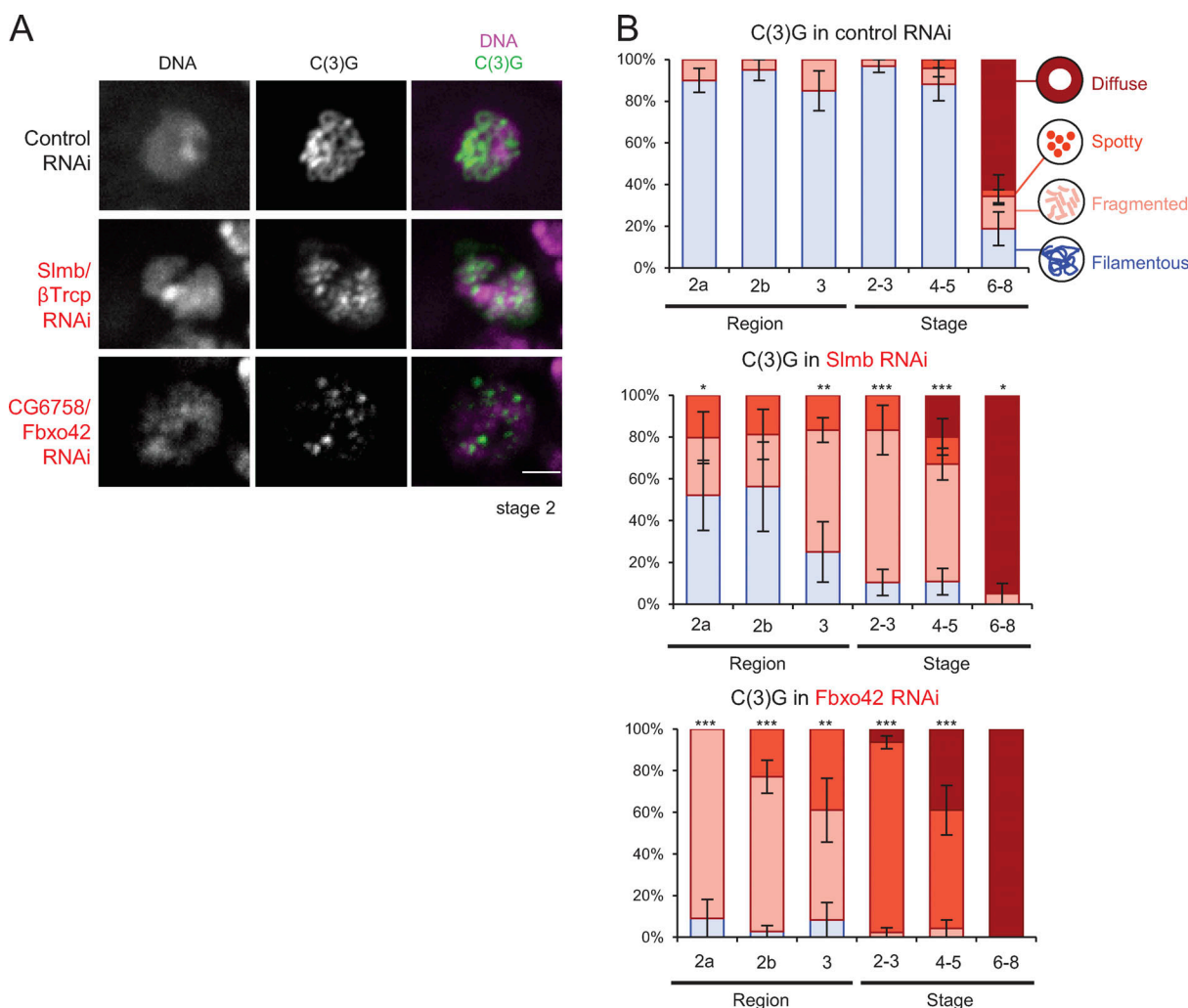
Figure 3. SCF complexes containing Slmb /βTrcp or CG6758 / Fbxo42 mediate regulation of the synaptonemal complex. (A) The synaptonemal complex component C(3)G and DNA in control, Slmb /βTrcp, and Fbxo42 RNAi throughout meiotic progression. Scale bar = 2 μm. (B) C(3)G localization patterns in control, Slmb /βTrcp RNAi, and Fbxo42 RNAi. Error bars represent SEM from triplicated experiments representing 20–31 germaria/oocytes for each region/stage. *, P < 0.05 ; **, P < 0.01 ; ***, P < 0.001 .
