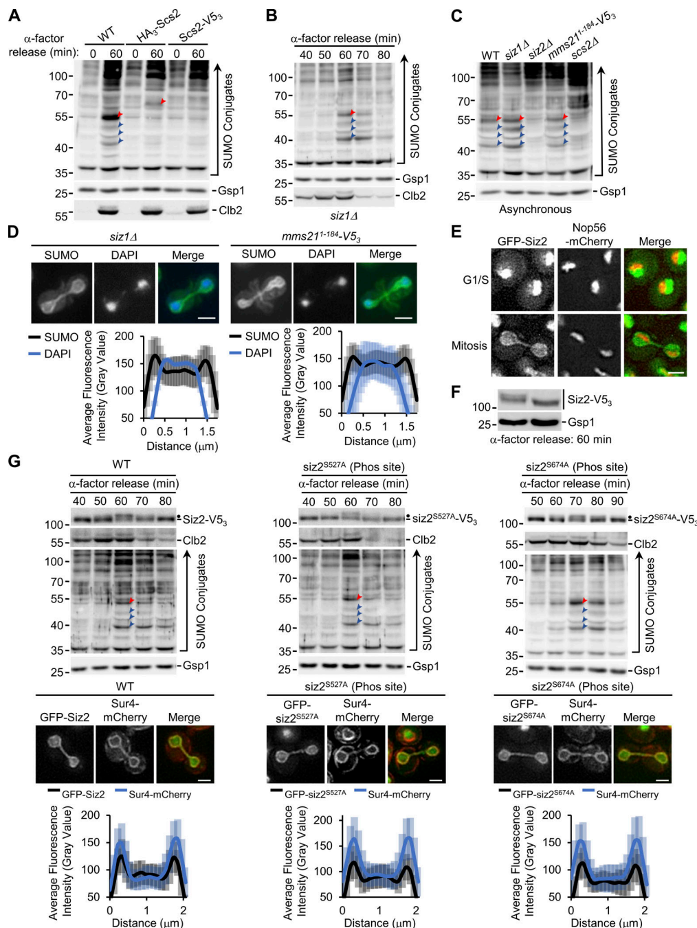
Figure S1. Siz2 localization and PTM. (A, B, and G) α-factor arrest-release assays were performed as in Fig. 1. Shown are WT cells and cells producing HA 3 -Scs2 or Scs2-V5 3 (A), siz1Δ cells (B), and Siz2-V5 3 , siz2 S527A -V5 3 , and siz2 S674A -V5 3 -producing cells (G). Cell lysates were analyzed by Western blotting using anti-SUMO, Clb2, and Gsp1 (load control) antibodies, as well as a V5 antibody in G, as indicated. Only the 0- and 60-min time points were analyzed in A. (C) Cell lysates derived from asynchronous cultures of WT, siz1Δ , siz2Δ , and mms21 1-184 -V5 3 (Mms21 derivative deficient in SUMO E3 ligase activity) cells were assessed by Western blotting using an anti-SUMO antibody to assess SUMO conjugate profiles. Gsp1 is a loading control. In A–C and G, red arrowheads point to SUMOylated Scs2 or SUMOylated tagged Scs2. Blue arrowheads point to other prominent mitotic SUMO conjugates. In G, dots highlight the position of mitotically phosphorylated Siz2-V5 3 . Molecular mass markers are shown in kD. (D) Anti-SUMO immunofluorescence analysis of siz1Δ and mms21 1-184 -V5 3 cells was performed as described in Fig. 1. DAPI staining identifies nuclear position. Imaging and quantification of the nuclear distribution of SUMO in mitotic cells ( n = 25 ) were performed as in Fig. 1. (E) Shown are epifluorescence images of representative G1/S- and M-phase WT cells producing GFP-Siz2 and nucleolar Nop56-mCherry. Merged images show that GFP-Siz2 is largely excluded from the nucleolus. (F) WT mitotic cell lysates were isolated at 60 min after release from α-factor arrest (see Fig. 1B). Proteins were extracted and solubilized in buffer lacking (-PPase) or containing protein phosphatase (+PPase). Samples were analyzed by Western blotting using anti-V5 and Gsp1 (loading control) antibodies. Mobility of modified Siz2-V5 3 is increased by phosphatase treatment. Vertical line indicates that all bands observed consist of Siz2-V5 3 . (G) Imaging and quantification of the nuclear distribution of GFP-Siz2, GFP- siz2 S527A , and GFP- siz2 S674A compared with Sur4-mCherry were examined as described in Fig. 3 for cells ( n = 25 ) in mitosis. Note, line scans show enrichment of Siz2-GFP, GFP- siz2 S527A , and GFP- siz2 S674A at the NE with Sur4-mCherry in these cells. Quantification of line scans shown in G were obtained at the same time as data shown in Fig. 3 C, and the WT data are also shown here for comparison. Error bars represent SD. Bar, 2 μm. Phos, phosphorylation.
