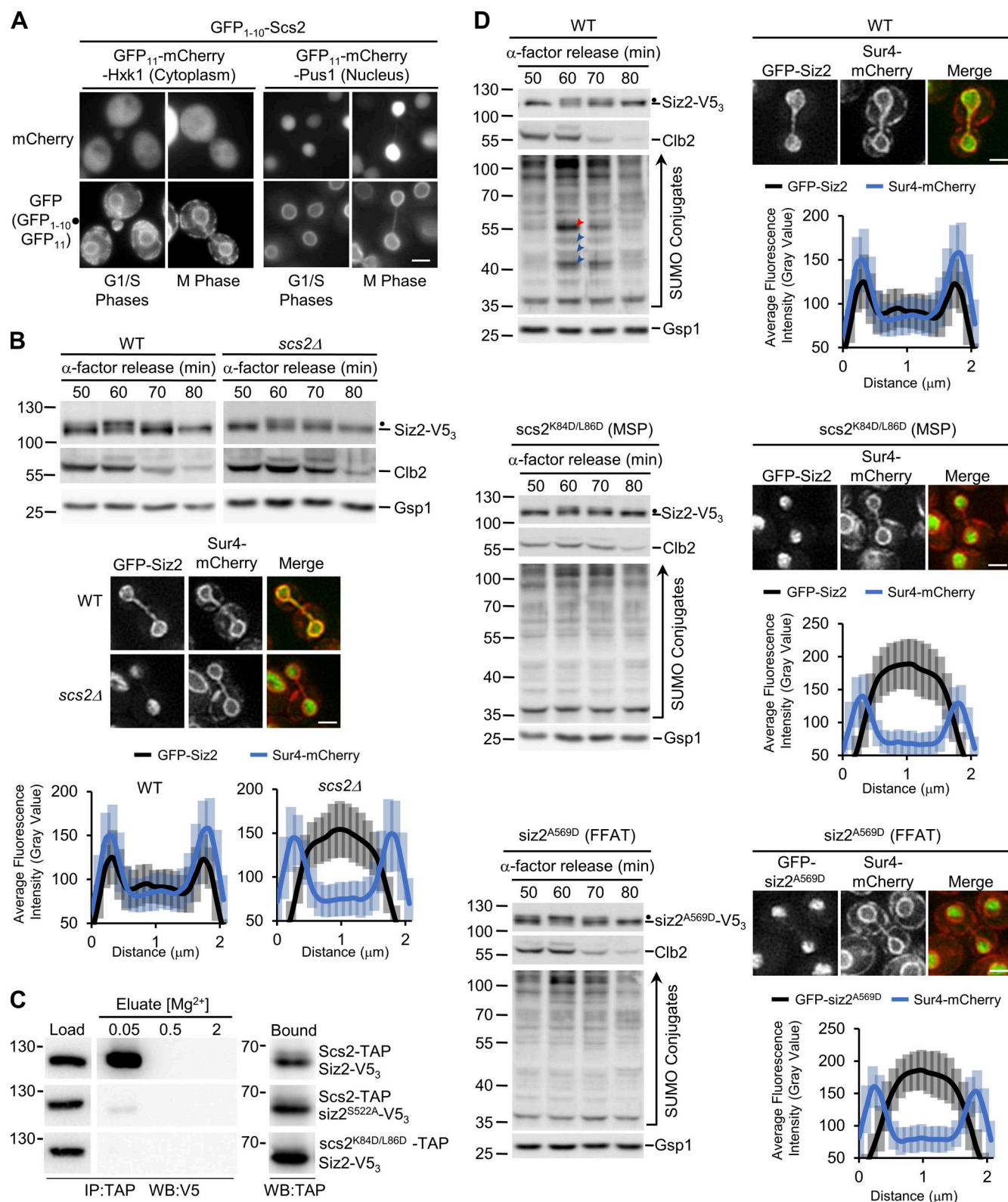
Figure 4. INM association of Scs2-Siz2 directs mitosis-specific SUMOylation events. (A) Scs2 localization was assessed using the split-superfolder GFP system. Epifluorescence images of WT cells containing GFP 1-10 -Scs2 and plasmid-encoded GFP 11 -mCherry-Hxk1(cytoplasmic) or GFP 11 -mCherry-Pus1 (nuclear). Localization of the reporter (mCherry) and assembled GFP 1-10 -GFP 11 (GFP) in representative G1-, S-, and M-phase cells is shown. Bar, 2 μm. Dot represents association of the GFP fragments. (B and D) The indicated strains were assessed for Siz2-V5 3 phosphorylation and their mitotic SUMO conjugate profile by Western blot analysis as described in Fig. 1 and Fig. 2. Dots highlight the position of mitotically phosphorylated Siz2-V5 3 . GFP-Siz2 and Sur4-mCherry imaging and quantification of the nuclear distribution were performed on mitotic cells of the specified strains as described in Fig. 3. Note, quantification of line scans shown in panels B and D was obtained at the same time as data shown in Fig. 3 C, and the WT data are also shown here for comparison. The scs2 K84D/L86D
