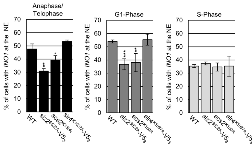
Figure 8. NPC association of activated INO1 requires the Scs2 - Siz2 complex and Scs2 SUMOylation. NE localization of the activated INO1 locus was examined using epifluorescence imaging. The graphs show the percentage of total GFP-lac/ INO1 - LacO 256 foci that co-localize with NE localized Nup49-RFP. For each indicated strain, three biological replicates were assessed. Cell cycle stage was determined using bud size and nuclear morphology. n = 50 cells/replicate/cell cycle stage. Error bars represent SD. Asterisks: significant change relative to WT using a two-tailed Student's t test. *, P ≤ 0.05; **, P ≤ 0.01; ***, P ≤ 0.001.
