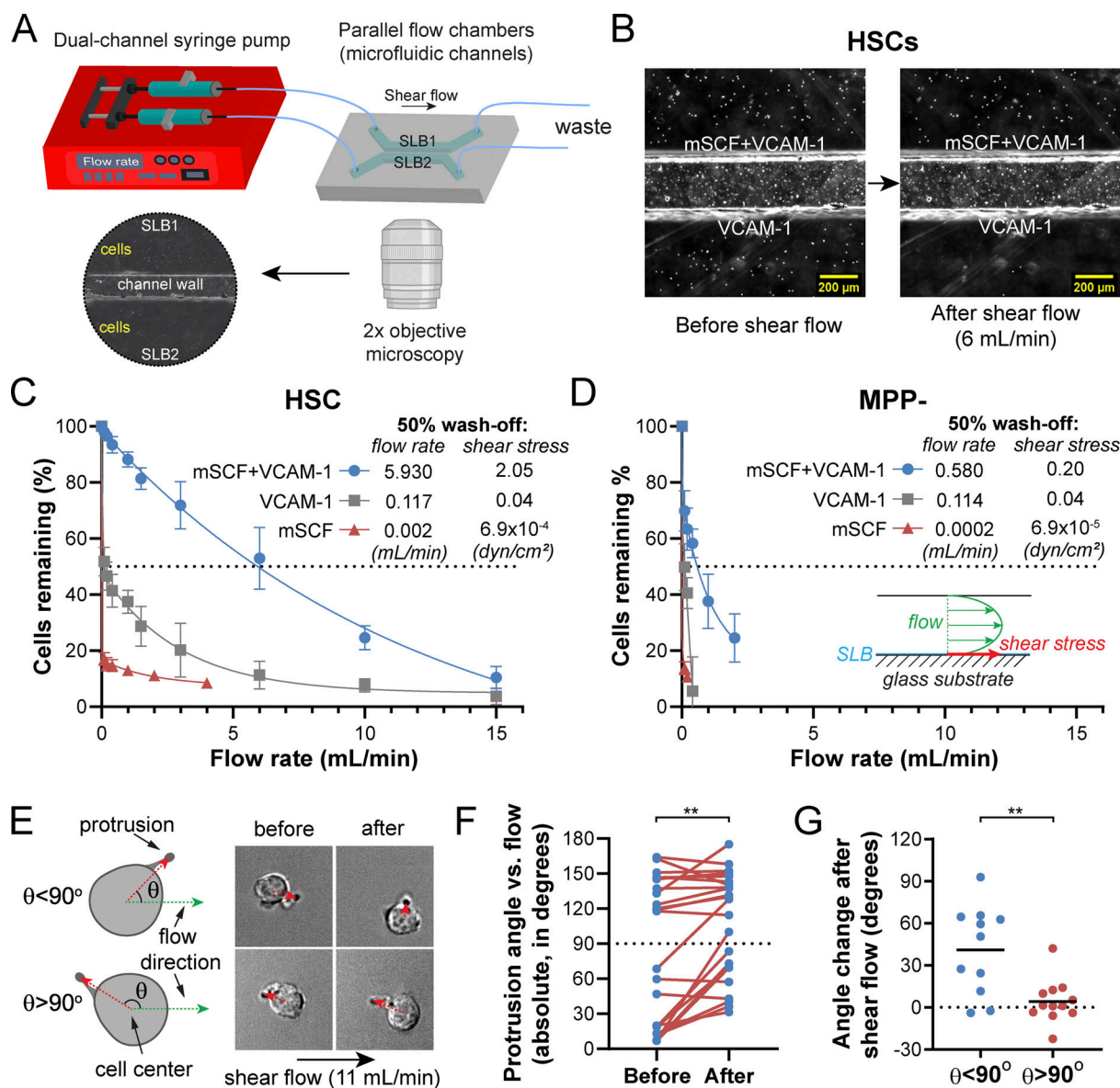
Figure 4. mSCF and VCAM-1 synergistically promote HSC adhesion. (A) Microfluidic setup for assessing the strength of HSC adhesion to SLBs tethered with membrane-bound factors. (B) 2× bright-field images of HSCs seeded on SLBs with mSCF+VCAM-1 and VCAM-1 alone, respectively. Before shear flow (left) and after the shear flow of 6 mL/min (right). (C and D) Percentages of HSCs (C) and MPP- cells (D) remaining on the SLBs after a series of increasing flow rates and the 50% wash-off flow rates and corresponding shear stresses on SLBs. n = 5 ROIs per data point. (E–G) Effect of shear flow on the orientation of the HSC protrusions on the SCF+VCAM-1 SLBs. (E) Definition of the protrusion angle ( \theta ) and orientation changes in HSCs with different starting \theta before and after the shear flow (11 mL/min). (F) Protrusion angles of single HSCs before and after the shear flow. (G) Changes of protrusion angles ( \theta_{\text{after}} - \theta_{\text{before}} ) in HSCs with starting \theta greater or less than 90^\circ . n = 22 single HSCs. Error bars represent SD. **, P < 0.01 by paired Student's t test and unpaired two-tailed Student's t test in F and G, respectively.
