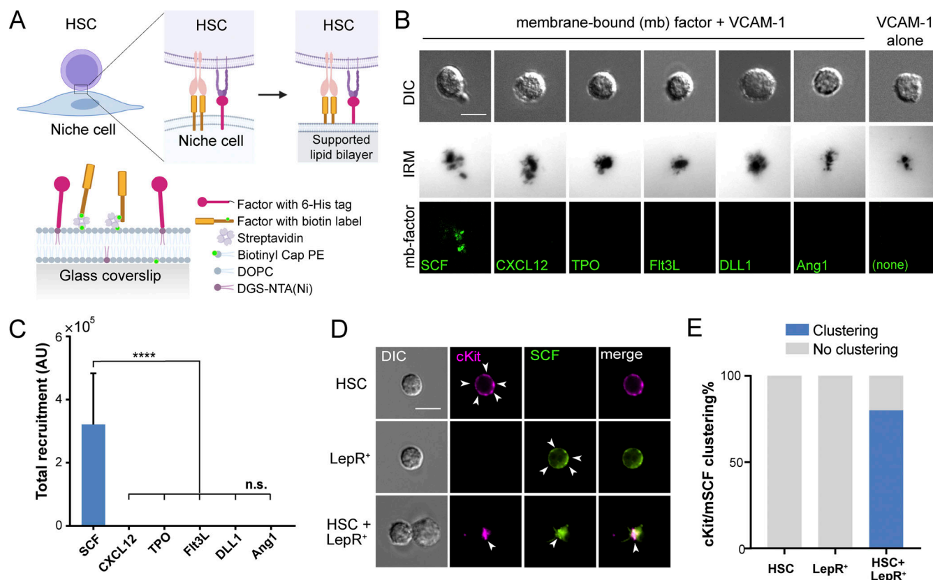
Figure 1. mSCF is the only factor recruited/clustered by HSCs in a screening. (A) Illustration of membrane-bound HSC–niche cell interaction and recapitulation on an SLB. (B) HSCs after incubation with VCAM-1 and a membrane-bound factor (mb-factor; with fluorescent label, background subtracted) on SLBs for 1 h. DIC, differential interference contrast. Dark regions represent cell–substrate contact/adhesion. Scale bar = 5 \mu m. (C) Total membrane-bound factors recruited by single HSCs assessed by the total fluorescence under each cell. n = 37 cells per condition. Error bars represent SD. ****, P < 0.0001 by one-way ANOVA with Tukey's test. AU, arbitrary units. (D) HSCs, LepR + MSCs, and HSC–LepR + MSC pairs forming physical contact after 1-h incubation. Arrowheads point to dispersed cKit or SCF on the surface of single HSCs or LepR + MSCs, respectively, or clustered SCF/cKit at the HSC–MSC interface. Scale bar = 5 \mu m. (E) Frequency of cKit/mSCF clustering on one side of the cell in single cells or in HSC–MSC pairs. n = 20 single cells or cell pairs for each condition.
