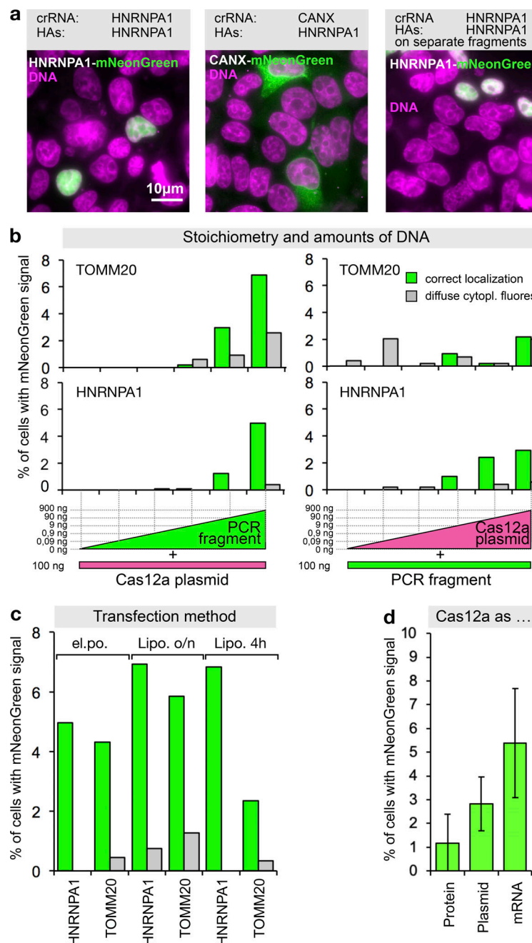
Figure S2. Exploring transfection parameters. (a) Control transfections to demonstrate the effect of the crRNA and the presence of homology arms (HAs). Locus specificity of the homology arms and the crRNA as indicated (related to Fig. 1 e). (b) Impact of transfected amounts of DNA on tagging efficiency using HEK293T cells. Transfected amounts of PCR cassette and Cas12a plasmid as indicated. Always 1 µg of DNA was transfected using lipofectamine. pUC18 was used as neutral DNA. Tagging efficiency was determined 3 d later by HOECHST staining and live-cell imaging. Data from one representative experiment are shown. (c) HEK293T cells were transfected for 4 h or overnight using Lipofectamine 2000 or transfected using electroporation, as indicated. Tagging efficiency was determined 3 d later as described in a. Data from one representative experiment are shown. (d) HEK293T cells were transfected in duplicates by electroporation with Cas12a protein, Cas12a-encoding mRNA, or Cas12-encoding plasmid. For protein-based expression, 100 ng of PCR cassette while for mRNA and plasmid 1.5 µg PCR cassette were electroporated. Error bars indicate range between the technical duplicates.
