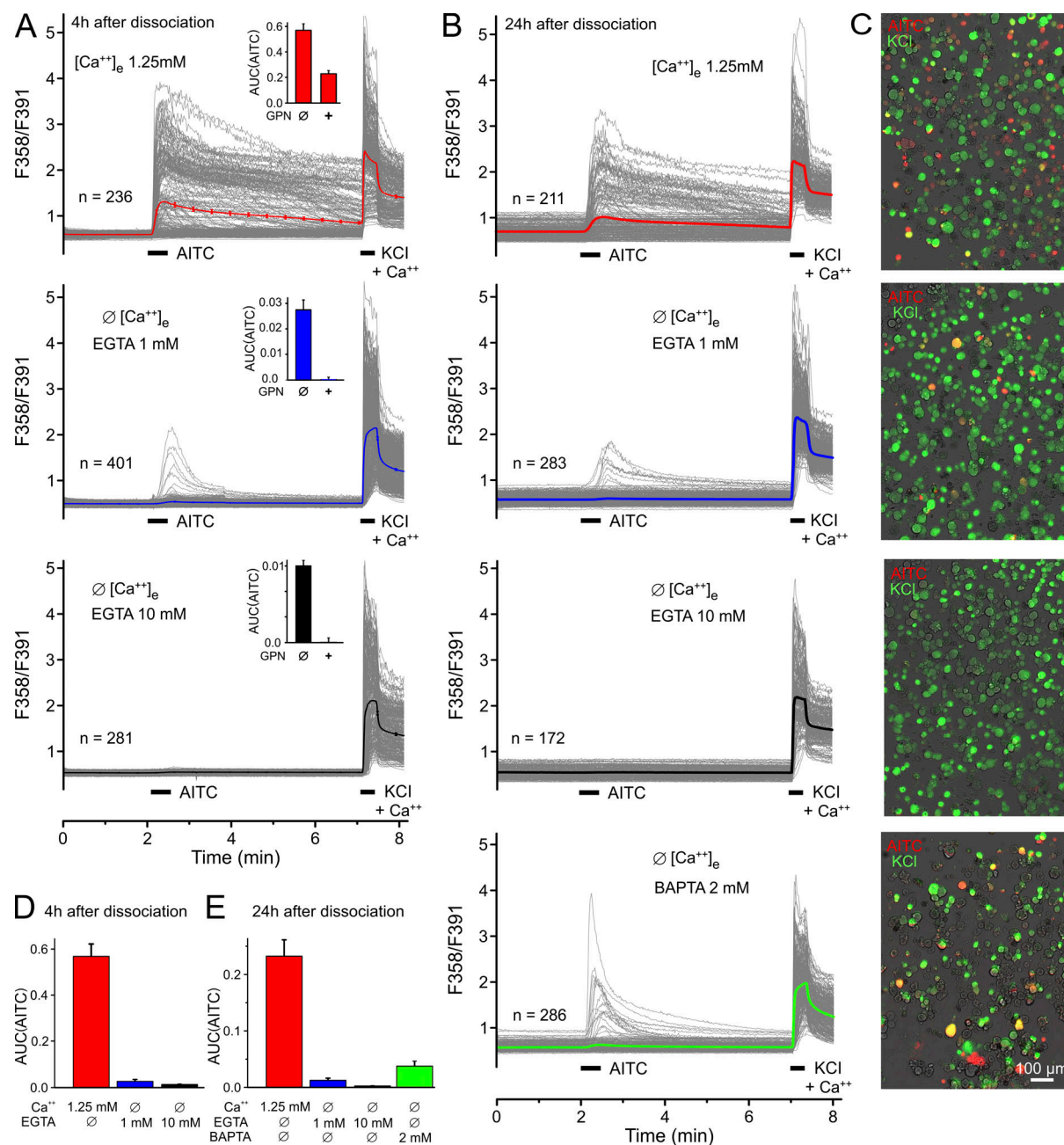
Figure 2. Mouse DRGs do not respond to 100 \mu M AITC in a nominally \text{Ca} -free environment with 10 mM EGTA. 100 \mu M AITC and 60 mM KCl (bars) were applied during calcium imaging; \text{Ca} -free condition was established during 10 min after washout of external Fura-2-AM and terminated just before KCl application. The ratio time courses of single neurons are shown in gray, and the average in bold and color. (A) Neurons were imaged 4–6 h after dissociation and incubation. The inserts show AITC responses after 200 \mu M GPN pretreatment for 40 min (+) in comparison to control ( \emptyset ); note the very different ordinate scales. (B) Neurons were incubated overnight before \text{Ca} imaging. BAPTA as calcium buffer reduced the number of responsive neurons to 8% (vs. 30% in Shang et al. [2016]). (C) Overlays of the transmission image (gray) and the response to AITC (red) and KCl (green) of representative experiments. Neurons responding to both applications appear in yellow. (D) Area under the curve of \text{Ca}^{2+} transients in response to AITC quantified from A. (E) Area under the curve of \text{Ca}^{2+} transients in response to AITC quantified from B, including the BAPTA effect. Data from A and photomicrographs from C also appear in Fig. S2, A and C, to allow for comparison. Error bars represent SEM values of the counted (n) neurons.
