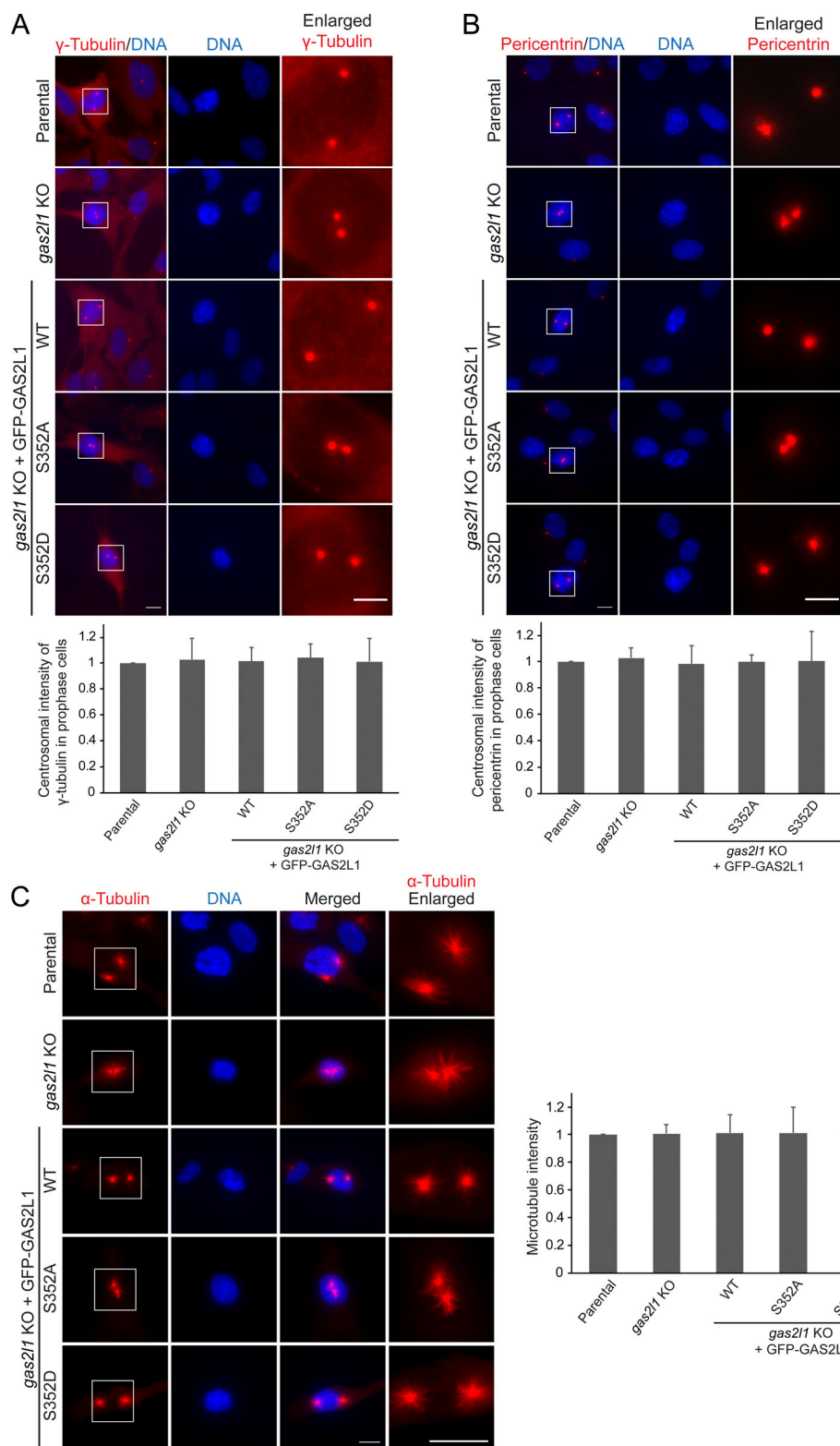
Figure S2. gas2l1 knockout or the disruption of GAS2L1 Ser352 phosphorylation does not affect centrosome maturation. (A and B) RPE-1 parental cells and sublines were stained for (A) \gamma -tubulin or (B) pericentrin. DNA was labeled with Hoechst 33258. Prophase cells were identified based on DNA patterns and analyzed for centrosomal intensities of \gamma -tubulin and pericentrin; data were collected from three independent experiments. Arrowheads: centrosomes. \gamma -Tubulin: n = 52 (Parental), 58 ( gas2l1 KO), 61 ( gas2l1 KO + WT), 55 ( gas2l1 KO + S352A), and 50 ( gas2l1 KO + S352D). Pericentrin: n = 48 (Parental), 51 ( gas2l1 KO), 44 ( gas2l1 KO + WT), 49 ( gas2l1 KO + S352A), and 56 ( gas2l1 KO + S352D). (C) Microtubule regrowth assay was performed on RPE-1 parental cells and sublines. Microtubules were visualized through anti- \alpha -tubulin labeling, and DNA was stained with Hoechst 33258. Centrosome-based microtubule asters were quantified in prophase cells from three independent experiments: n = 50 (Parental), 50 ( gas2l1 KO), 51 ( gas2l1 KO + WT), 55 ( gas2l1 KO + S352A), and 53 ( gas2l1 KO + S352D). Boxed regions are enlarged to show microtubule asters. Scale bars, 10 \mu m.
