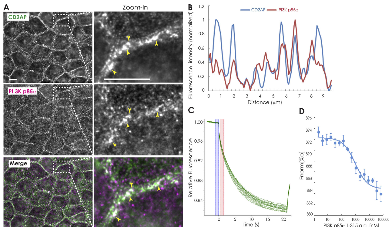
Figure 3. CD2AP colocalizes with and binds to PI3K p85α at the adherens junction. (A) Wide-field immunofluorescence images of mature WT-MDCK cells stained for CD2AP (green) and PI3K p85α (magenta). Zoom-in view of dashed white boxes are shown on the right. CD2AP and PI3K p85α partly colocalize at cell-cell borders (arrowheads). Merged images show regions of colocalization (white spots). Scale bar, 10 μm. (B) Fluorescence intensity profiles along the indicated lines in A support the partial colocalization of CD2AP and PI3K p85α. (C) The association of GFP-CD2AP-1-475 aa with PI3K p85α 1-315 aa was measured by MST. 16 different concentrations (from 2.09 nM to 68.5 μM) of PI3K p85α 1-315 aa were titrated into GFP-CD2AP-1-475 aa (20 nM). Thermophoresis traces shown from one representative experiment are shown. (D) Binding isotherm derived from the raw data and fitted to yield a K_d of 0.94 \pm 0.41 μM. Error bars represent SD; n = 3 .
