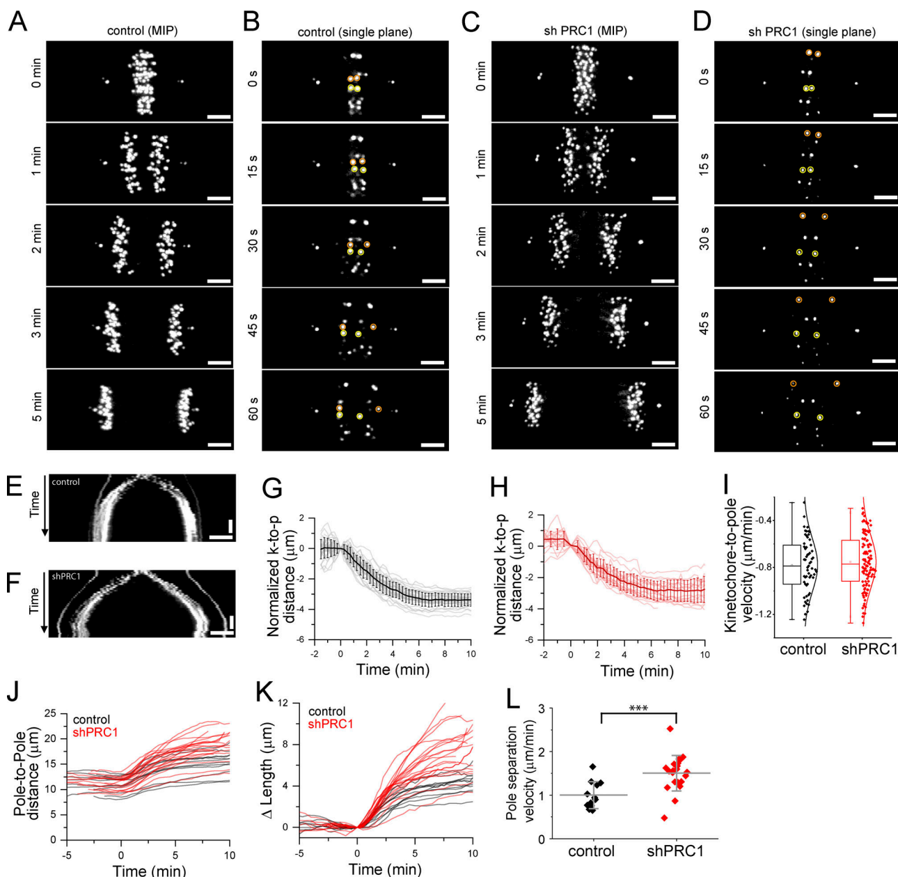
Figure 5. Defects in microtubule bundle assembly increase the rate of anaphase spindle elongation. (A–D) Live-cell imaging of centromere and spindle pole position by spinning disk confocal microscopy. Example hTERT-RPE1 cells expressing GFP-CENP-A to label the kinetochores and GFP-Centrin to label the centrosomes are shown. Select images from time series are shown. A control cell (A and B) and a cell expressing shRNA to PRC1 (shPRC1; C and D) are shown. T = 0 was assigned to the frame immediately prior to that with detectable sister kinetochore separation. (A and C) Maximum-intensity projections (MIPs) show select time points from a cell in anaphase. Time-lapse recordings are provided in Videos 6 and 7. (B and D) Single image planes show consecutive images (15-s intervals) from the cells shown in A (B) or C (D). Selected kinetochore pairs are highlighted (orange and yellow circles). (E and F) Kymograph generated from the time-lapse videos of the cell shown in A (E) or C (F). Horizontal scale bar, 3 \mu\text{m} . Vertical scale bar, 2 min. (G and H) Analysis of normalized kinetochore-to-pole (k-to-p) distance show individual kinetochores (thin lines) and average (bold line) traces from an example control cell (G) and an example shPRC1 cell (H). Error bars are SD. (I) Box-and-whisker plots of kinetochore-to-pole velocity. Each point represents the velocity of a single kinetochore. Velocity was determined by linear fit to kinetochore-to-pole distance versus time in the T = 0.5–3-min time window. Negative sign indicates direction of slope. Data were pooled data from all experiments ( n = 59 and 111 kinetochores for control and shPRC1 cells, respectively) and fit to a Gaussian. (J) Plots of pole-to-pole distance versus time for control ( n = 12 cells; black traces) and shPRC1 ( n = 21 cells; red traces) cells. (K) Plot of relative pole separation distance ( \Delta\text{Length} ), defined as the pole-to-pole distance at time t ( L_t ) minus the pole-to-pole distance at T = 0 ( L_0 ). (L) Pole separation velocity for control and shPRC1 cells (***, P < 0.003 ). Mean \pm SD.
