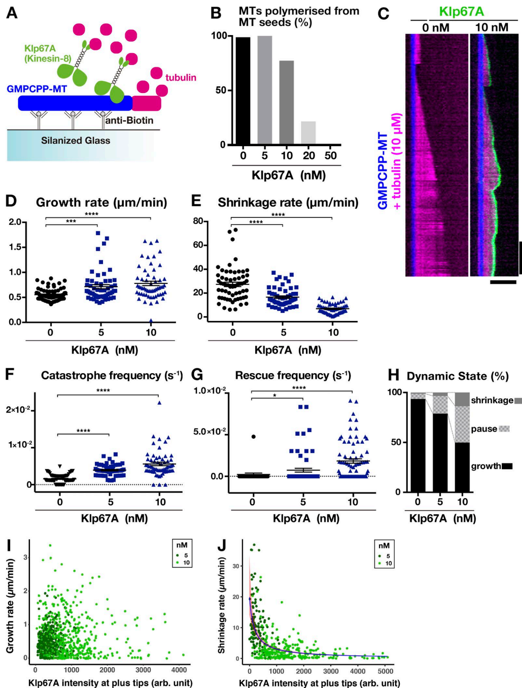
Figure 3. Kinesin-8 Klp67A regulates MT plus end dynamics in vitro. (A) Schematic presentation of the in vitro MT polymerization assay. (B) Inhibitory effect of kinesin-8 Klp67A on MT polymerization from the seed ( n = 84, 74, 84, 74 , and 94 ; from left to right). (C) MT dynamics are represented by kymographs. MTs stabilized with GMPCPP are colored blue, dynamic MTs are magenta, and kinesin-8 Klp67A -GFP (0 or 10 nM) is green. Horizontal bar, 5 \mu\text{m} ; vertical bar, 120 s. (D–H) Parameters of MT plus end dynamics. Experiments were performed twice, and the combined data are displayed (the change in rate/frequency by kinesin-8 Klp67A was reproduced). n = 41 + 33 (0 nM), 25 + 31 (5 nM), and 20 + 41 (10 nM). Each dot represents a value obtained from a single MT, and error bars represent SEM. Note that rescue was rarely observed in the absence of kinesin-8 Klp67A . *, P < 0.03 ; ***, P < 0.002 ; ****, P < 0.0001 or by Games-Howell (D–F) or Steel Dwass (G) tests. (I and J) Correlation between the amount of kinesin-8 Klp67A -GFP at the tip and growth (I; n = 397 [5 nM] and 494 [10 nM]) or shrinkage (J; n = 116 [5 nM] and 293 [10 nM]) rate. Negative correlation was found for shrinkage rate ( P < 2 \times 10^{-16} , likelihood ratio test).
