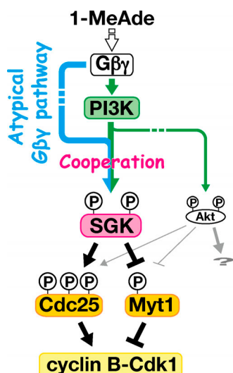
Figure 7. SGK triggers cyclin B-Cdk1 activation in 1-MeAde signaling. Downstream of 1-MeAde stimulation, Gβγ activates the PI3K pathway (green arrow) and the atypical Gβγ pathway (cyan arrow). SGK is activated by co-operation of these pathways and subsequently activates and inactivates Cdc25 and Myt1, respectively, via direct phosphorylation. Consequently, reversal of the balance of Cdc25 and Myt1 activities triggers cyclin B-Cdk1 activation. Akt is weakly activated after 1-MeAde stimulation and may phosphorylate Cdc25 and Myt1 at undetectable levels. However, Akt is dispensable for cyclin B-Cdk1 activation and may have other functions in oocytes.
