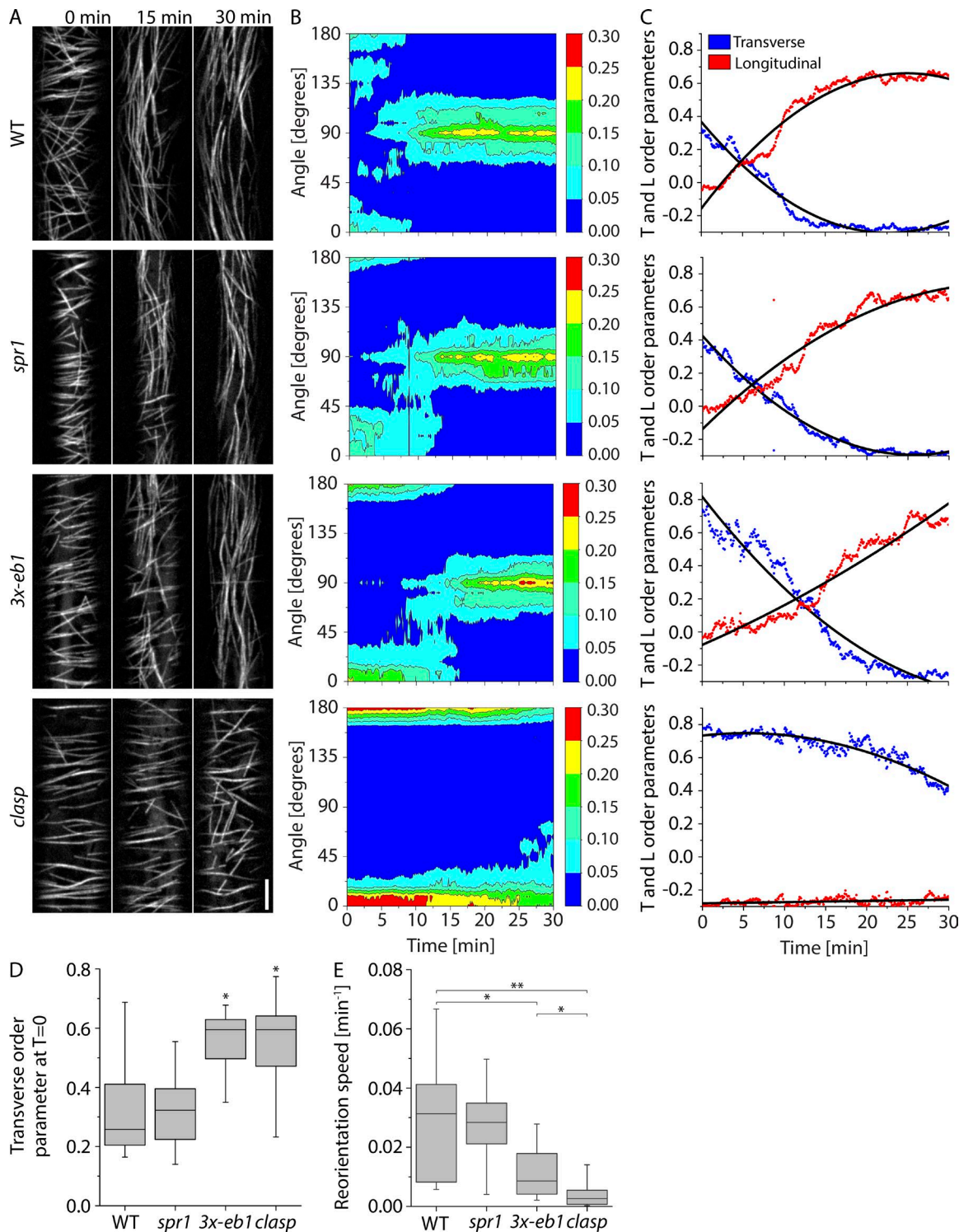
Figure 1. Microtubule reorientation in +TIP mutants. (A) Panels from confocal image time series of dark-grown hypocotyl cells expressing YFP-TUA5 in WT, spr1 , 3x-eb1 , and clasp mutant backgrounds at 0, 15, and 30 min after induction of reorientation by blue light. See Video 1. Scale bar is 5 \mu\text{m} . (B) Representative contour plots of MT orientation over time corresponding to the videos shown in A. The color scale represents fraction of microtubules. (C) Longitudinal and transverse order parameters during MT reorientation for the videos shown in A. Black lines show quadratic fit. (D) Transverse order parameter at T = 0 for cortical microtubules imaged in WT, spr1 , 3x-eb1 , and clasp seedlings. n = 8, 9, 9 , and 9 cells, respectively. A Kruskal–Wallis test showed significant differences among the genotypes ( P < 0.01 ). Asterisks represent significant difference from WT by Mann–Whitney U test ( P < 0.05 ). (E) Longitudinal reorientation speed (Lindeboom et al., 2013b) of imaged microtubule arrays in etiolated hypocotyl cells expressing YFP-TUA5 in WT, spr1 , 3x-eb1 , and clasp seedlings. A Kruskal–Wallis test showed significant differences for reorientation speed distributions among the genotypes ( P < 0.01 ). n = 8, 9, 9 , and 9 cells, respectively. Asterisks represent significant difference from WT in Mann–Whitney U test (*, P < 0.05 ; **, P < 0.01 ; ***, P < 0.001 ). Boxplots show the 25th and 75th percentile as box edges, the line in the box indicates median value, and the whiskers show the 2.5th and 97.5th percentile.
