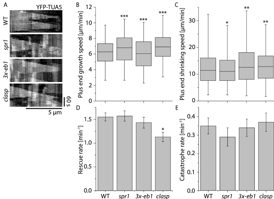
Figure 2. Microtubule plus end dynamics in +TIP mutants. (A) Kymographs of microtubules during early stages of cortical array reorientation induced by blue light in WT , spr1 , 3x-eb1 , and clasp seedlings expressing YFP-TUA5. (B and C) Boxplot of microtubule plus end growth speeds (B) and plus end shrinkage speeds (C) in n = 2,148, 1,405, 1,837 , and 1,516 segments measured in WT , spr1 , 3x-eb1 , and clasp seedlings, respectively. Boxplots show the 25th and 75th percentile as box edges, the line in the box indicates median value, and the whiskers show the 2.5th and 97.5th percentile. Asterisks indicate a significant difference from WT. (D) Microtubule rescue rates. n = 213, 135, 110 , and 116 rescues in WT , spr1 , 3x-eb1 , and clasp mutant backgrounds, respectively. Error bars represent SEM. Asterisks indicate a significant difference by rate ratio test. (E) Microtubule catastrophe rates. n = 190, 119, 155 , and 148 rescues in WT , spr1 , 3x-eb1 , and clasp mutant backgrounds, respectively. Error bars represent SEM. Asterisks indicate significant difference compared with WT by rate ratio test. *, P < 0.05 ; **, P < 0.01 ; ***, P < 0.001 . Data for all measurements are from six cells in six plants for each genotype.
