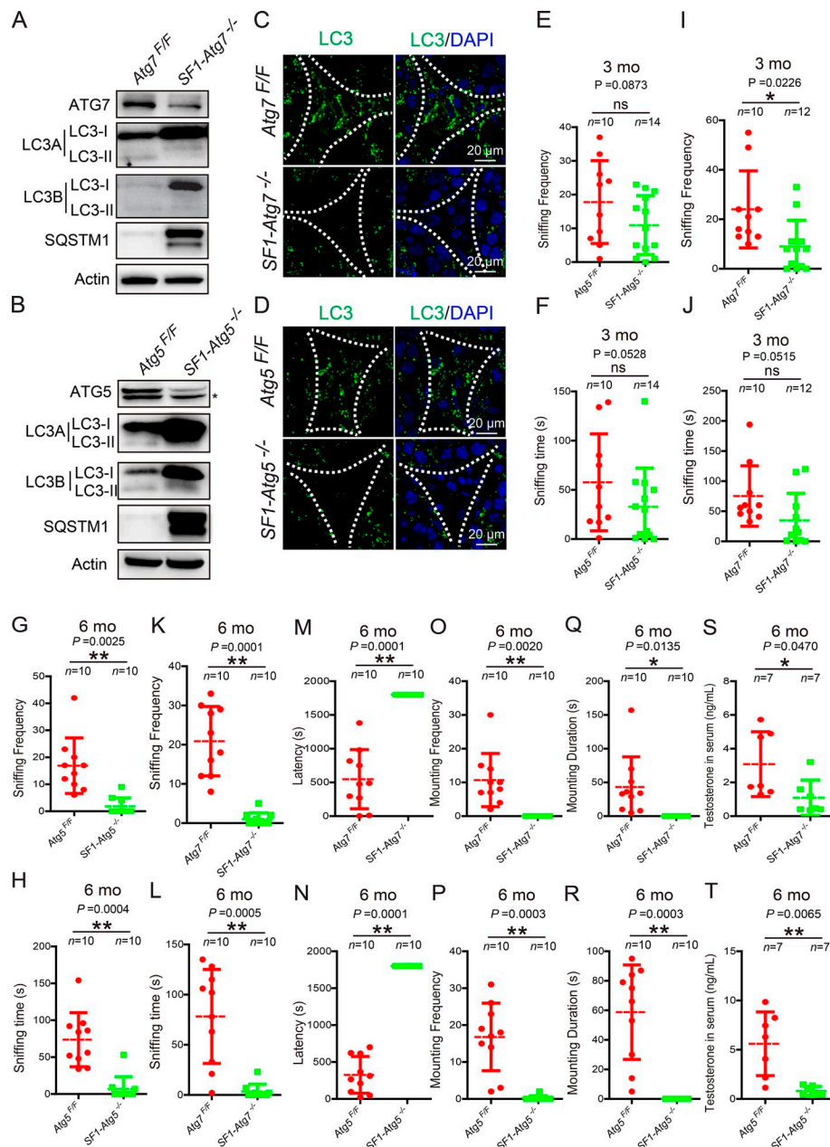
Figure 2. Steroidogenic cell-specific knock-out of Atg7 - or Atg5 -affected testosterone synthesis. (A and B) The autophagic flux was disrupted in autophagy-deficient Leydig cells. Immunoblotting analyses of ATG7, SQSTM1/p62, and LC3 were performed in both Atg7 Flox/Flox (left) and SF1-Atg7 -/- Leydig cells (right; A). The ATG7 protein level was dramatically reduced, and actin served as a loading control. Similar results were observed in Atg5 Flox/Flox mice (left) and SF1-Atg5 -/- mice (right) as shown in B. The asterisk indicates nonspecific signals. (C and D) The LC3 punctate structures disappeared in Leydig cells of autophagy-deficient mice. Immunofluorescence analysis using LC3 (green) in both Atg7 Flox/Flox (top) and SF1-Atg7 -/- Leydig cells (bottom; C). Similar results were obtained in Atg5 Flox/Flox mice (top) and SF1-Atg5 -/- mice (bottom) as shown in D. Nuclei were stained with DAPI (blue). (E–L) Aging autophagy-deficient male mice spent less time sniffing female targets than the control male mice. 3-mo-old Atg5 -deficient mice showed no significant difference in sniffing frequency and time (E and F), whereas 6-mo-old autophagy-deficient mice spent less time sniffing female genital odor than the control groups (G, H, K, and L). (M and R) Aging autophagy-deficient male mice showed a failure of mounting. 6-mo-old autophagy-deficient male mice mounted female mice with a longer latency (M and N), less frequency (O and P), and shorter duration (Q and R) than the control groups. (S and T) Testosterone production was significantly reduced in autophagy-deficient mice. *, P < 0.05 ; **, P < 0.01 .
