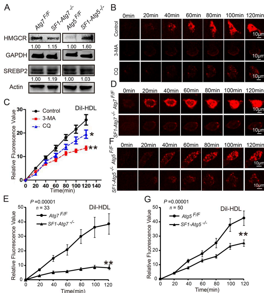
Figure 4. Impaired autophagy perturbs cholesterol uptake. (A) The levels of cholesterol synthesis-related proteins did not decrease in autophagy-deficient Leydig cells. Immunoblotting analysis of HMGR and SREBP2 in Atg7 Flox/Flox , SF1-Atg7 -/- , Atg5 Flox/Flox , and SF1-Atg5 -/- Leydig cells. GAPDH and actin served as loading controls. (B) The isolated Leydig cells were treated with physiological saline (control), 3-MA, or CQ. The in vitro cholesterol absorption experiment was subsequently performed in Leydig cells using the fluorescence-labeled cholesterol-rich lipoprotein Dil-HDL and were examined using live-cell imaging. (C) The absorption curves of Dil-HDL in 3-MA- or CQ-treated Leydig cells and control groups. (D and F) The steroidogenic cell-specific knockout Atg7 or Atg5 affected cholesterol uptake. Absorption of Dil-HDL (red) was examined using live-cell imaging. (E and G) The absorption curve of Dil-HDL in autophagy-deficient Leydig cells and control groups. Error bars show means \pm SD. *, P < 0.05; **, P < 0.01.
