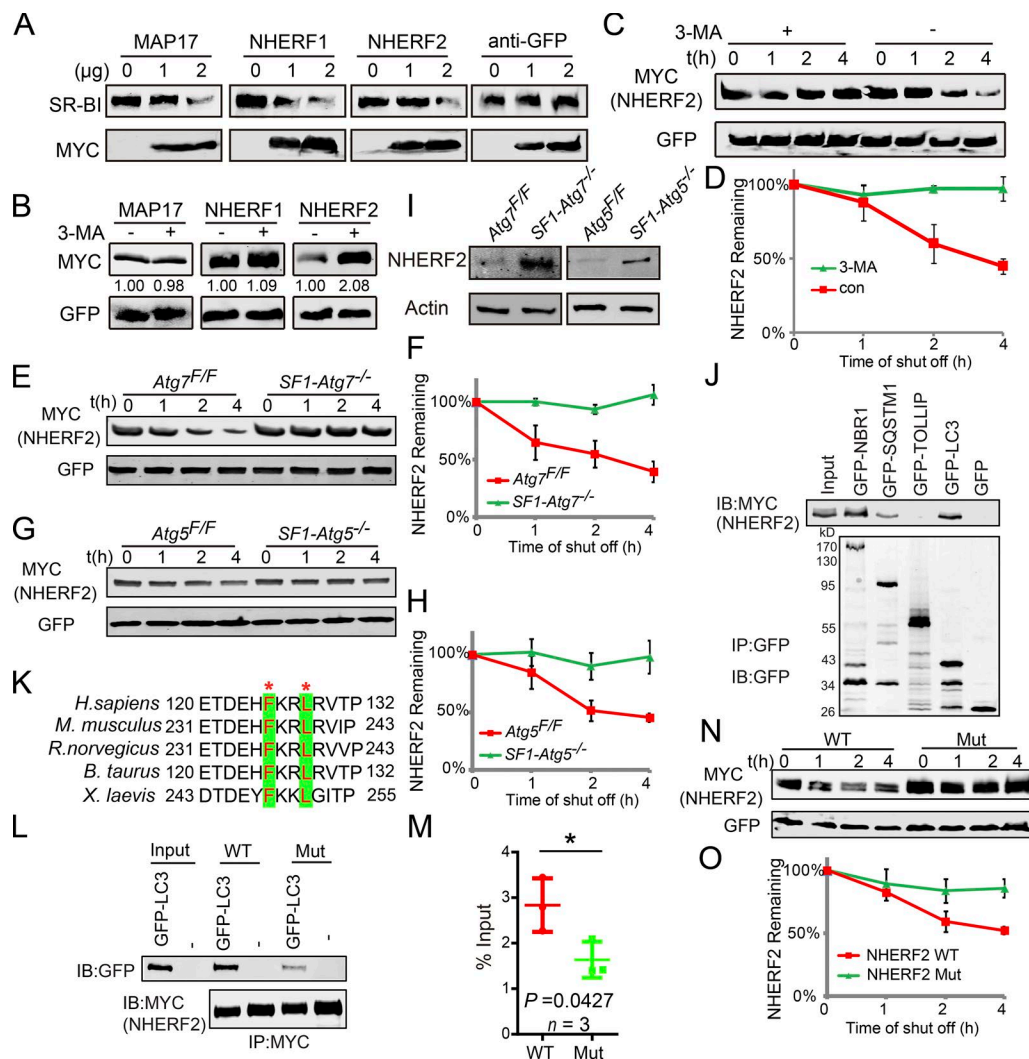
Figure 6. Selective autophagy-dependent degradation of NHERF2. (A) The overexpression of NHERF1, NHERF2, and MAP17 down-regulated the protein levels of SR-BI. (B) Treatment with 3-MA resulted in the accumulation of NHERF2 but not the other two SR-BI negative regulators. (C) NHERF2 was stabilized in autophagic flux-disrupted cells. CHX chase assay of NHERF2 in HEK293T cells in the absence or presence of 3-MA. (D) Quantification of the relative NHERF2 levels in C. (E and G) NHERF2 was stabilized in autophagy-deficient Leydig cells. CHX chase assay of NHERF2 in Atg7 Flox/Flox and SF1-Atg7 -/- (E) as well as Atg5 Flox/Flox and SF1-Atg5 -/- (G) Leydig cells. (F and H) Quantification of the relative NHERF2 levels in E and G. (I) NHERF2 is accumulated in autophagy-deficient Leydig cells. The immunoblotting (IB) analysis of NHERF2 was performed in Atg7 Flox/Flox and SF1-Atg7 -/- as well as Atg5 Flox/Flox and SF1-Atg5 -/- Leydig cells. Actin served as a loading control. (J) NHERF2 interacts with LC3, NBR1, and SQSTM1. pCMV6-Myc-Nherf2 and pMXs-puro-GFP-SQSTM1, pMXs-IP-GFP-NBR1(38283), pEGFP-TOLLIP, or pEGFP-LC3 were cotransfected into HEK293T cells. 24 h after transfection, cells were collected for IP with anti-GFP antibody and analyzed with GFP antibodies, respectively. (K) Sequence alignment of NHERF2 LIR motifs from different species. Asterisks indicate conserved residues in LIR motifs. (L) The disruption of the LIR motif in NHERF2 influences its interaction with LC3. (M) Quantification of the relative binding affinity between NHERF2 (WT/mutant [F236A/L239A]) and GFP-LC3. Relative amounts of GFP-LC3 were quantified using Odyssey software and compared with the input. (N) The LIR motif of NHERF2 is essential for its degradation. CHX chase assay of NHERF2 (WT) and NHERF2 F236A/L239A (Mut) in HEK293T cells. (O) Quantification of the relative NHERF2 levels in N. The amounts of NHERF2 were quantified using Odyssey software. See also Figs. S4 and S5. Error bars show means \pm SD. *, P < 0.05 .
