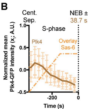
Figure 9. An analysis of Plk4 centriolar dynamics. (A) Micrographs show spinning-disk confocal fluorescence images taken from a time-lapse movie of an early embryo expressing Jupiter-mCherry (as a microtubule marker) and Plk4-GFP; time in minutes:seconds is indicated. At time t = 0:00 , the embryo is in early S-phase, and the centrosomes have recently separated. Inset shows a single centriole pair (bar, 1 \mu\text{m} ), which is then shown at 30-s or 1-min intervals (bar, 0.5 \mu\text{m} ). The cell-cycle stage is indicated above each time interval. A series of lower-magnification views of the embryos are shown below the images of the individual centrioles to illustrate how MTs were used to determine the cell-cycle stage at each time point. Bar, 10 \mu\text{m} . (B) Graph shows the mean Plk4-GFP incorporation profile during S-phase of nuclear cycle 12 in WT embryos ( n = 6 embryos). The mean incorporation profile of Sas-6-GFP is shown overlaid (dotted orange, same data shown in Fig. 3 A, but normalized for the length of S-phase). (C and D) Charts quantify parameters of Plk4-GFP behavior derived from mean Plk4-GFP profiles from embryos at nuclear cycles 11, 12, and 13 ( n \geq 5 embryos for each cycle; n = 34, 31 , and 33 centriole pairs [mean] per embryo, respectively). A.U., arbitrary units. Data are represented as mean \pm SD. Statistical significance was assessed using either an ordinary one-way ANOVA test (for Gaussian-distributed data) or a Kruskal–Wallis test, and is shown above each chart.
