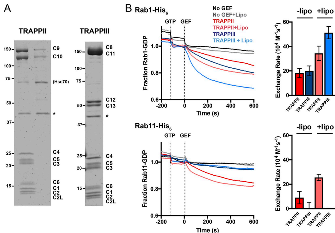
Figure 5. TRAPPII complex activates the Rab GTPases Rab1 and Rab11, whereas TRAPPIII only shows GEF activity toward Rab1. (A) Coomassie blue-stained protein gels of recombinant Drosophila TRAPP complexes purified from Sf9 cells coexpressing the subunits of each complex. FLAG tags on C10 or C11 allowed isolation of TRAPPII or TRAPPIII, respectively. PreScission protease (GST-HRV-3C protease) was used to cleave the tags (asterisks) and was subsequently removed using glutathione Sepharose beads. C10 also copurified with C9 in the absence of the shared subunits (TRAPPII lane). The Hsc70 chaperone (CG4264) is a contaminant of the TRAPPII purification protocol. Molecular masses are given in kilodaltons. (B) Release of mant-GDP from 250 nM of Rab-His 6 by 50 nM of TRAPPII or TRAPPIII in the presence or absence of synthetic fly Golgi mix liposomes. Traces are the mean of at least three experiments. Error bars show SEM.
