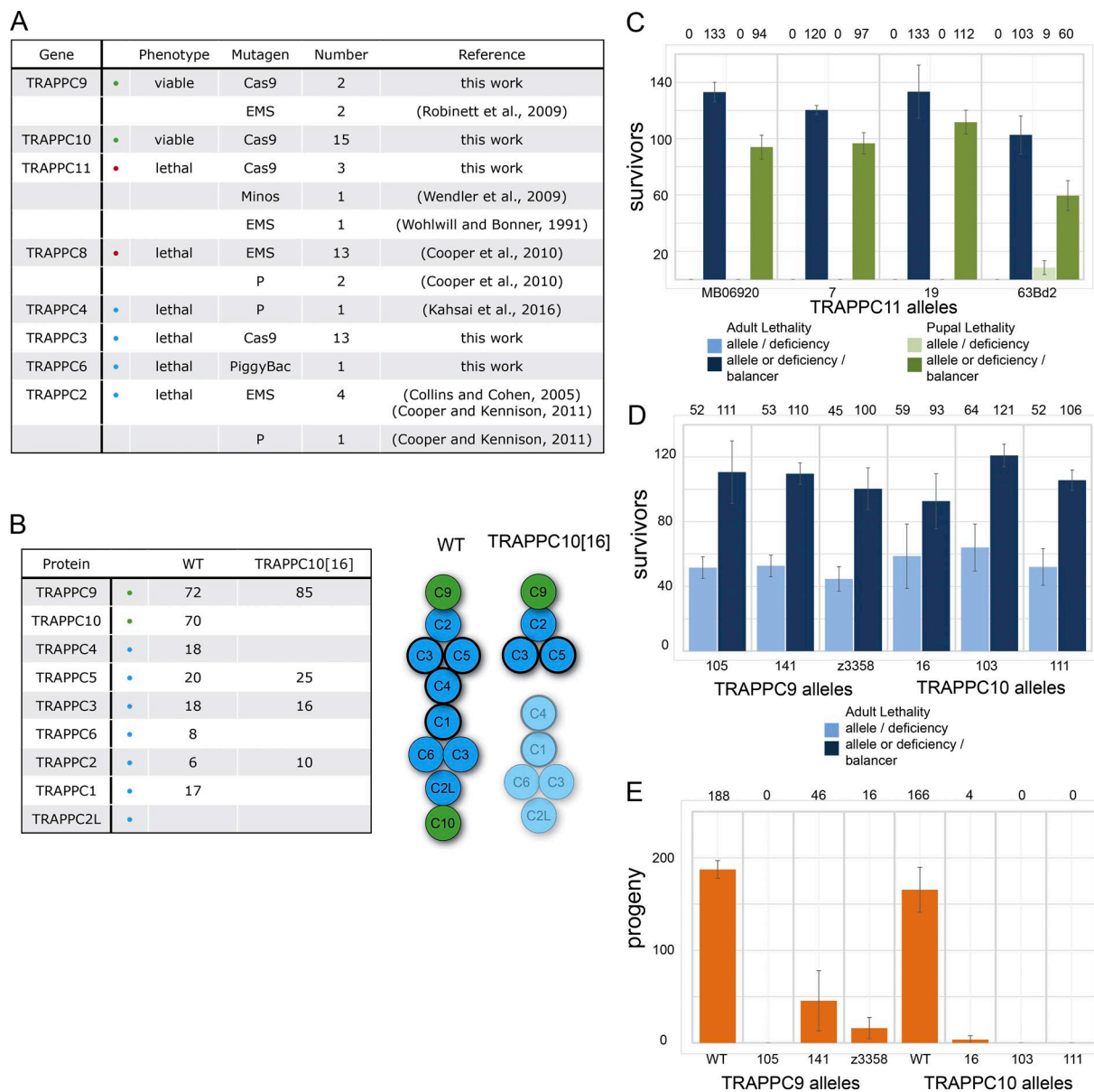
Figure 4. TRAPPII is required for male fertility, and TRAPPIII is essential for viability. (A) Summary of mutations generated in TRAPP subunits in this and previous studies. The nature of the lesions in the EMS alleles of TRAPPC2, TRAPPC8, and TRAPPC11 were determined by sequencing the locus from the relevant mutants (Fig. S2 B). (B) Mass spectrometry analysis of TRAPPC9–SBP–GFP tandem affinity–purified from a WT or TRAPPC10[16] mutant background. Total spectral counts for each protein are shown. Subunits with a thick line in the cartoon are essential for Rab1 nucleotide exchange activity in yeast. (C) TRAPPC11 is essential for adult (blue bars) and pupal (green bars) viability. The bars show mean numbers of adult or pupal progenies calculated from two parallel crosses (pupal lethality of TRAPPC11[MB06920]/deficiency heterozygotes and TRAPPC11[63BD2]/deficiency heterozygotes) or three parallel crosses (all other heterozygotes). The mean value is shown above each bar. Note that TRAPPC11[63BD2]/deficiency heterozygotes occasionally develop into pupae, suggesting the allele is a strong hypomorph. (D) TRAPPC9 and TRAPPC10 are not essential for adult viability. The bars show the mean number of adult progeny obtained in three independent crosses. (E) TRAPPC9 and TRAPPC10 are required for male fertility. The bars show the mean number of pupal progeny from three independent crosses using males with the indicated allele over the relevant deficiency. Error bars show SD.
