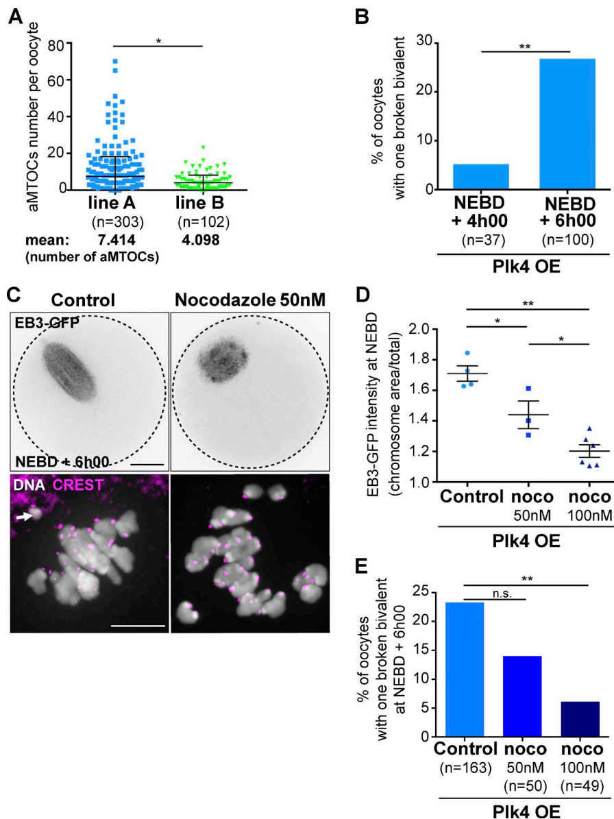
Figure 6. Extent of bivalent breakage correlates with aMTOC spreading and MT density. (A) Quantitative analysis of aMTOC number per oocyte in the two Plk4 OE lines (line A, blue squares; line B, green triangles) in prophase I; *, P = 0.0365 (two-tailed Mann-Whitney test). The mean number of aMTOCs per prophase I oocyte is indicated below the graph for each line. (B) Extent of bivalent breakage increases significantly as meiosis I progresses in oocytes from line A. Percentage of Plk4 OE oocytes from line A with one broken bivalent as a function of the stage of meiosis I (NEBD + 4h00 and NEBD + 6h00); **, P = 0.0047 . (C) Effect of 50 nM nocodazole treatment observed at NEBD + 6h00 in living Plk4 OE oocytes from line A, expressing EB3-GFP (upper panels) and in fixed samples (lower panels) labeled for DNA (white) and CREST (pink). The black dotted circles in the upper panels highlight the oocyte contour. Scale bar is 20 \mu\text{m} . (D) Quantification of the relative MT density measured at NEBD around chromosomes in Plk4 OE from line A oocytes injected with EB3-GFP in control conditions or after treatment with 50 or 100 nM nocodazole (noco). The EB3-GFP signal was measured in a \varnothing 20\text{-}\mu\text{m} region around the chromosomes; total signal intensity was measured in a \varnothing 70\text{-}\mu\text{m} region covering the whole oocyte. Normalized signal intensity is the ratio of local/total intensity measured for individual oocytes. Tukey's multiple comparison test gives *, P < 0.05 for controls vs. noco 50 nM; **, P < 0.01 for controls vs. noco 100 nM; and *, P < 0.05 for noco 50 nM vs. noco 100 nM. (E) Decreasing MT density with nocodazole reduces the extent of DNA breakage. Percentage of Plk4 OE oocytes from line A presenting one broken bivalent at NEBD + 6h00 as a function of nocodazole concentration (0, 50, and 100 nM, respectively, darker blue histograms). P = 0.1725 for 0 vs. 50 nM, and **, P = 0.0068 for 0 vs. 100 nM. For B and E, the statistical tests used are Fisher's exact tests. For A, B, and E, n is the number of oocytes. Error bars correspond to SD.
