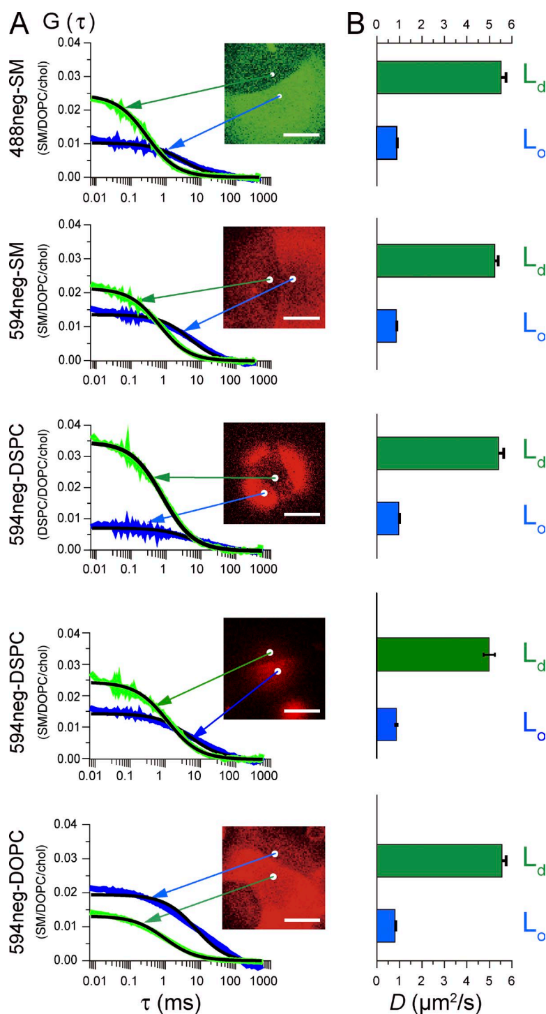
Figure 4. Diffusion coefficients of 488neg-SM, 594neg-SM, 594neg-DSPC, and 594neg-DOPC in L_o and L_d domains in L_o - L_d phase-separated GUVs, determined by FCS. (A) Autocorrelation functions G(\tau) values for the time-dependent changes of the signal intensities of the fluorescent probes observed at typical diffraction-limited areas (white spots) shown in the image on the right in L_o and L_d domains (the spots in the images are expanded 5 \times to show their locations clearly). The black solid smooth curves indicate the best-fit functions, providing the diffusion coefficients ( D ). Bars, 10 \mu\text{m} . 594neg-DSPC was examined in both L_o - L_d phase-separated GUVs consisting of SM(18:0)/DOPC/cholesterol and those made of DSPC/DOPC/cholesterol (1:1:1 by moles). (B) Mean \pm SE values of D in the L_d and L_o domains ( n = 24, 24, 31, 27, 24, 31, 25, 24, 25 , and 25 GUVs from top to bottom). See also Figs. 2 and 3.
