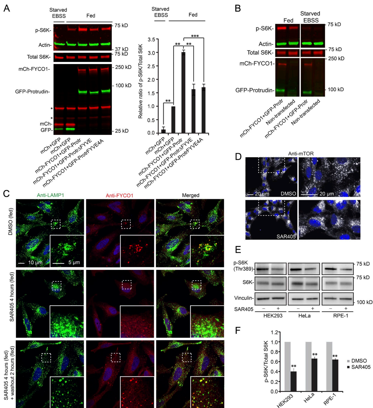
Figure 2. Protrudin and FYCO1 increase S6K phosphorylation in a PtdIns3P-dependent manner. (A) HeLa cells were transfected (40 h) with GFP-Protrudin WT, ΔFYVE, or FYVE4A in combination with mCherry-FYCO1 and analyzed by immunoblotting using antibodies specific to the proteins indicated. GFP and mCherry were used as controls. Where indicated, the cells were starved for 2 h with EBSS. Asterisks indicate unspecific bands from anti-mCherry. Graph shows quantification of immunoblots, representing the relative intensity of phospho-S6K normalized to the total amount of S6K in each sample. Error bars denote \pm SEM from independent experiments ( n = 3 ). **, P < 0.01 ; ***, P < 0.001 (Protrudin WT vs. mutants; unpaired t test; fed control set to 1 vs. starved control or fed Protrudin WT; one-sample t test). (B) HeLa cells were cotransfected (40 h) with GFP-Protrudin WT and mCherry-FYCO1 and analyzed by immunoblotting using antibodies specific to the proteins indicated. Nontransfected cells were used as controls. Where indicated, the cells were starved for 2 h with EBSS. The immunoblot is representative of three independent experiments. (C) HeLa cells were treated with 0.1% DMSO or 3 \mu M SAR405 for 4 h, before washout of SAR405 for 2 h (all treatments in complete medium), stained with antibodies against LAMP1 and FYCO1, and analyzed by confocal microscopy. (D) RPE-1 cells were treated with 0.1% DMSO or 3 \mu M SAR405 for 4 h (all treatments in complete medium), stained with an antibody against mTOR, and analyzed by wide-field microscopy. (E) HeLa, HEK293, and RPE-1 cells were treated with 0.1% DMSO or 3 \mu M SAR405 in complete medium for 4 h and analyzed by immunoblotting. (F) Quantification of immunoblots (as in E), representing the relative intensities of phospho-S6K normalized to the total amount of S6K in each sample. Error bars denote \pm SEM from independent experiments ( n = 3 ). **, P < 0.01 (one-sample t test).
