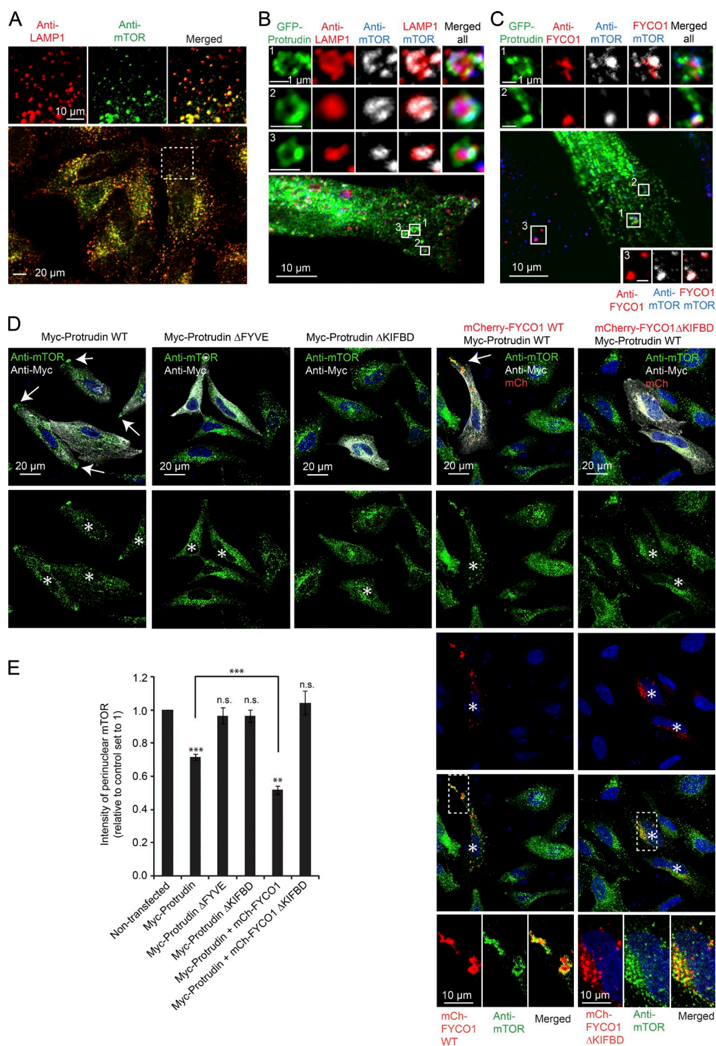
Figure 1. Protudrin and FYCO1 mediate translocation of mTOR lysosomes to the cell periphery. (A) Confocal micrograph showing colocalization between endogenous LAMP1 and mTOR in HeLa cells grown in complete medium. (B and C) HeLa cells were transfected with GFP Protudrin for 20 h, stained with antibodies against LAMP1 and mTOR (B) or FYCO1 and mTOR (C), and analyzed by confocal microscopy. Insets show magnification of lysosomes in contact with Protudrin-positive ER. (D) HeLa cells were transfected (40 h) with the constructs indicated, labeled for endogenous mTOR, and analyzed by confocal microscopy. Asterisks indicate transfected cells. Arrows point at mTOR in the cell periphery. Insets show magnification of mTOR- and mCherry-FYCO1-positive lysosomes. Note that whereas mCherry-FYCO1WT colocalizes with mTOR in the cell periphery, mCherry-FYCO1 \Delta KIFBD colocalizes with mTOR in the perinuclear area. (E) Automated quantification of cells treated as in D, using the Olympus ScanR system. Graphs represent the relative total intensities of perinuclear localization of mTOR-positive lysosomes. The transiently transfected cells were compared directly with nontransfected neighboring cells (set to 1) in each sample. Error bars denote \pm SEM from independent experiments: GFP-ProtudrinWT ( n = 5 ), GFP-Protudrin \Delta FYVE and \Delta KIFBD ( n = 4 ), and GFP-ProtudrinWT+mCh-FYCO1WT or \Delta KIFBD ( n = 3 ). **, P < 0.01 ; ***, P < 0.001 . Myc-ProtudrinWT and Myc-ProtudrinWT+mCh-FYCO1WT, unpaired t test. Transfected cells versus control set to 1, one-sample t test. In total 200–800 transfected cells were analyzed per condition.
