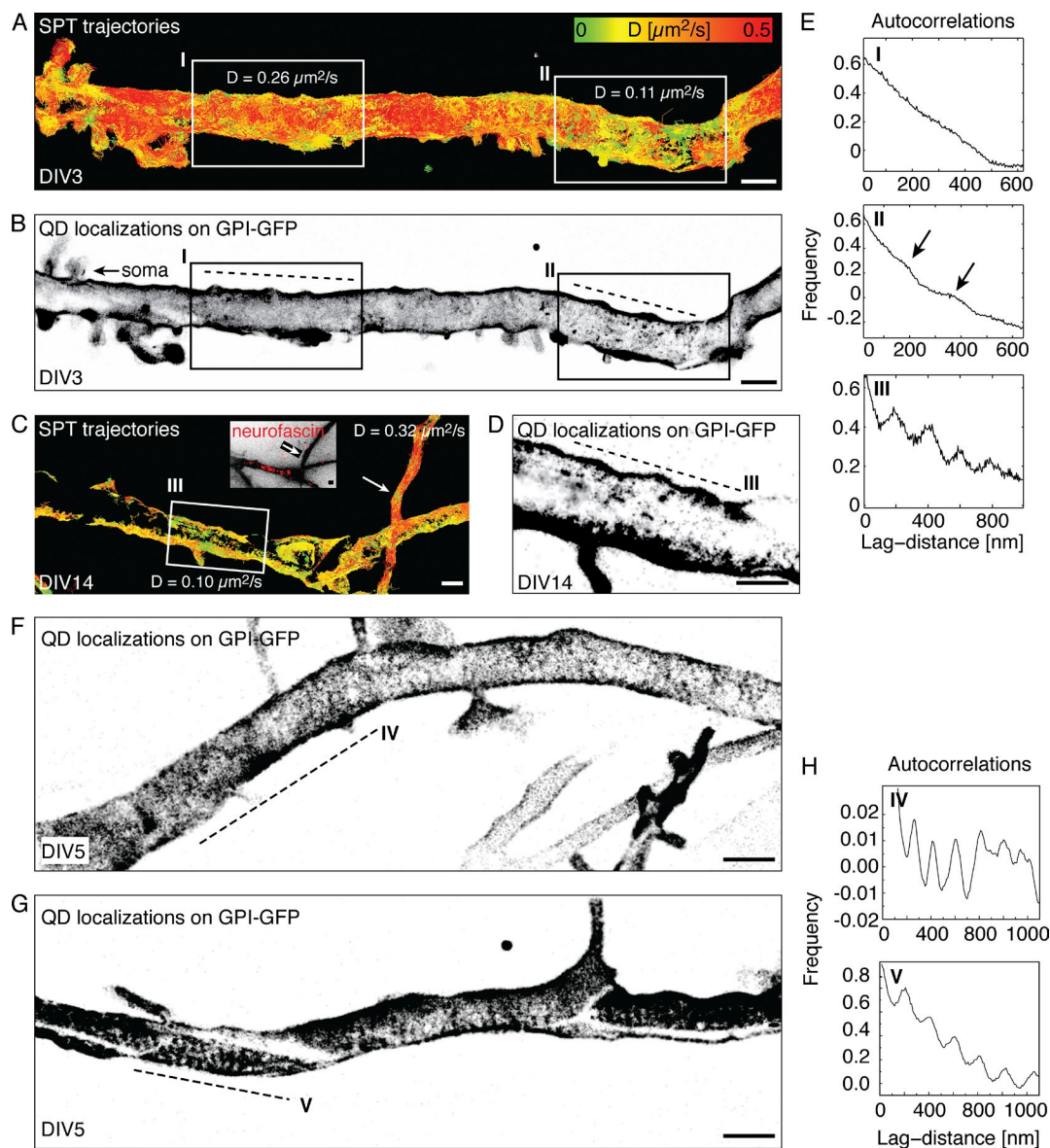
Figure 3. Accumulated positions of GPI-GFP molecules from SPT show a periodic pattern of \sim 190 \text{ nm} along the AIS that emerges as early as DIV3 during development. (A) Plot of SPT trajectories on the proximal axon of a DIV3 hippocampal neuron expressing GPI-GFP color-coded according to the instantaneous diffusion coefficient ( D ). Two areas are emphasized: one with a high (inset I) and one with a lower mean D (inset II). (B) Reconstructed image from all localizations acquired during SPT of QDs corresponding to the trajectories in A. (C) Trajectories color-coded for D on the proximal axon of a DIV14 neuron. In a neurofascin-positive area (inset III), the lateral mobility is reduced compared with the distal axon that loops back to the neuron (arrow). The periodic pattern was observed directly on the AIS in DIV14 neurons. (D) Reconstructed image of all localizations from the SPT experiment in C. (E) Autocorrelations of localizations along the axon (dashed lines) reveal a periodicity of \sim 190 \text{ nm} emerging in areas of low D trajectories in insets II and III, but not in the area of high D in inset I. (F and G) A periodic pattern was observed along the entire proximal axon where the AIS is located but was usually more prominent in some regions (dashed line lines in IV and V). (H) Autocorrelations along segments IV and V show periodically arranged stripes of localizations. Bars, 1 \mu\text{m} .
