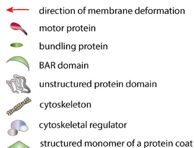
Figure 3. Indirect membrane bending through peripheral exertion of force onto the bilayer. (A and B) Inherently curved proteins, such as the BAR domain protein superfamily, act as scaffolds to introduce curvature. The BAR domain shape is caused by the dimer interface and kinks in the \alpha -helices. This can produce positive curvature, such as that formed by the BAR and FCH-BAR (F-BAR) domain proteins (A), or negative curvature, as formed by inverse BAR (I-BAR) domains (B). (C and D) Scaffold proteins do not need to be curved themselves to deform membranes; curvature can arise from the interactions between monomers or dimers to give either positive (C) or negative curvature (D). (E) Large, unstructured protein regions introduce an asymmetry in the membrane by protein crowding. (F–H) Cytoskeletal proteins can push on membranes to enforce a protrusion (F), constrict the neck of a membrane invagination (G), or pull at tubular/circular membrane compartments with the help of motor proteins (H).
