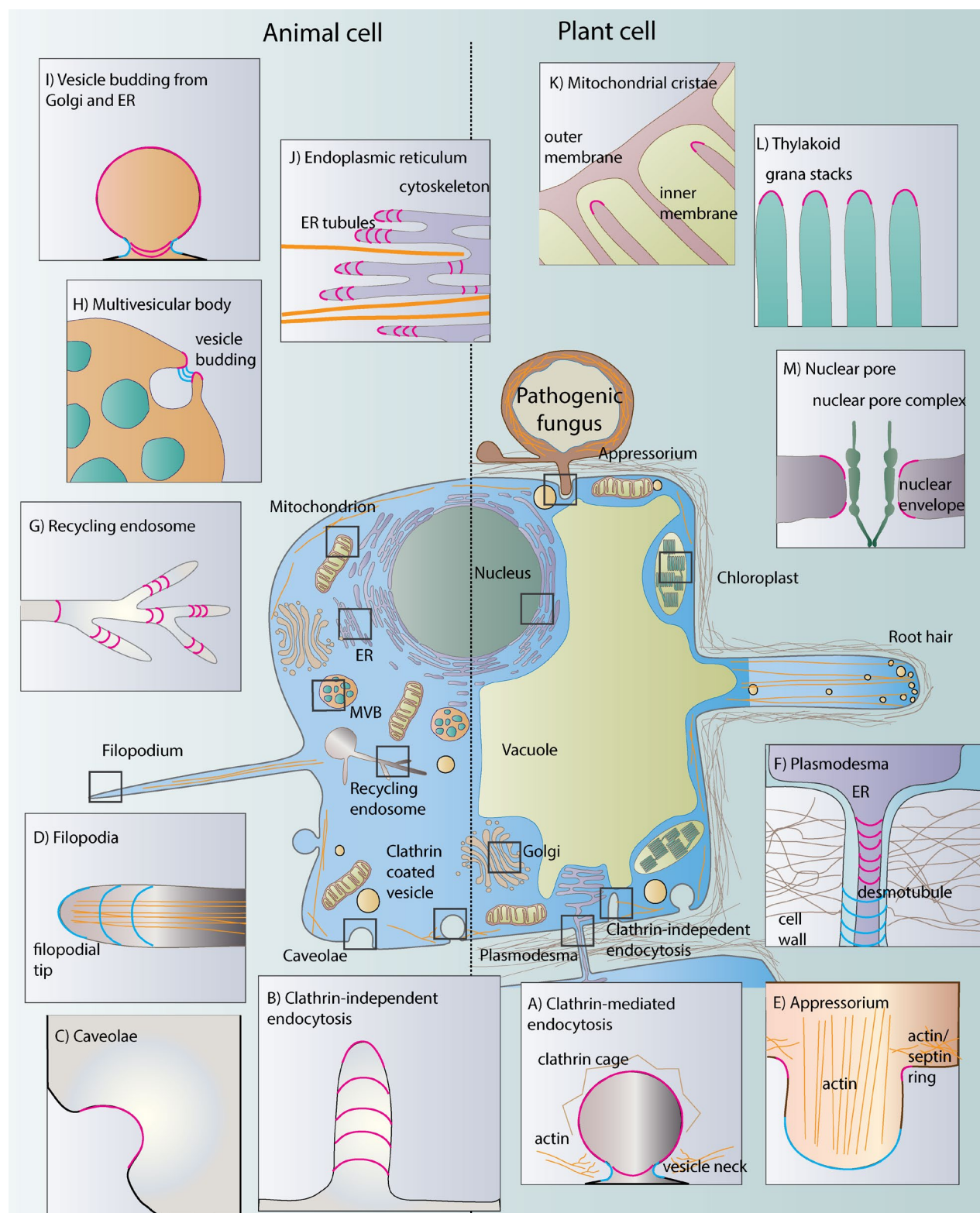
Figure 1. Cell shaping through membrane curvature. We highlight prominent examples of membrane curvature in cells where recent progress has revealed insights into the underlying molecular mechanisms. (A) Multiple bending mechanisms in CME; (B) clathrin-independent endocytosis; (C) caveolae formation; (D) induction of negative curvature at the PM for protrusions like filopodia; (E) bulging of the fungal appressorium; (F) constriction of the PM sleeve and the ER-derived desmotubule at plasmodesmata; (G) dynamic membrane curvature at endosomal tubules; (H) establishment of a protrusion into the MVB to induce vesicle budding; (I) vesicle budding from the ER and Golgi; (J) shaping of morphologically distinct and highly dynamic ER sheets and tubules; (K) sculpting and maintenance of mitochondrial cristae membranes; (L) shaping the surface-maximized grana in plant thylakoids; and (M) assembly and persistence of the nuclear pore complex in the highly bent nuclear envelope. Positive curvature is shown in pink lines, and negative curvature is shown in blue.
