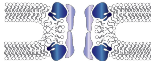
Figure 2. Mechanisms of direct membrane bending within the lipid bilayer. (A) The shape of the lipid molecules gives rise to spontaneous curvature of the membrane, and individual lipids can be curvature promoting. (B) Transmembrane proteins can introduce curvature into the bilayer by the shape of their transmembrane domain. (C) Individual transmembrane protein without curved shapes can bend the membrane via oligomerization and clustering. Interactions with the membrane can be (a) through the formation of single leaflet hairpins; (b) via transmembrane regions; or (c) via protein interactions with lipid receptors. (D) Many curvature-inducing proteins have peptide sequences that are disordered in solution and that fold into \alpha -helices upon interacting with the cell membrane, creating one hydrophobic and one polar face, termed amphipathic helices. The hydrophobic side of the helix penetrates like a wedge into the outer leaflet of the membrane, inducing curvature. (E) Amphipathic helices can cooperate with other proteins, such as the curved scaffold proteins that contain a BAR domain. (F) Amphipathic helices can also be present in the component proteins of large membrane-associated complexes (also called protein coats) and thus anchor them tightly onto the bilayer.
