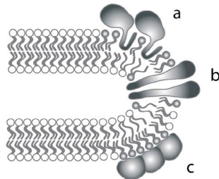
Figure 2. Mechanisms of direct membrane bending within the lipid bilayer. (A) The shape of the lipid molecules gives rise to spontaneous curvature of the membrane, and individual lipids can be curvature promoting. (B) Transmembrane proteins can introduce curvature into the bilayer by the shape of their transmembrane domain. (C) Individual transmembrane protein without curved shapes can bend the membrane via oligomerization and clustering. Interactions with the membrane can be (a) through the formation of single leaflet hairpins; (b) via transmembrane regions; or (c) via protein interactions with lipid receptors. (D) Many curvature-inducing proteins have peptide sequences that are disordered in solution and that fold into \alpha -helices upon interacting with the cell membrane, creating one hydrophobic and one polar face, termed amphipathic helices. The hydrophobic side of the helix penetrates like a wedge into the outer leaflet of the membrane, inducing curvature. (E) Amphipathic helices can cooperate with other proteins, such as the curved scaffold proteins that contain a BAR domain. (F) Amphipathic helices can also be present in the component proteins of large membrane-associated complexes (also called protein coats) and thus anchor them tightly onto the bilayer.
