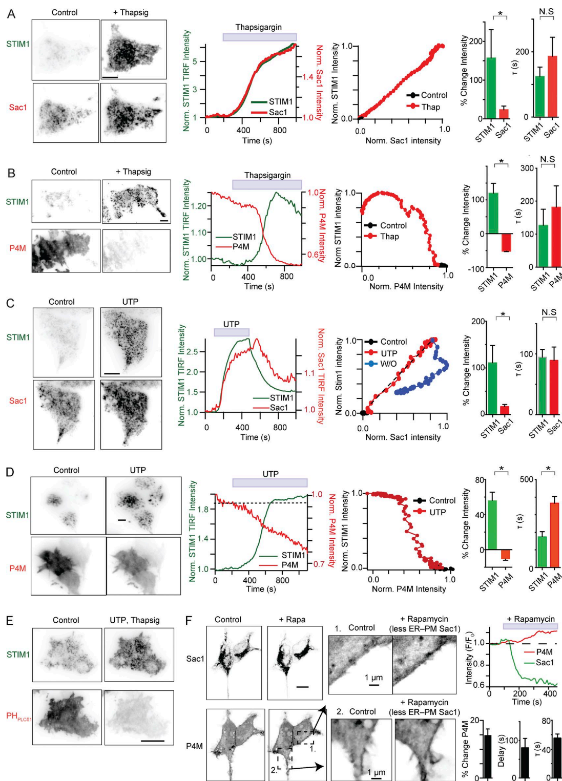
Figure 4. Sac1 at ER-PM junctions reduces PM PI(4)P. (A, left) Inverted TIRF footprint from a single tsA201 cell expressing GFP-STIM1 (top row) and Sac1-mCherry (bottom row), before (left) and after (right) the addition of thapsigargin (500 nM). (second panel) Normalized kinetics of GFP-STIM1 and Sac1-mCherry changes after the addition of thapsigargin. (third panel) Temporal relationship between STIM1 and Sac1 recruitment to the PM (same cell as left panel). (right) Summary of the change in intensity and kinetics of recruitment to the PM of STIM1 and Sac1 (means \pm SEM, n = 11 ). (B) Similar experiments as A, except P4M-mCherry is expressed and monitored (means \pm SEM, n = 9 ). (C) and D) Same experimental design as before, except 100 \mu M UTP is used to initiate STIM1–Orai1 interactions (means \pm SEM, n = 8–13 ). (E) Same experiment as D, except RFP-PH PLCδ1 is expressed. (F, left) Confocal micrographs of two tsA201 cells expressing Sac1 (top) and P4M-mCherry (bottom), before (left) and after (right) the addition of rapamycin (5 \mu M) to recruit the ER to the mitochondria. (middle) Higher magnification confocal images from the regions labeled in A, before (left) and after (right) the addition of rapamycin. (right) (top) Normalized kinetics. (bottom) Summary histograms (means \pm SEM, n = 4 ). All changes in P4M intensity are significantly different compared with no application of rapamycin. Bars, 5 \mu m. N.S., P > 0.05 ; *, P < 0.05 .
