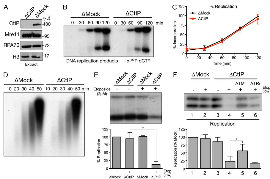
Figure 1. Replication of etoposide-treated chromosomal DNA requires CtIP. (A) CtIP immunodepletion from LSS extracts. Control (ΔMock) and CtIP-depleted extracts (ΔCtIP) were probed with the indicated antibodies. (B) Mock and CtIP-depleted extracts were incubated with sperm nuclei. DNA replication was monitored by agarose gel electrophoresis after incorporation of α-[32P]dCTP into genomic DNA at the indicated time points. (C) Quantification of three independent experiments as shown in B. The mean is plotted, and error bars indicate the standard deviation. (D) Control (mock) and CtIP-depleted extracts were supplemented with sperm nuclei, and DNA replication of Xenopus sperm nuclei was monitored by alkaline gel electrophoresis after incorporation of α-[32P]dCTP into genomic DNA at the indicated time points. (E) DNA replication was monitored as in B in the presence of a low dose (2 μM) of etoposide in mock- or CtIP-depleted extracts, below quantification of three independent experiments (**, P = 0.003 , two-tailed unpaired t test; n = 3 ). (F) Effect of ATM and ATR inhibitors in the sensitivity to low-dose etoposide (2 μM). Bar graph shows quantification of three independent experiments (*, P = 0.014 , two-tailed unpaired t test; n = 3 ).
