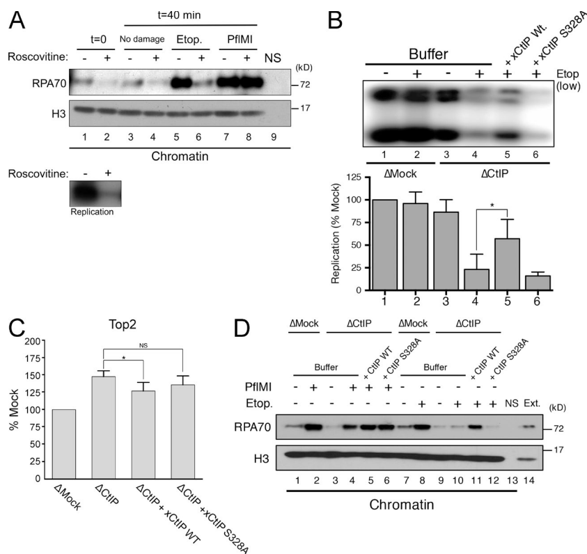
Figure 6. CtIP-BRCA1 interactions are required for CtIP-dependent processing of etoposide-induced DSBs. (A) Control extract (no damage), extracts treated with etoposide (Etop.), or extracts treated with PflMI were incubated with the CDK inhibitor roscovitine. Chromatin was isolated at 0 or 40 min and processed for Western blot with the indicated antibodies. Roscovitine inhibits genomic DNA replication (bottom). (B) Control ( \Delta Mock) and CtIP-depleted extracts ( \Delta CtIP) with or without etoposide were supplemented with sperm nuclei, and replication was monitored by agarose gel electrophoresis after incorporation of \alpha - ^{32} P]dCTP into genomic DNA. CtIP-depleted extracts were supplemented with recombinant xCtIP WT or CtIP-S328A mutant (xCtIP S328A). Bar graph shows quantification of three independent experiments (*, P = 0.026 , two-tailed unpaired t test). (C) Relative quantification of Top2-DNA adducts in CtIP-depleted extracts supplemented with buffer, xCtIP WT, or xCtIP S328A (*, P = 0.035 , two-tailed unpaired t test; NS, not statistically significant [ P = 0.08 ]; n = 3 ). (D) Control ( \Delta Mock) and CtIP-depleted extracts were supplemented with sperm nuclei (5,000/ \mu l) and treated with either PflMI endonuclease or etoposide. CtIP-depleted extracts were supplemented with recombinant xCtIP WT or xCtIP S328A. Chromatin was isolated and processed for Western blotting with the indicated antibodies. NS, no sperm control; Ext., extract.
