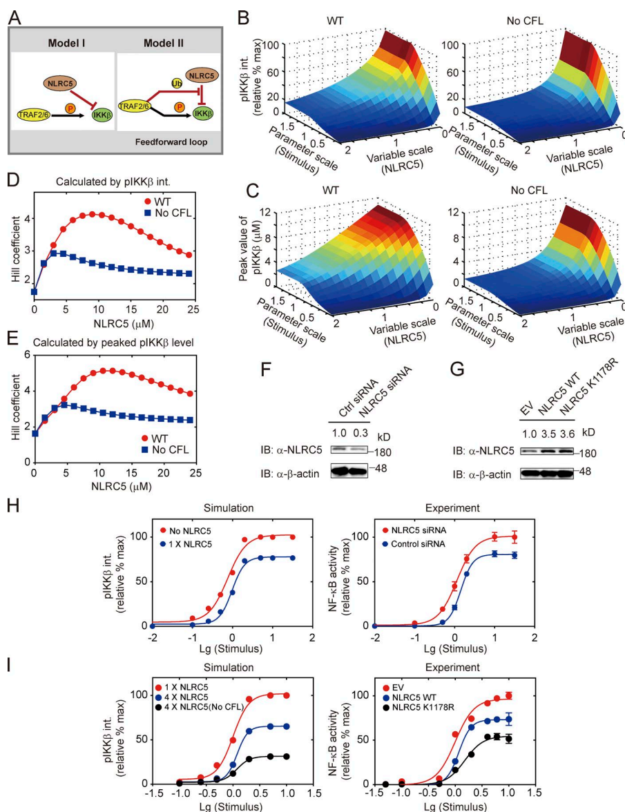
Figure 4. Ubiquitination of NLRC5 by TRAF2/6 creates a feedforward loop to increase the ultrasensitivity of NF-κB signaling.
