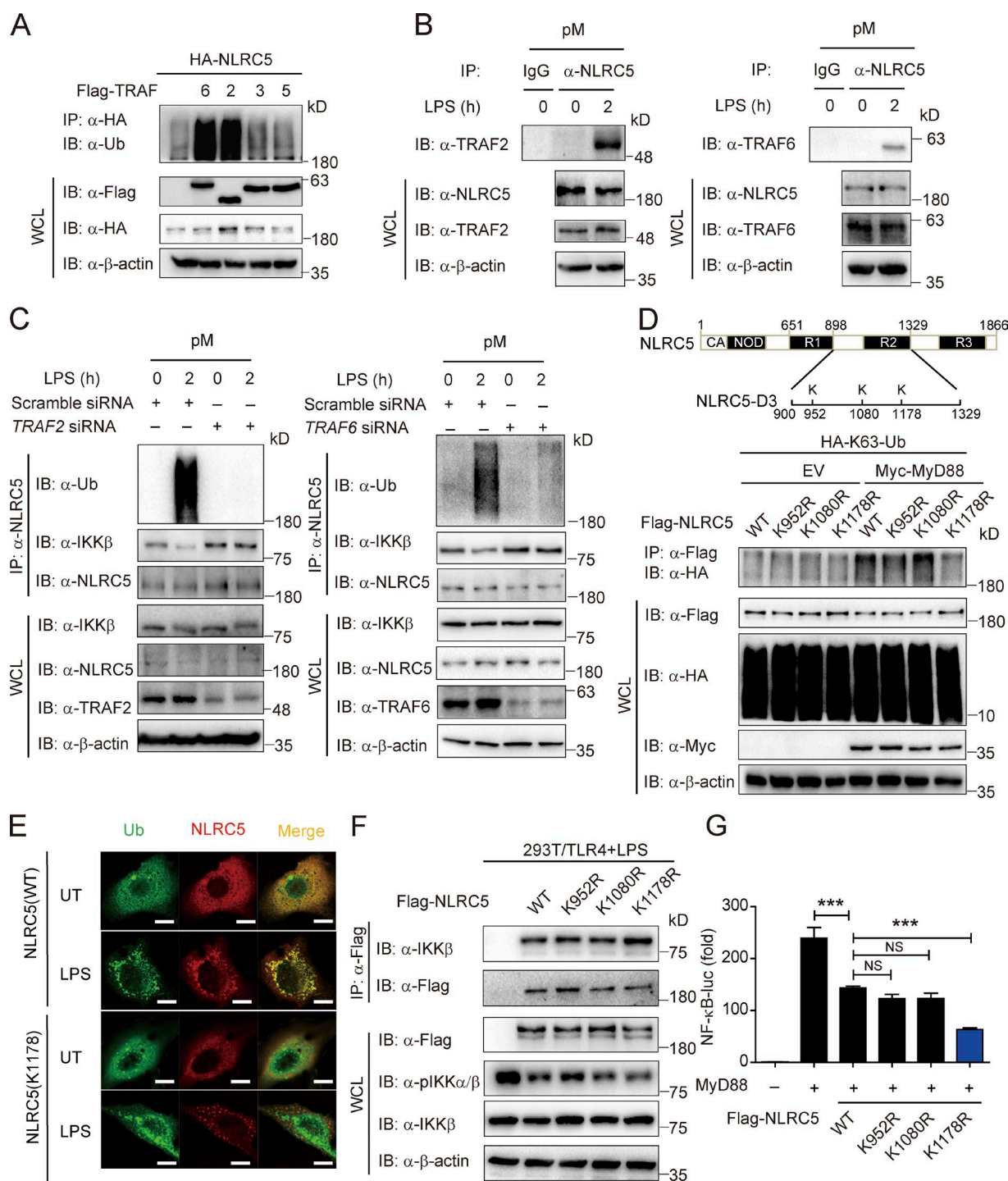
Figure 3. TRAF2 and TRAF6 ubiquitinate NLRC5 at lysine 1,178. (A) HEK293T cells were transfected with plasmids encoding Flag-tagged TRAF6, TRAF2, TRAF3, and TRAF5 and HA-tagged NLRC5. Cell lysates were immunoprecipitated with anti-HA beads followed by immunoblotting with anti-Ub antibody. (B) The interaction between NLRC5 and TRAF2 or TRAF6 in pMs by LPS treatment. (C) The ubiquitination level of NLRC5 and IKK-β-NLRC5 interaction by LPS treatment in WT or TRAF2/6 knockdown pMs. (D) A schematic representation of predicted ubiquitination sites (marked K) in NLRC5 (top). HEK293T cells were transfected with plasmids encoding Flag-NLRC5 or its mutants and HA-K63-Ub with or without Myc-MyD88. Cell lysates were immunoprecipitated with anti-Flag beads and immunoblotted with the indicated antibodies (bottom). (E) Fluorescence microscopy of NLRC5 or K1178R NLRC5 mutant (red) and Ub (green) in HeLa cells with or without LPS stimulation. Bars, 10 μm. (F) HEK293T/TLR4 cells were transfected with plasmids encoding Flag-tagged NLRC5 and its mutants 24 h before LPS (200 ng/ml) treatment. Cell lysates were immunoprecipitated with anti-Flag beads and immunoblotted with the indicated antibodies. (G) Luciferase activity of HEK293T cells transfected with plasmids encoding MyD88, with Flag-NLRC5 and its mutants, together with an NF-κB-luc reporter. ***, P < 0.001 versus the cells with MyD88 overexpression alone (two-tailed Student's t test). Data are representative of at least three independent experiments. n = 3 . Error bars indicate the SEM. IB, immunoblotting; IP, immunoprecipitation; UT, untreated; WCL, whole cell lysate.
