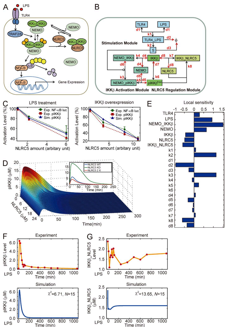
Figure 1. Mathematical model of current NLRC5-IKK-β module cannot reproduce NLRC5-IKK interaction dynamics. (A) Schematic representation of TLR4-mediated NF-κB signaling regulated by NLRC5. (B) The mass action model considering only the competitive interactions between NLRC5 and NEMO to bind IKK-β (model I). (C) Comparison of experimental data from three independent experiments ( n = 3 ; error bars indicate the SD) and simulation results of pIKK-β (the sum of pIKK-β free and NEMO-pIKK-β; Tables S1 and S2) level from model I. (D) Temporal trajectories of total phosphorylated IKK (pIKK-β + NEMO-pIKK-β; also see Tables S1 and S2) with different levels of NLRC5. The inset denotes total pIKK-β dynamics with NLRC5 KO (no NLRC5 protein), WT, and a twofold elevation (2x) of WT. (E) Local sensitivity coefficients for all kinetic parameters and nonzero initial conditions. (F and G) Temporal curves of pIKK-β levels (F) and IKK-β-NLRC5 complex levels (G) upon treatment of RAW264.7 cells with 200 ng/ml LPS adapted from our previous measurements and simulation results by model I. \Phi , null; \chi^2 , the sum of deviations; N , number of experimental points.
