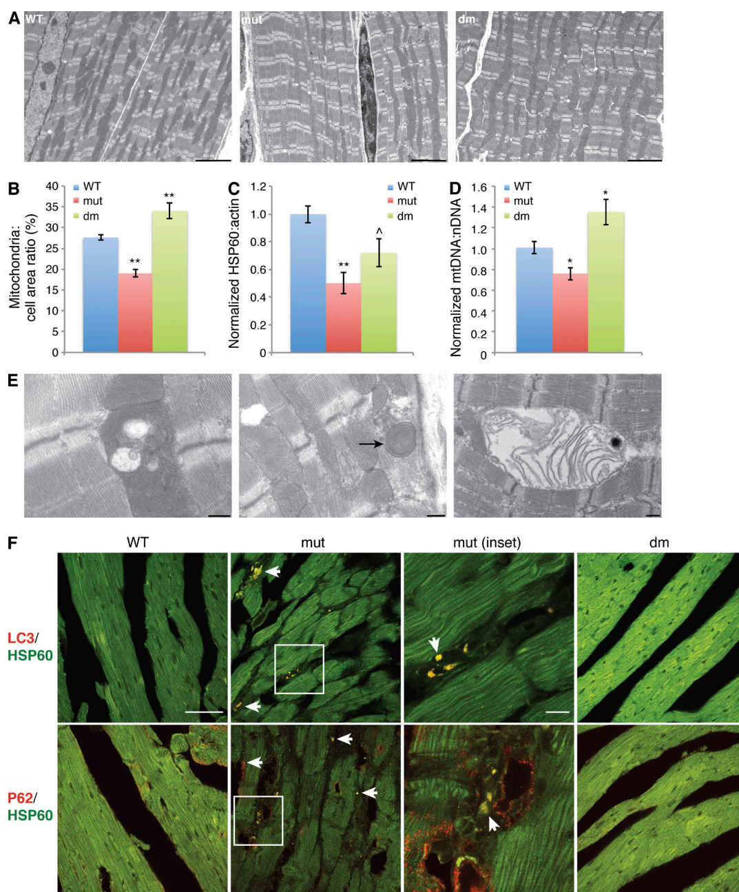
Figure 4. Loss of mitochondria in Mff fl myocardium. (A) Low-magnification EM showing differences in mitochondrial mass. Bars, 5 \mu m. (B) Quantification of mitochondrial area in EM images. (C) HSP60/actin protein ratio, normalized to wild type ( n \geq 7 ). (D) mtDNA per cell, normalized to wild-type content ( n \geq 7 ). (E) EM of mutant myocardium, showing examples of defective mitochondria. Arrow indicates mitophagic structure. Bars, 0.5 \mu m. (F) Heart sections immunostained with LC3 or p62 (red) and HSP60 (green). Arrows indicate positive puncta. Mutant inset is enlarged. Bars: 10 \mu m; (mutant inset) 50 \mu m. Error bars = SEM. P-values as compared with wild type: ^, P \leq 0.05 ; *, P \leq 0.01 ; **, P \leq 0.001 . nDNA, nuclear DNA; WT, wild type.
