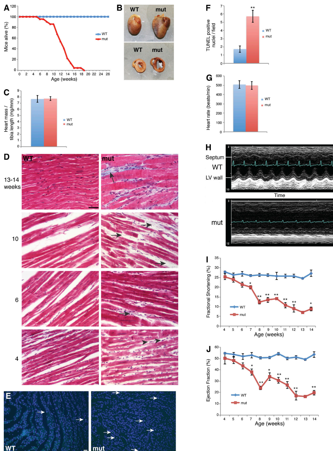
Figure 1. Cardiomyopathy in Mff Δt mice. (A) Survival curve. Mff Δt mutant (mut) mice ( n = 22 ) die by 13 wk on average, as opposed to wild-type controls ( n = 14 ). (B) Increased size, dilation of chambers, and thinning of walls in mutant hearts. (C) Heart mass normalized to tibia length. (D) Masson's trichrome stain of heart sections. Arrowheads indicate fibroblasts. Blue strands (arrows) denote collagen deposition. (E) TUNEL staining of heart sections. Arrows indicate apoptotic nuclei. (F) Quantification of apoptotic nuclei per field ( n \geq 6 ). (G) Heart rate ( n \geq 6 ). (H) M-mode echocardiogram of 13–14-wk-old mice. Electrocardiogram is superimposed. (I and J) Longitudinal echocardiography measuring fractional shortening (I) and ejection fraction (J). Study conducted on 5 wild-type and 10 Mff Δt mice (five mutants died during the course of the study). Error bars = SEM. *, P \leq 0.01 ; **, P \leq 0.001 . Bars, 50 \mu m. WT, wild type.
