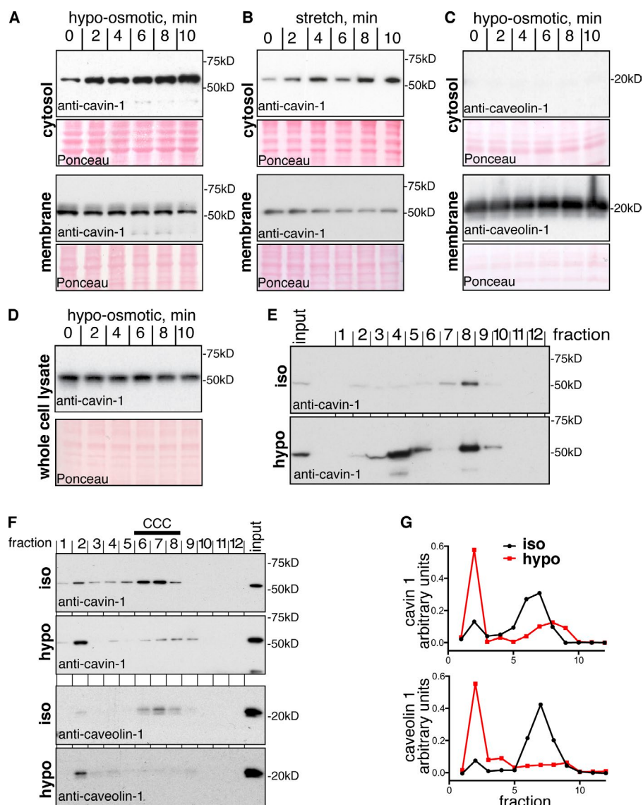
Figure 1. Loss of plasma membrane caveolae under mechanical force is accompanied by disassembly of caveolar protein complexes.
