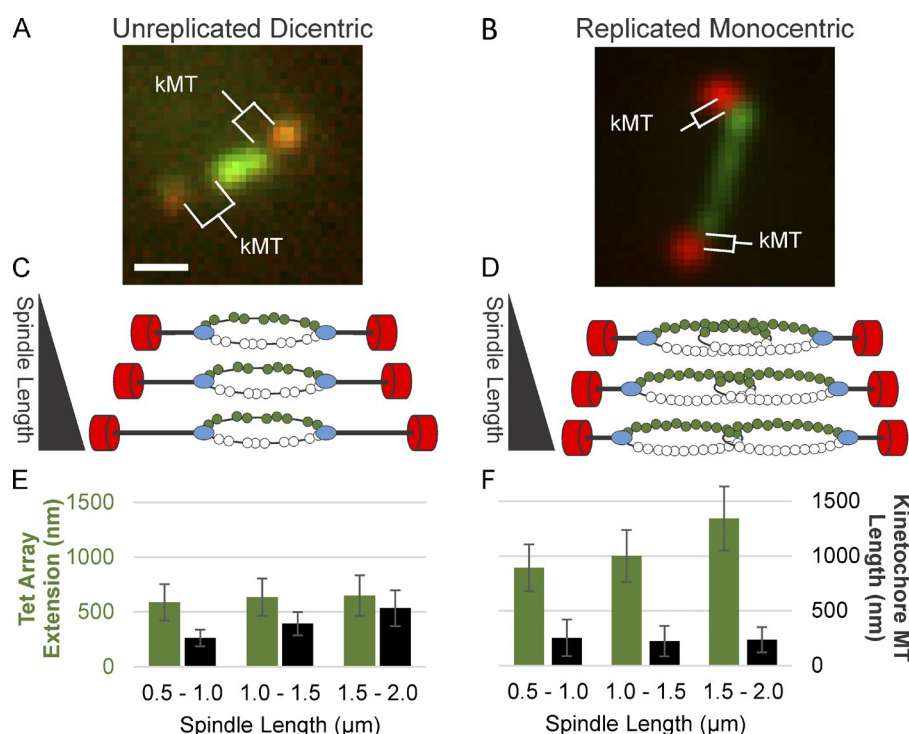
Figure 4. Tension along the spindle axis promotes microtubule growth. TetO array extension and kMT length in unreplicated, dicentric plasmids versus replicated, monocentric plasmids. Image of metaphase yeast containing an unreplicated, dicentric plasmid (A) and a replicated, monocentric plasmid (B). Schematic of a spindle containing an unreplicated, dicentric plasmid (C) and a replicated, monocentric plasmid (D). SPBs are shown in red, kinetochores are shown in blue, and DNA is shown in green. Tet array extension and kMT length versus spindle length for unreplicated, dicentric plasmids (E) and for replicated, monocentric plasmids (F). Bar, 0.5 μm. Error bars are standard deviation. The data shown are from multiple experiments (dicentric, n = 43 arrays; replicated monocentric, n = 54 ).
