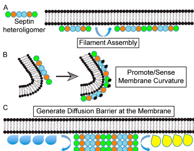
Figure 3. Septins assemble on and organize membranes. (A) Membrane association of septin heteroligomers promotes assembly of septin filaments. (B) Septins may play a role in promoting or sensing membrane curvature. Posttranslational modifications (indicated by black stars) are implicated in this function. (C) By providing a diffusion barrier, septins play a role in compartmentalizing the membrane.
