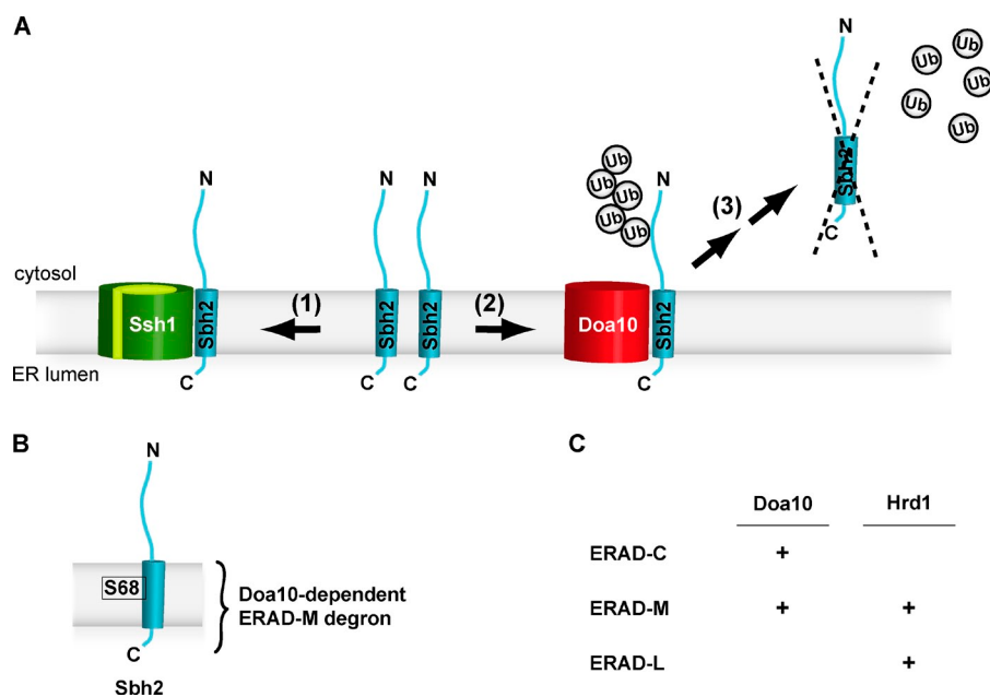
Figure 6. Model for Sbh2 quantity control via a Doa10-dependent intramembrane degon. (A) The TA Sbh2 protein associates with the Ssh1 protein in the ER membrane (1). Together with a third integral membrane protein, Sss1 (not depicted), Ssh1, and Sbh2 form the heterotrimeric Ssh1 complex implicated in cotranslational protein translocation in S. cerevisiae (besides the heterotrimeric Sec61 complex). Assembled Sbh2 is stable/protected from degradation. In contrast, unassembled Sbh2 (e.g., in ssh1Δ cells or surplus Sbh2 in WT cells) is readily degraded via a Doa10-dependent ERAD pathway involving ubiquitylation (2), retrotranslocation, and proteasomal degradation of Sbh2 (3). Ub, ubiquitin. (B) Schematic depiction of the Doa10-dependent intramembrane (ERAD-M) degon of Sbh2. The degon encompasses the Sbh2 TM domain and the short ER-luminal domain. The serine residue at position 68 (S68) located within the Sbh2 TM helix is a crucial part of the degon. (C) Assignment of the two major S. cerevisiae ERAD E3 ligases to different ERAD substrate classes. The identification of a Doa10-dependent ERAD-M substrate, Sbh2, allows assigning Doa10 to the ERAD-M pathway.
