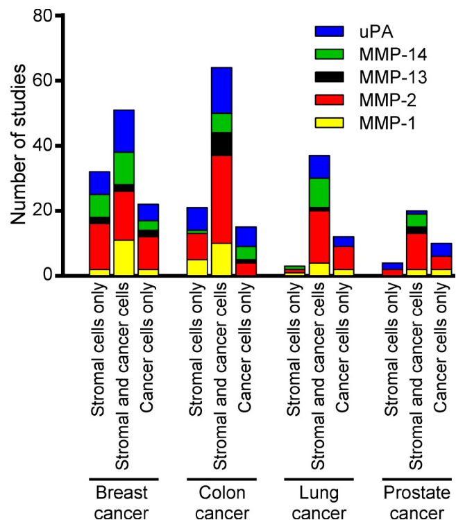
Figure 2. Localization of extracellular matrix-degrading proteases in human cancer. Compilation of expression localization data for MMP-1, MMP-2, MMP-13, MMP-14, and uPA obtained from 291 published studies of human breast, colon, lung, and prostate cancer ( supplemental text ). The bar graphs show the number of studies reporting the expression of any of the proteases in stromal cells only, both cancer and stromal cells, and cancer cells only.
