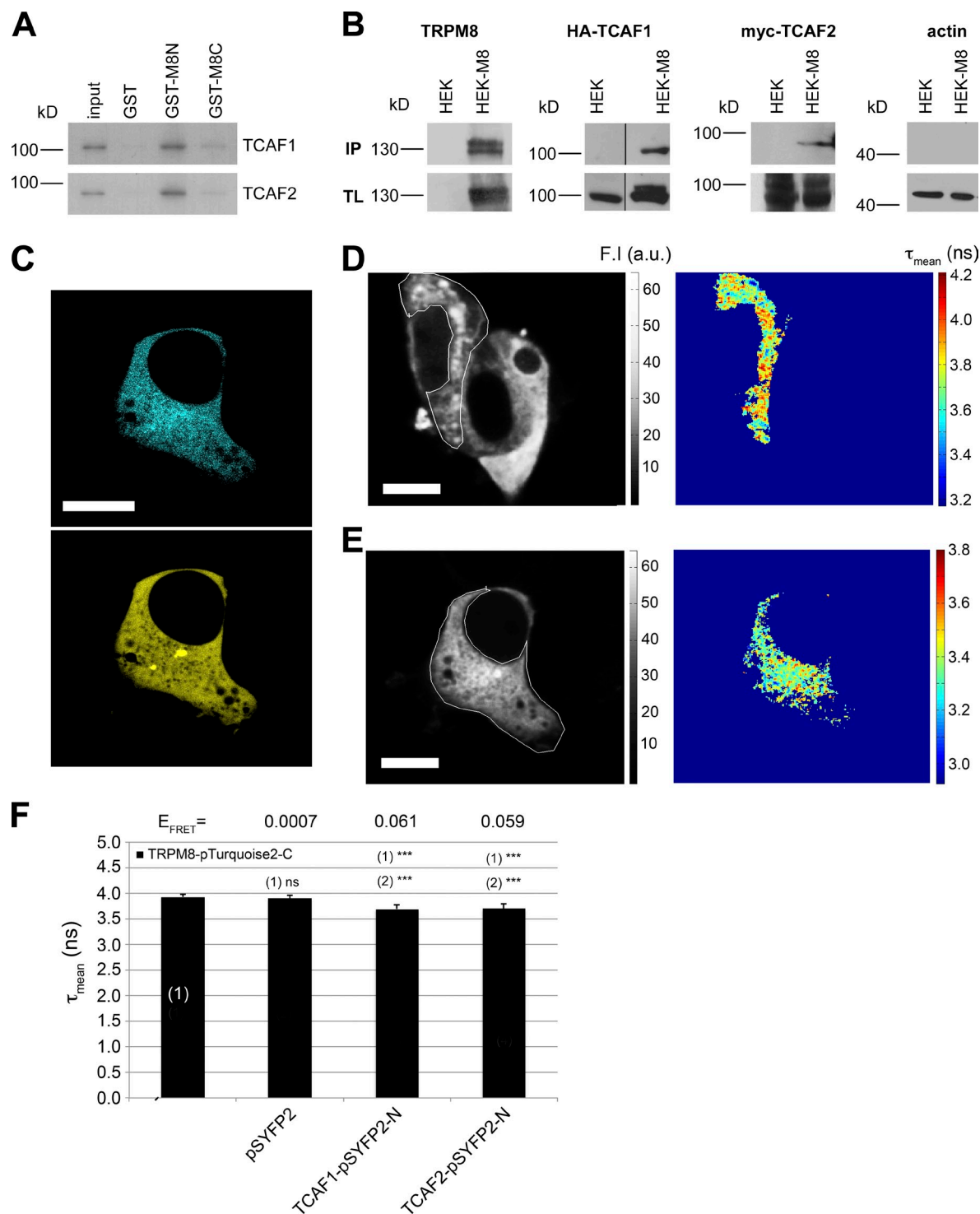
Figure 3. TCAFI and TCAF2 interact and colocalize with TRPM8. (A) GST pull-down assay using [ ^{35}\text{S} ]methionine-labeled TCAFI or TCAF2 protein and GST or GST fused to the TRPM8 N-terminal tail (GST-M8N) or C-terminal tail (GST-M8C). (B) Cells transfected with HA-tagged TCAFI or myc-tagged TCAF2 with (HEK-M8) or without (HEK) his-tagged full-length TRPM8, and total lysates (TL) were used for immunoprecipitation and subsequent immunoblot analysis. Immunoprecipitation of the channel was confirmed by immunoblotting for TRPM8, and the coimmunoprecipitation of TCAFI or TCAF2 proteins was detected using an anti-HA or anti-myc antibody, respectively, on the immunoprecipitated complex (IP). No coimmunoprecipitation was detected in control immunoblots for actin. The black lines on the HA-TCAFI blots indicate the removal of intervening lanes for presentation purposes. (C–F) TCAFI/2-to-TRPM8 binding was assessed by measuring FRET with TM FLIM in HEK293 cells after a 24-h transfection. The TCSPC approach was chosen to achieve a good spatial resolution, which would allow discriminating TRPM8-ER localization. (C) An example of concomitant expression of TRPM8-mTurquoise2 (cyan) and TCAFI-SYFP2 (yellow). (D and E) Representative FRET-FLIM images for TRPM8-mTurquoise alone and for TRPM8-mTurquoise + TCAFI-SYFP2, respectively. Grayscale-coded fluorescence images of the donor of FRET (left images in D and E; fluorescence intensity [FI] is given in arbitrary units [a.u.]) were analyzed by the phasor plot method (Phasor) to compute FLIM images ( \tau_{\text{mean}} ) showing the mean lifetime (ns; right images of D and E). The outlines define the regions of interest for which mean lifetime of the donor of fluorescence was calculated. Bars, 10 \mu\text{m} . (F) Chart representing the mean lifetime of TRPM8-mTurquoise2 alone, coexpressed with the negative control SYFP2, or with TCAFI-SYFP2 or TCAF2-SYFP2. FRET efficiency ( E_{\text{FRET}} ) is shown on the top of the chart. Values are presented as means \pm SD (error bars). ***, P < 0.001 .
