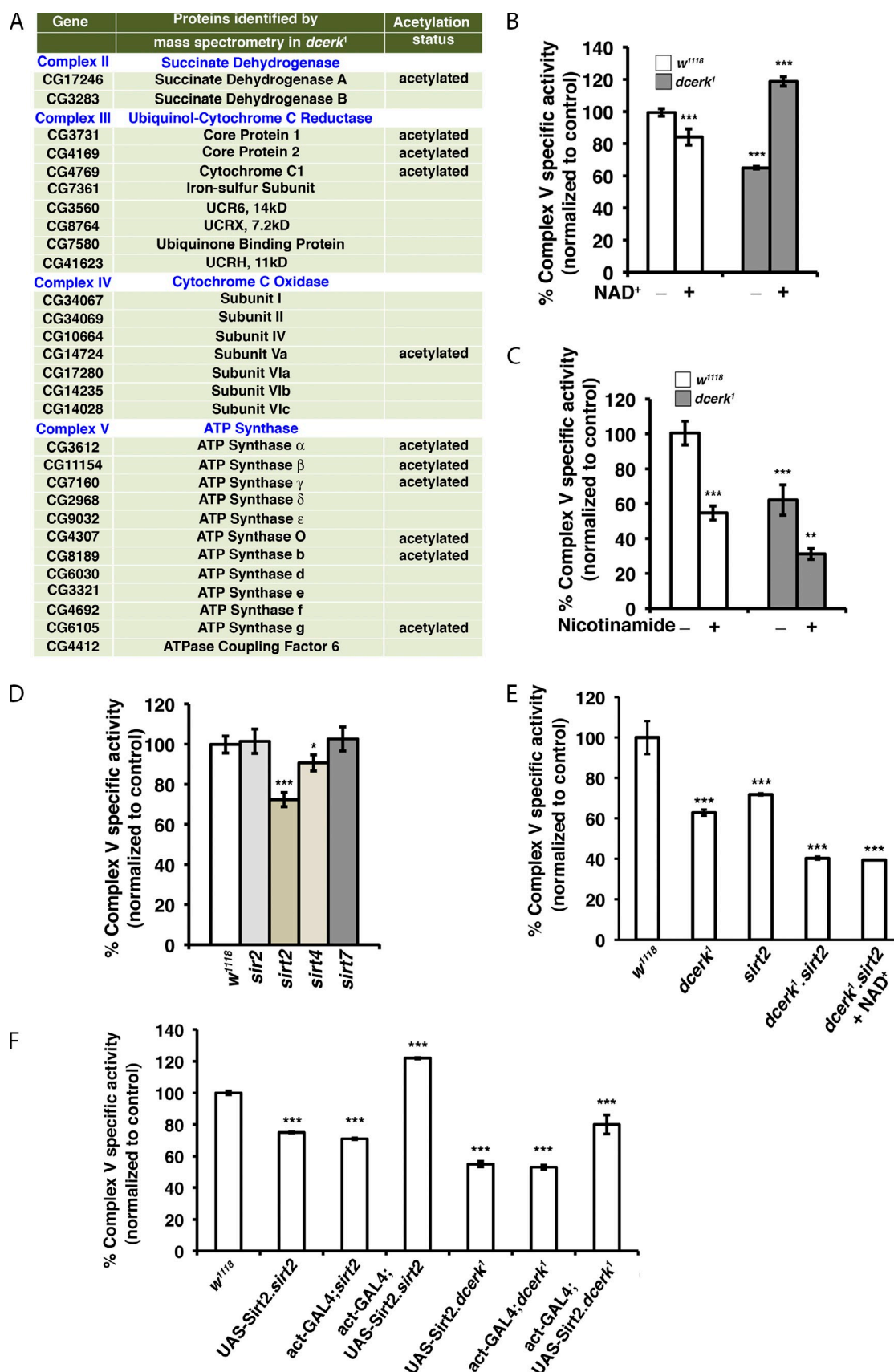
Figure 2. dcerk 1 mutants show acetylation of many OXPHOS subunits and decrease in complex V activity, which is rescued by supplementing NAD + and inhibited by nicotinamide. dSirt2 regulates complex V activity in dcerk 1 mutants. (A) BN-PAGE-separated bands from dcerk 1 were digested with trypsin and subjected to LC-MS/MS to identify the different subunits of the complexes and the subunits that are acetylated. (B) dcerk 1 mitochondria show a 40% reduction in complex V activity. Supplementing with NAD + restores complex V activity in dcerk 1 . Complex V activity was normalized to the activity of
