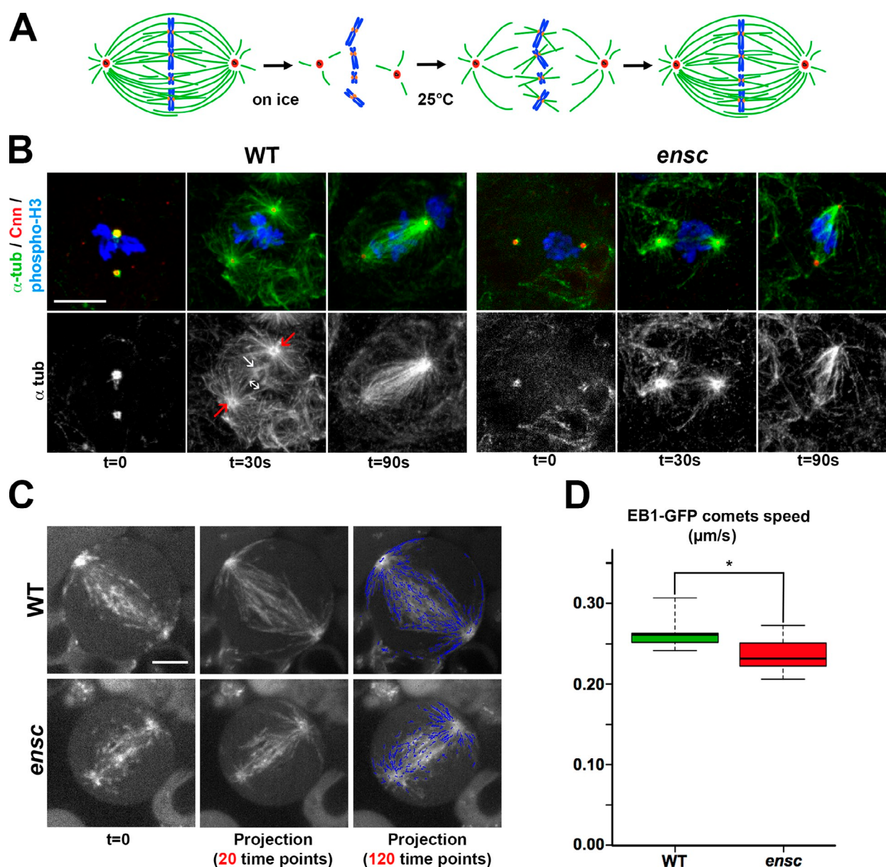
Figure 3. Ensconsin mutant Nbs display defective spindle reassembly and a lower Mt velocity in live cells. (A) Mt regrowth assay. Mts were depolymerized on ice (see Materials and methods), and spindle reformation was analyzed by immunostaining after the cells had been returned to 25°C conditions. (B) In the WT (left), Mts were depolymerized after 30 min at 0°C. Numerous Mts were nucleated by the centrosomes after 30 s at 25°C (red arrows). Small asterisks are visible around the chromatin (white arrow), together with Kt fibers (double-ended arrow). At 90 s, the spindles have a normal shape. In ensc mutant cells (right), only centrosomal Mts can be visualized after 30 s, and the spindles remain short and disorganized after 90 s. Centrosomes are shown in red (centrosomin, cnn ), Mts ( \alpha tub) in green (gray in the lower panels), and phospho-H3 in blue. Bar, 10 \mu m. (C) Control (top) and ensc (bottom) Nbs expressing EB1-GFP were imaged by time-lapse microscopy (Video 8). A single frame (in which EB1-GFP comets are visible) is presented (left), with time projections for the 20- and 120-min time points (middle and right, respectively). Blue lines represent EB1-GFP tracks after filtering (see Materials and methods). Bar, 4 \mu m. (D) Quantification of Mt velocity in WT ( n = 17 ) and ensc mutant ( n = 16 ) mitotic Nbs: 0.26 and 0.23 \mu m/s, respectively (*, P = 1.2 \times 10^{-4} ).
