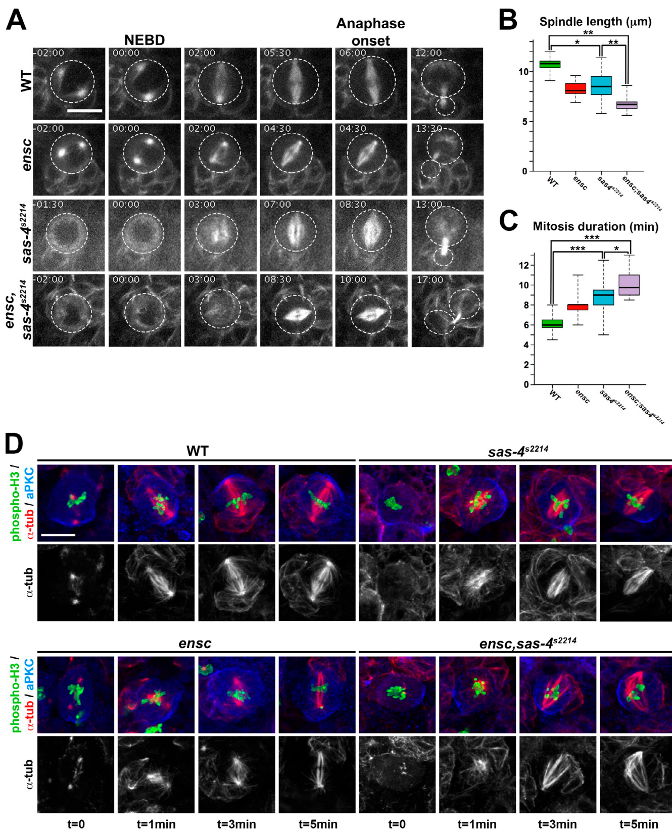
Figure 4. Ensconsin-dependent spindle assembly defects are enhanced by centrosome ablation. (A) Cell division of WT, ensc , sas-4 s2214 , and ensc, sas-4 s2214 double mutant Nbs expressing \beta -tubulin-GFP. Time is given in minutes:seconds. The circles indicate the contours of the cells. Bar, 10 \mu\text{m} . (B) Analysis of mitotic spindle length in WT (green), ensc (red), sas-4 s2214 (blue), and ensc, sas-4 s2214 (purple) mutant Nbs. Spindle length was 10.7 \pm 0.7 \mu\text{m} in the WT ( n = 15 ), 8.2 \pm 1.2 \mu\text{m} in the ensc mutant ( n = 23 ), 8.5 \pm 1.4 \mu\text{m} in the sas-4 s2214 mutant ( n = 45 ), and 6.7 \pm 0.7 \mu\text{m} in the ensc, sas-4 s2214 double mutant ( n = 31 ). *, P = 2 \times 10^{-6} ; **, P < 5.2 \times 10^{-8} . (C) Analysis of the duration of mitosis in WT (green), ensc (red), sas-4 s2214 (blue), and ensc, sas-4 s2214 (purple) mutant Nbs. The time between NEBD and anaphase onset was 6.1 \pm 0.9 \text{ min} for the controls ( n = 23 ), 8.0 \pm 1.2 \text{ min} for the ensc mutant ( n = 37 ), 9.0 \pm 1.2 \text{ min} for the sas-4 s2214 mutant ( n = 48 ), and 10.0 \pm 1.2 \text{ min} for the ensc, sas-4 s2214 double mutant ( n = 38 ). *, P = 1.8 \times 10^{-3} ; ***, P < 1 \times 10^{-10} .
