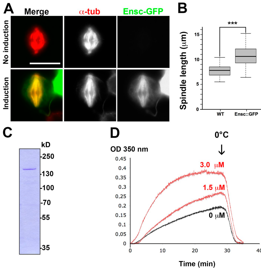
Figure 5. Ensconsin promotes Mt growth in cells and in vitro. (A) Ensconsin (Ens) overproduction in mitotic S2 cells led to the formation of longer spindles. Ensconsin-GFP is green (gray in the panels on the right) and Mts are shown in red (gray in the middle panels). Exogenous Ensconsin-GFP is localized on the mitotic spindle during mitosis. Bar, 10 \mu\text{m} . (B) Analysis of mitotic spindle length in WT ( n = 56 ) and Ensconsin-GFP-overexpressing mitotic S2 cells ( n = 26 ). ***, P = 5.1 \times 10^{-11} . (C) Recombinant Ensconsin purified, separated by SDS-PAGE, and stained with Coomassie blue. (D) Effect of Ensconsin on Mt polymerization in vitro. Purified porcine brain tubulin was mixed with polymerization buffer supplemented with either PBS or PBS containing Ensconsin on ice. Mt polymerization was induced by heating at 35°C. Absorbance at 350 nm was monitored to evaluate the formation of Mt polymers. After 28 min, the samples were shifted to 0°C to estimate protein aggregation. Ensconsin increased the rate of Mt polymerization and the total number of polymers in a dose-dependent manner (red curves), as shown by comparison with buffer alone (black curve).
