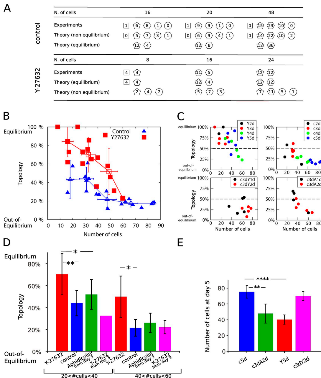
Figure 5. Relaxation of cortical tension via inhibition of ROCK drives topology toward equilibrium, independent of cell division rate. (A) The table reports the experimentally observed and theoretically predicted topological configurations of a subset of control (top) and (bottom) MDCK cysts treated with Y-27632 to inhibit ROCK activity. Each line of the table represents, for a given number of cells in the cyst (top rows), the number of cells displaying four, five, six, seven, and eight neighbors. The topology of control cysts is never consistent with equilibrium and approaches the nonequilibrium topology for increasing numbers of cells, as expected from the theory. (B) After reconstructing the 3D structure of treated and untreated cysts, we calculated the distance from equilibrium and plotted it as a function of the number of cells. The topology of control cysts (closed blue triangles) is clearly closer to the nonequilibrium distribution, whereas Y-27632-treated cysts (closed red squares) are closer to equilibrium, especially when the number of cells is small. Here Y-27632 is given right after seeding. Open symbols are medians on series of data ( n = 0-20 , 20-40 , 40-80 , and 80-100 ), and lines are a guide to the eye. The data shown are from a total of n = 34 cysts, each containing between 10 and 90 cells, coming from a single experiment. (C) Topology of cysts at different times: untreated (top right), Y-27632 given from seeding (top left), Y-27632 given from day 3 (bottom left), and Aphidicolin given from day 3 (bottom right). Labels: c, control; Y, Y-27632; A, Aphidicolin; 1d/2d/3d, 1/2/3 d; and c3dY1d, untreated for 3 d, then treated with Y-27632 for 1 d; c3dA2d, untreated for 3 d, then treated with Aphidicolin for 2 d. Y-27632-treated cysts (top left) lie systematically in the half plane closer to equilibrium with respect to control cysts (top right) and contain on average a smaller number of cells (at a given time from seeding), due to the slowdown of cell division induced by Y-27632. Each point corresponds to the topology of a single cyst. (D) To account for the differences in topology, different groups of cysts were compared by means of a one-tailed Welch's test to assess for statistical significance, where the existence of a difference in the mean value of the topology was used as a null hypothesis. Cysts with 20–40 cells (left) and 40–60 cells (right) were grouped and compared. A statistically significant difference is seen between Y-27632-treated (left, n = 7 ; right, n = 6 ) and control (left, n = 7 ; right, n = 4 ) for any number of cells. As for other treatments, such as Aphidicolin (left, n = 5 ; right, n = 3 ) or Y-27632 given from day 3 (left, n = 1 ; right, n = 2 ), the topology is different from the Y-27632-treated cysts, resembling the untreated case, albeit not significantly. Asterisks indicate statistical significance: *, P < 0.05 ; **, P < 0.01 ; ***, P < 0.001 , etc. Error bars indicate standard deviations. (E) The effect of the different treatments on cell division was assessed by means of statistical comparison (Welch's Test) of different groups. The number of cells in the cysts at day 5 was compared in the different populations. All cases have n = 5 samples. Error bars indicate standard deviations.
