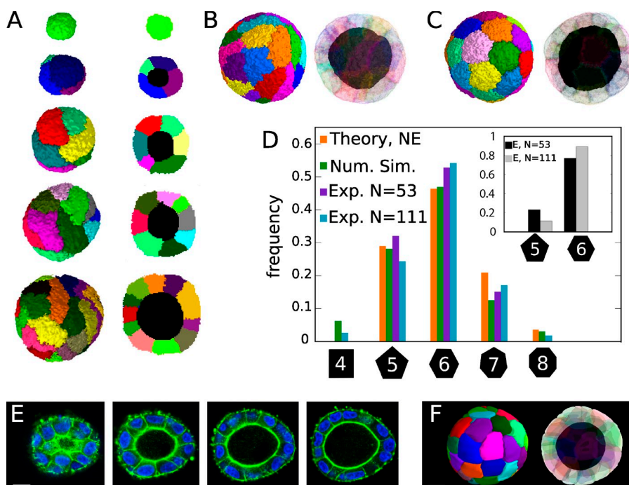
Figure 1. Cysts are spherical monolayers out of mechanical equilibrium. (A) Computational simulation of cyst morphogenesis from 1 (top) to 32 cells (bottom), under nonequilibrium conditions and with control of the cell-division axis. The cross section (right) shows the presence of a single spherical lumen. The left column is the external overview of the cyst. Equivalent time from seeding is around 4 d. (B) Numerical simulation of a cyst with 32 cells out of equilibrium. (C) The same cyst as in B, after relaxation to equilibrium. (D) Analytical nonequilibrium topological distribution (orange; Gibson et al., 2006) and numerical simulations results (green). Normalized frequency of contacts for two MDCK cysts ( n = 53 cells, blue; and n = 111 cells, cyan) obtained by 3D reconstructions of confocal scans. (inset) Theoretical equilibrium topology distributions for two cysts of n = 53 (black) and n = 111 cells (gray). The result of equilibrium numerical simulations is identical (not depicted). (E) Four confocal scans of the same cyst from bottom (left) to equator (right), stained with DAPI (blue) and phalloidin (green). Time from seeding: 4 d. Bar, 10 \mu\text{m} . (F) 3D computer-assisted reconstruction of the cyst geometry of E from the full confocal scans. External overview (left) and cross section (right). Each cell is identified with a unique color for ease of visualization. Bar, 10 \mu\text{m} .
