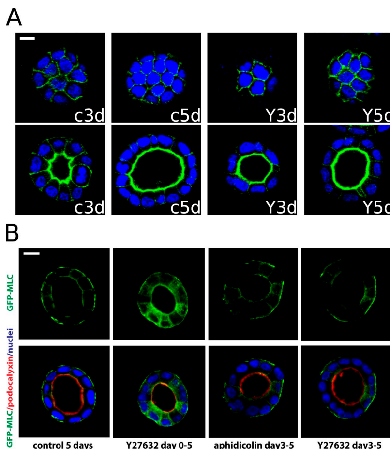
Figure 4. ROCK inhibition alters the cellular spatial distribution of MLC. (A) Representative micrographs of top (top) and mid sections (bottom) of cysts fixed at days 3 and 5 grown under no treatment (c3d and c5d) and treated with Y-27632 (Y3d and Y5d). Cysts were stained with DAPI and phalloidin. Bar, 10 \mu m. (B) We used GFP-MLC as an indicator for cortical tension (Yu et al., 2003). MDCK cells expressing GFP-MLC were cultured in Matrigel solution. Aphidicolin and Y-27632 were applied separately from day 0 or day 3. Cells were then fixed at day 5 and stained for PCX and nuclei. In control cysts, MLC is concentrated at the basal surface in an untreated cyst. When Y-27632 is applied from day 0, MLC is no longer accumulated at the basal surface, and instead is diffuse in the cytoplasm. In contrast, Aphidicolin does not change the localization pattern of MLC, which remains mainly at the basal surface. For a more detailed quantification of this effect see Fig. S5. Bar, 20 \mu m.
