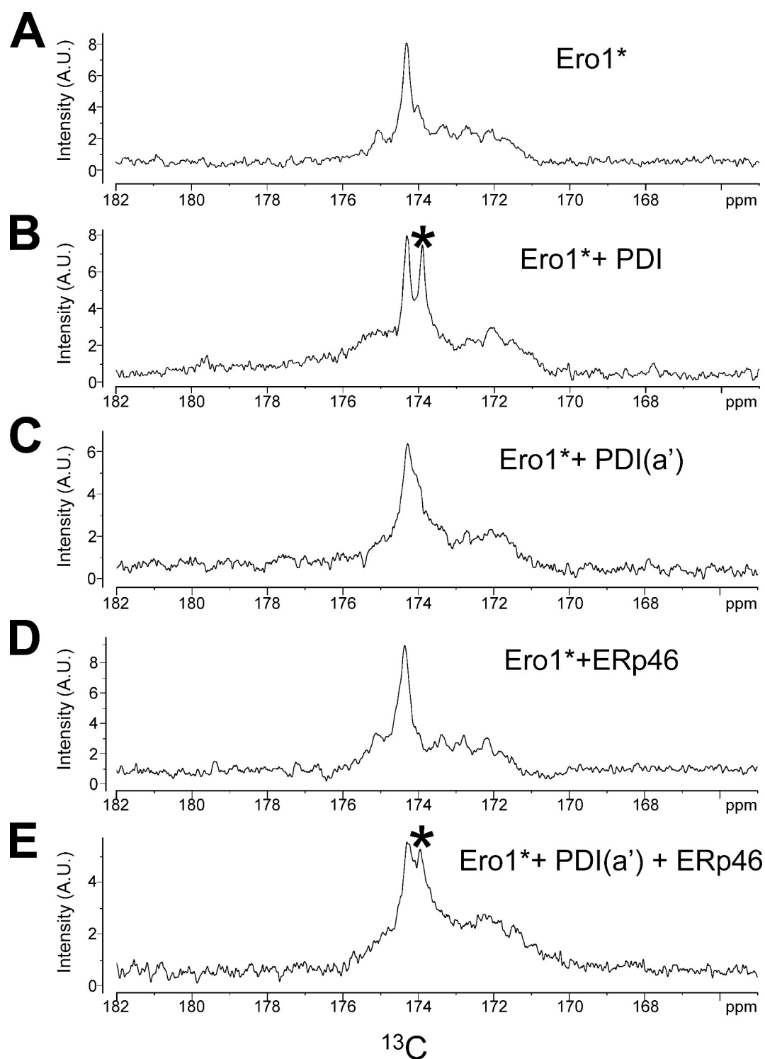
Figure 5. ERp46 substitutes for the a domain of PDI and increases conformational flexibility in a shuttle cysteine, Cys99, of Ero1- \alpha . ^{13}\text{C} NMR spectra of the constitutively active Ero1- \alpha (C104A/C131A) labeled with ^{13}\text{C} selectively at the carbonyl carbons of cysteine residues (Ero1*). (A–E) Spectra were measured in the absence (A) and presence of equimolar amounts of PDI (B), PDI(a') (C), ERp46 (D), or PDI(a') and ERp46 (E). Spectrum of the unlabeled protein has already been subtracted. PDI(a') or ERp46 had no apparent effect on the mobilization of Cys99. The asterisk indicates the peak originating from Cys99. A.U., arbitrary unit.
