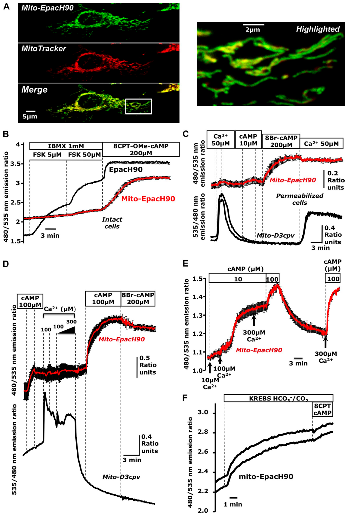
Figure 1. Cyclic AMP produced in the cytosol does not reach the mitochondrial matrix. (A) Confocal images of HeLa cells expressing mito-EpachH90 and loaded with MitoTracker red suggesting proper localization of mito-EpachH90. (B) cAMP measurements in intact cells expressing cytosolic EpachH90 (black trace) or mito-EpachH90 (red trace; mean of five cells); typical of n = 9 experiments; 34 mito-H90, 19 Epach-H90 cells. (C) Digitonin-permeabilized
