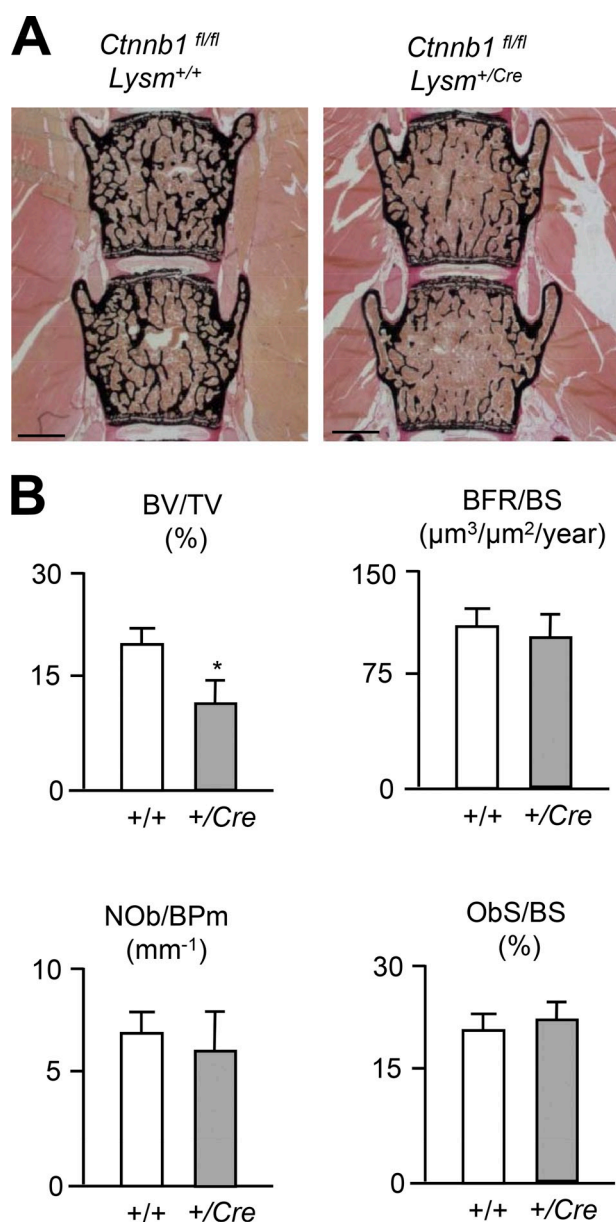
Figure 7. Phenotypic analysis of Ctnnb1 fl/fl /LysM +/cre mice. (A) Von Kossa/van Gieson-staining of non-decalcified spine sections from 12-wk-old Ctnnb1 fl/fl /LysM +/+ and Ctnnb1 fl/fl /LysM +/cre mice. Bars, 1 mm. (B) Histomorphometric quantification of trabecular bone volume (BV/TV), bone formation rate (BFR/BS), osteoblast number (Ob.N/B.Pm), and osteoblast surface (ObS/BS) in the same mice. All error bars represent mean \pm SD ( n = 6 ). Asterisks indicate statistically significant differences between the two groups.
