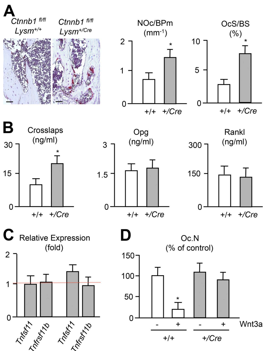
Figure 8. Opg-independent increase of osteoclastogenesis in Ctnnb1 fl/fl /LysM +/-cre mice. (A) TRAP activity staining on spine sections shows increased osteoclastogenesis in Ctnnb1 fl/fl /LysM +/-cre mice. Histomorphometric quantification of osteoclast number (Oc.N/B.Pm) and osteoclast surface (OcS/BS) is given on the right. Bars, 50 \mu m. (B) Concentrations of collagen degradation products (Crosslaps), Opg, and Rankl in the serum of Ctnnb1 fl/fl /LysM +/- and Ctnnb1 fl/fl /LysM +/-cre mice. All error bars represent mean \pm SD ( n = 6 ). Asterisks indicate statistically significant differences between the two groups. (C) qRT-PCR expression analysis of the indicated genes in marrow-flushed bones (left) or in bone marrow-derived osteoclast cultures (right) from Ctnnb1 fl/fl /LysM +/-cre mice relative to Ctnnb1 fl/fl /LysM +/- littermates. Error bars represent mean \pm SD ( n = 4 ). (D) Quantification of TRAP-positive multinucleated cells in Ctnnb1 fl/fl /LysM +/- and Ctnnb1 fl/fl /LysM +/-cre bone marrow cells differentiated by addition of M-CSf, Rankl in the absence or presence of Wnt3a, as indicated. All error bars represent mean \pm SD ( n = 6 ). Asterisks indicate statistically significant differences compared with untreated controls.
