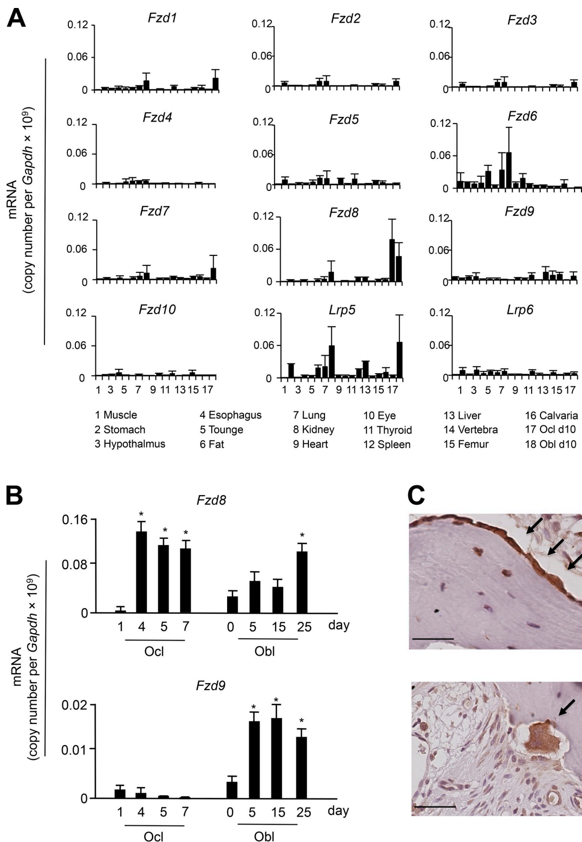
Figure 1. Fzd8 expression in bone cells. (A) qRT-PCR expression analysis for Wnt receptor-encoding genes using cDNA from various tissues and bone cells. Expression levels were normalized to Gapdh as indicated. Error bars represent mean ± SD ( n = 4 ). (B) qRT-PCR expression analysis for Fzd8 and Fzd9 during the course of osteoclast and osteoblast differentiation. Error bars represent mean ± SD ( n = 4 ). Asterisks indicate statistically significant differences compared with the earliest stage of differentiation. (C) Immunohistochemistry on human bone sections demonstrates the presence of FZD8 in osteoblasts (top) and osteoclasts (bottom). Bars, 25 \mu m.
