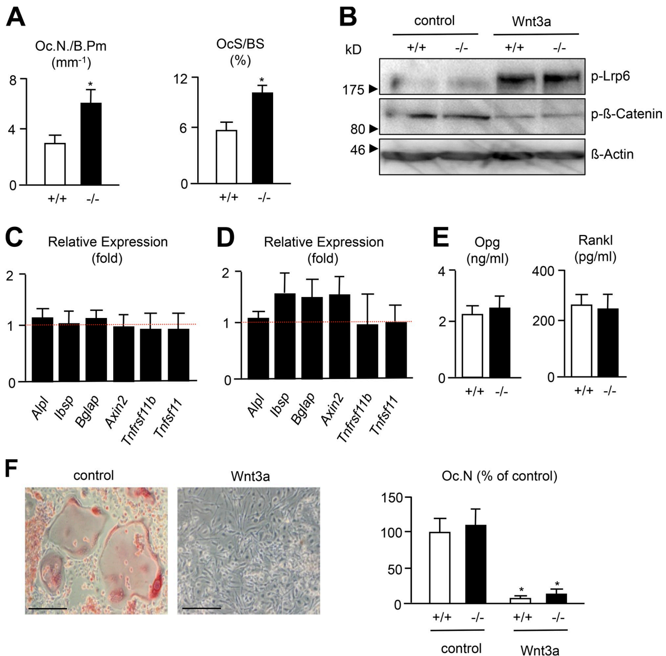
Figure 3. Increased osteoclastogenesis in Fzd8 -deficient mice. (A) Quantification of osteoclast number per bone perimeter (Oc.N/B.Pm) and osteoclast surface per bone surface (OcS/BS) in 24-wk-old wild-type and Fzd8 -deficient mice. Error bars represent mean \pm SD ( n = 6 ). Asterisks indicate statistically significant differences between the two groups. (B) Western blot analysis for phosphorylated Lrp6 and \beta -catenin after stimulation of wild-type and Fzd8 -deficient osteoblasts by Wnt3a at day 10 of differentiation. The black arrows indicate the position and molecular weight of the nearest marker. (C) qRT-PCR expression analysis of the indicated genes in Fzd8 -deficient osteoblasts relative to wild-type cultures. Error bars represent mean \pm SD ( n = 4 ). (D) qRT-PCR expression analysis of the same genes in Fzd8 -deficient marrow-flushed bones relative to wild-type littermates. Error bars represent mean \pm SD ( n = 4 ). (E) Serum levels of Opg and Rankl in 24-wk-old wild-type and Fzd8 -deficient littermates. Error bars represent mean \pm SD ( n = 6 ). (F) TRAP activity staining of bone marrow cells differentiated in the presence of M-CSf and Rankl with or without Wnt3a as indicated. Bars, 50 \mu m. Quantification of TRAP-positive multinucleated cells in wild-type and Fzd8 -deficient cultures is given on the right. Error bars represent mean \pm SD ( n = 6 ). Asterisks indicate statistically significant differences compared with control-treated cells.
