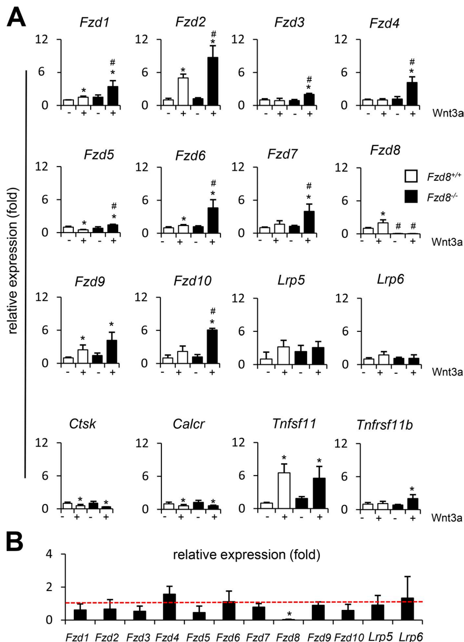
Figure 4. Compensatory induction of Fzd genes in Wnt3a-treated Fzd8 -deficient osteoclast cultures. (A) qRT-PCR expression analysis of the indicated genes in wild-type and Fzd8 -deficient bone marrow cultures differentiated in the presence of M-CSf and Rankl with or without Wnt3a as indicated. Error bars represent mean \pm SD ( n = 4 ). Asterisks indicate statistically significant differences compared with control-treated cells. Number signs indicate statistically significant differences between wild-type and Fzd8 -deficient cultures. (B) qRT-PCR expression analysis of the indicated genes in Fzd8 -deficient marrow-flushed bones relative to wild-type littermates. Error bars represent mean \pm SD ( n = 4 ).
