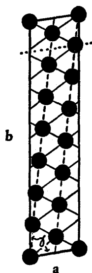
FIG. 5. The actin-net cell. Cell elements a , b , and \gamma are 82 Å, 406 Å, and 82^\circ , respectively, for dry samples. The dotted line shows how the cell is shortened ( b' = 351 \text{ \AA} ) if k' rather than k indices are adopted. Solid circles denote nodes, whose primitive connection is shown by light continuous lines; the outline of the non-primitive cell is heavy. Dashed lines show the nodal connection preferred for the actin "rods" in the Discussion section.
