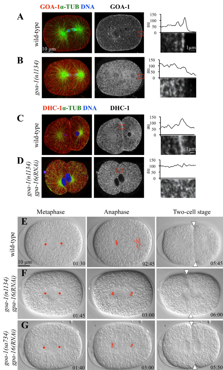
Figure 4. G\alpha is required at the membrane to direct spindle positioning in C. elegans embryos. (A and B) Wild-type (A) or goa-1(n1134) (B) one-cell stage embryos stained with antibodies against GOA-1 and \alpha -tubulin. Higher magnifications of cortical regions (red boxes) and accompanying line scans of representative embryos are given as in Fig. 3 and highlight the presence (A) or absence (B) of GOA-1. 10 cells were scored for each condition. (C and D) Wild-type (C) or goa-1(n1134) gpa-16(RNAi) (D) two-cell stage embryos stained with antibodies against DHC-1 and \alpha -tubulin. Higher magnifications of cortical regions (red boxes) and accompanying line scans of representative embryos are given as in Fig. 3 and highlight the presence (C) or absence (D) of DHC-1. 10 cells were scored for each condition. (E–G) Images from time-lapse DIC microscopy of C. elegans embryos from metaphase in the one-cell stage (left) through anaphase in the one-cell stage (middle) and in the early two-cell stage (right) from the wild-type (E), goa-1(n1134) gpa-16(RNAi) (F), and goa-1(sa734) gpa-16(RNAi) (G; see also corresponding Video 6). Symbols and tracking as described in the legend of Fig. 3. Red discs and white triangles indicate the position of centrosomes during metaphase and the cleavage furrow, respectively. Note equal size of blastomeres in goa-1(n1134) gpa-16(RNAi) (F) and goa-1(sa734) gpa-16(RNAi) (G) embryos. Time is given in minutes and seconds. au, arbitrary unit; \alpha -TUB, \alpha -tubulin.
