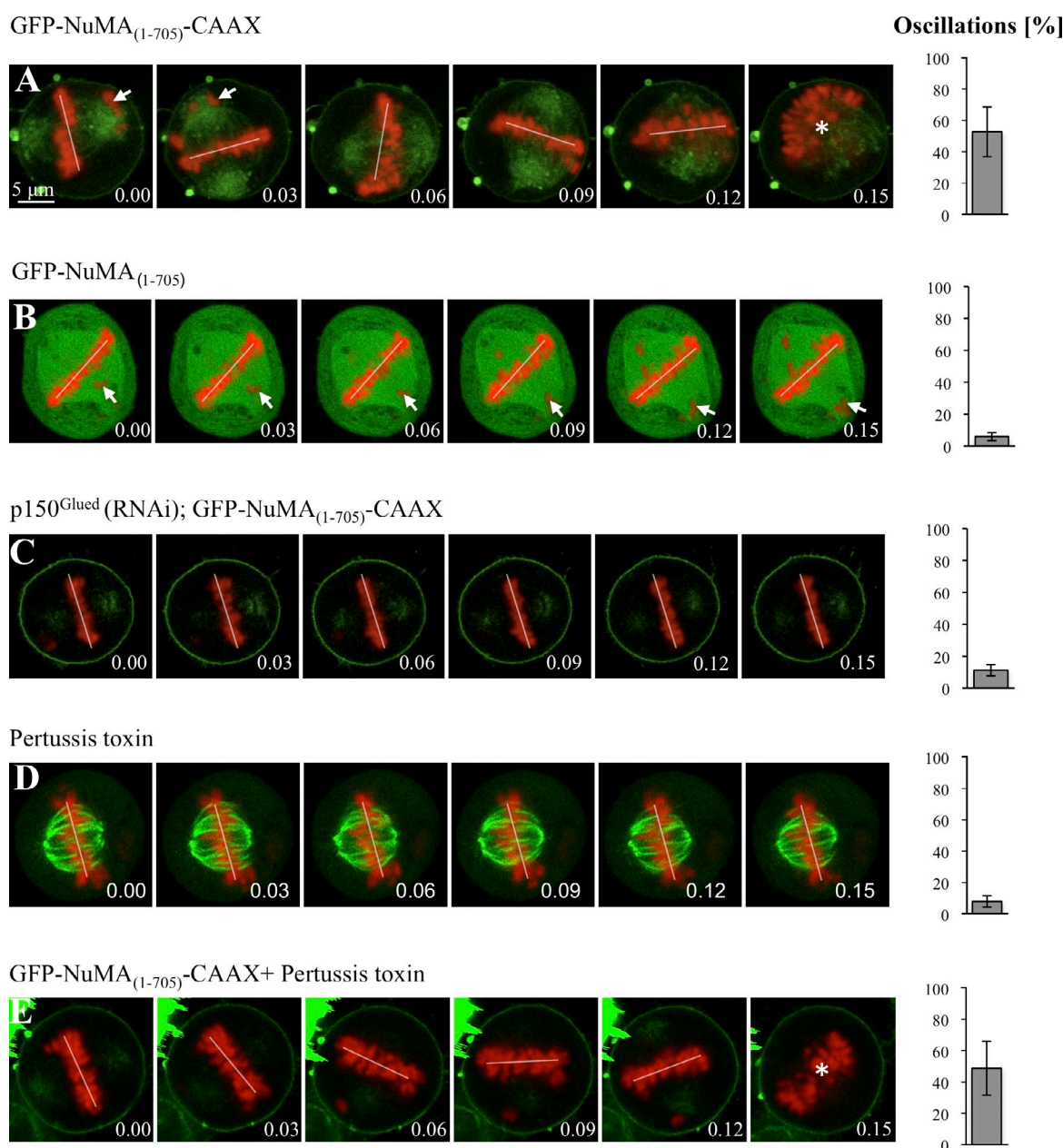
Figure 7. Dynein anchored at the plasma membrane is sufficient for directing spindle positioning in HeLa cells. (A–E) Images from time-lapse microscopy of metaphase HeLa Kyoto cells stably expressing GFP- \alpha -tubulin as well as mCherry-H2B, transfected with GFP-NuMA(1–705)-CAAX (A), GFP-NuMA(1–705) (B), or GFP-NuMA(1–705)-CAAX and p150 Glued siRNAs (C), treated with pertussis toxin (D), or transfected with GFP-NuMA(1–705)-CAAX and also treated with pertussis toxin (E; see also corresponding Videos 7 and 8). Arrows point to misaligned chromosomes. Spindle positioning is monitored as explained for Fig. 2, with time indicated in hours and minutes. Given that chromosome congression was impaired upon GFP-NuMA(1–705)-CAAX overexpression, we also analyzed spindle oscillations using the GFP- \alpha -tubulin signal in this case, with an indistinguishable outcome (oscillations 52 \pm 7\% SEM). 10 cells were analyzed for each condition. The extent of spindle oscillations upon overexpression of GFP-NuMA(1–705)-CAAX does not differ statistically from that upon overexpression of GFP-NuMA(1–705)-CAAX plus pertussis toxin (A vs. E, two-tailed Student's t tests; P = 0.39 ). Similarly, the values in GFP-NuMA(1–705)-CAAX and p150 Glued siRNA (C), as well GFP-NuMA(1–705) (B), are not statistically different from those in the control condition (Fig. 2 A); P = 0.74 and P = 0.20 , respectively. In contrast, the values in GFP-NuMA(1–705)-CAAX and p150 Glued siRNA (C) are statistically different from those of GFP-NuMA(1–705)-CAAX overexpression alone (A; P < 0.0005 ). The position of chromosomes is indicated by a white line when chromosomes are within the imaging plane and by an asterisk when the metaphase plate is no longer in the plane of view.
