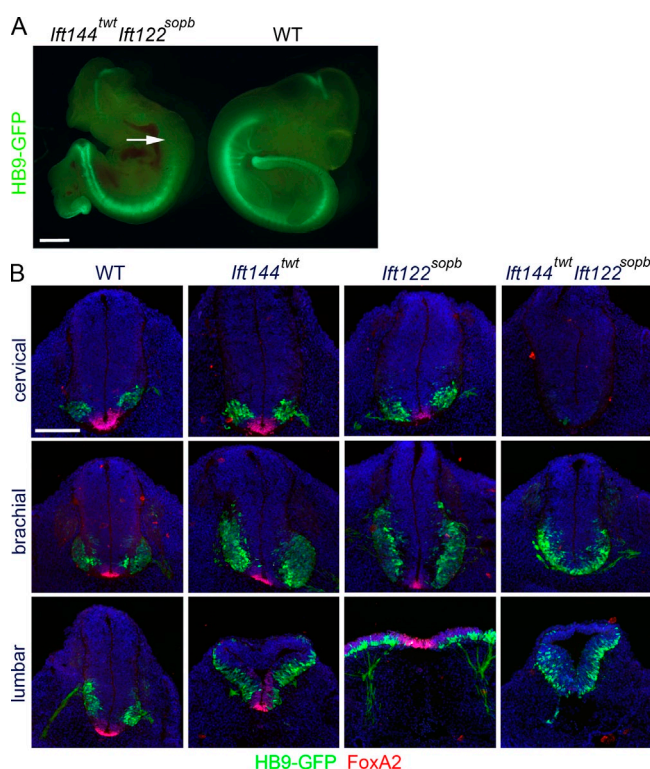
Figure 5. Neural patterning in Ifi144 twi Ifi122 sob double mutants resembles that in Ifi144 dmhd . (A) Based on expression of HB9-GFP, Ifi144 twi Ifi122 sob double-mutant embryos lack motor neurons in the anterior spinal cord (arrow) but retain them in caudal regions. The double mutants are exencephalic and have laterality defects, similar to Ifi144 dmhd . WT, wild type. (B) Cross-sections through Ifi144 twi , Ifi122 sob , and Ifi144 twi Ifi122 sob double-mutant embryos at E10.5, marked by the expression of HB9-GFP and FoxA2. Ifi144 twi Ifi122 sob double mutants lack FoxA2+ floor plate cells at all levels, lack cervical motor neurons, and show dorsally expanded motor neurons at lumbar levels, like Ifi144 dmhd . Bars: (A) 1 mm; (B) 200 \mu m.
