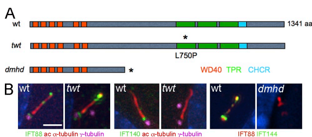
Figure 2. Two mutations in mouse Ift144 affect cilia structure. (A) Schematic drawing of how the mutations affect protein structure. Two isoforms of the 1,341-amino acid WDR19/IFT144 protein have been described; conserved protein–protein interaction motifs are shown in colored boxes. Depending on the isoform, the dmhd splice site mutation would truncate the protein at amino acid 592 (ENSMUSP00000038098) or amino acid 543 (ENSMUSP000000109414). The twf mutation causes a leucine-to-proline substitution in the first tetratricopeptide repeat (TPR; Ashe et al., 2012). Asterisks indicate the position of the sequence changes in the mutant proteins. CHCR, clathrin heavy chain repeat; wt, wild type. (B) Altered cilia protein expression and structure in the mutants. Cilia in twf MEFs are of approximately normal length and width but accumulate higher than normal levels of IFT88 (an IFT-B protein) at cilia tips and lack detectable IFT140 (an IFT-A protein; 0/9 twf cilia were positive for IFT140 compared with 13/14 wild-type cilia). Cilia in dmhd MEFs are short and wide; they accumulate IFT88 but lack any detectable IFT144 protein, consistent with the hypothesis that dmhd is a null allele (0/18 were positive for IFT144). ac, acetylated. Bar, 2 \mu m.
