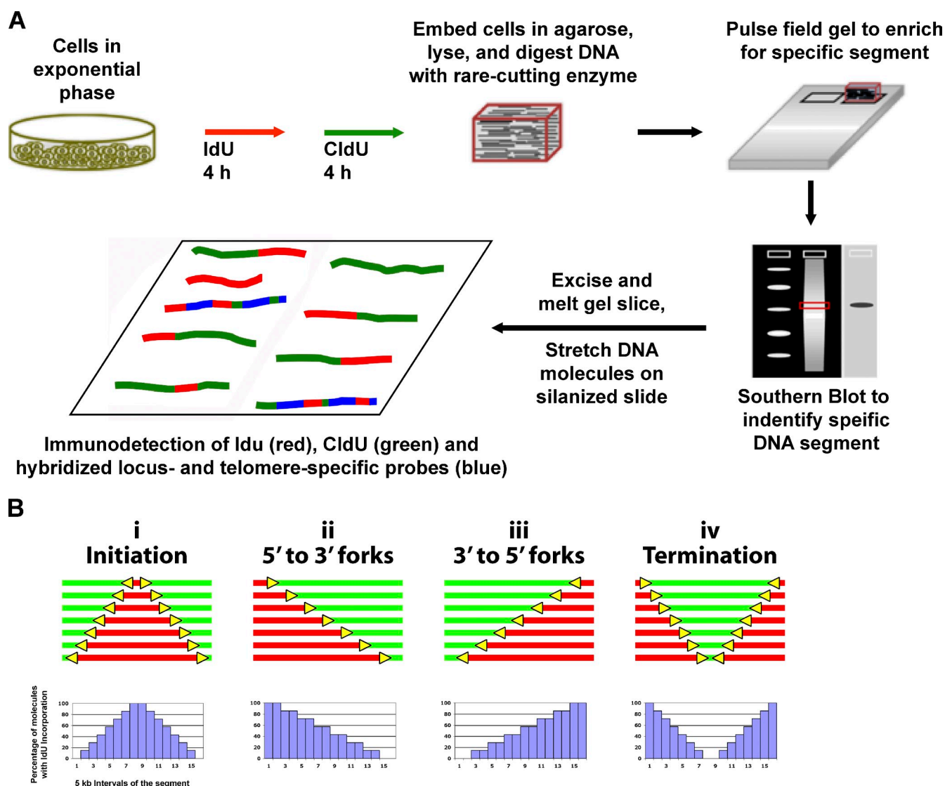
Figure 1. SMARD. (A) Exponentially growing cells were labeled with the halogenated nucleosides IdU for 4 h followed by CldU for 4 h. Genomic DNA was then isolated. To avoid the breakage of large molecules, the cells were embedded in agarose. We used rare cutting restriction endonucleases to obtain unique large molecules of genomic DNA, which were separated by pulse field gel electrophoresis to enrich by size for the particular subtelomere segments of interest. Southern blotting was performed to identify the target segment within the gel, which was excised. The gel slice containing the segment of interest was melted and the enriched DNA in the melted gel solution was stretched on silanized glass slides. Fluorescent antibodies were used to identify regions where IdU (red) or CldU (green) were incorporated into the DNA. Immunodetected biotinylated FISH probes (blue) were used to identify the target molecules and to align the images of individual molecules to produce a composite profile of replication. (B) Specific replication events are identified by characteristic patterns in the aligned molecule images. DNA molecules with increasing red stain from one end indicate replication forks progressing in a single direction through the aligned region (ii and iii). Initiation events are indicated by a red tract flanked on both sides by green (i), whereas a green tract flanked on both sides by red (iv) indicates a termination event. Molecule alignments can be graphically depicted as histograms of the percentage of IdU incorporation along each 5 kb of a segment. Specific replication events produce characteristic features in these replication profiles. Positions of the centers of initiation zones are indicated by peaks (i), whereas termination events are indicated by valleys (iv). Replication progressing through the segment primarily in one direction (5' to 3' or 3' to 5') from an external origin is observed as a progressive decrease in the percentage of IdU incorporation from one end to the other across the segment (x axis; ii and iii).
