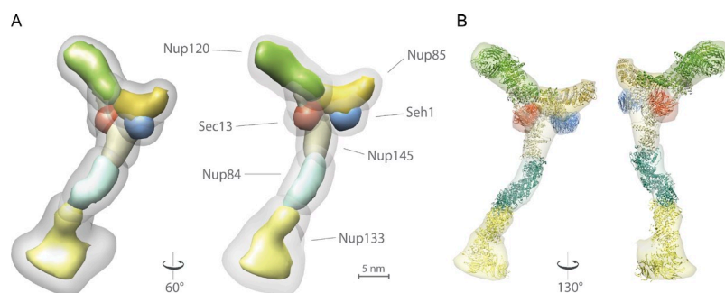
Figure 5. Density map for the Nup84 complex ensemble.
