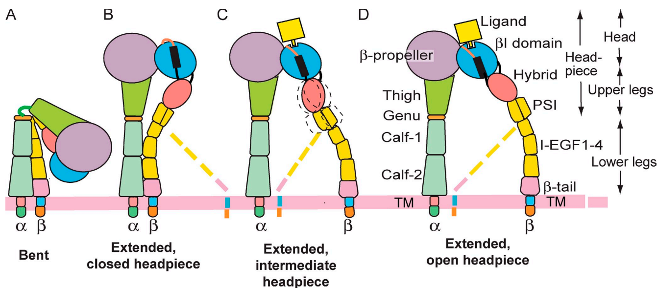
Figure 1. Schematic of integrin domain organization and conformational states. The pink loop and black bar in B–D represent the \beta 6 - \alpha 7 loop and \alpha 7 -helix of the \beta I domain, respectively. Broken lines symbolize lower \beta leg flexibility. The intermediate headpiece state is shown here for the first time.
