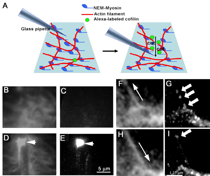
Figure 2. Binding of cofilin to actin filaments. (A) A schematic drawing of the experimental setup. (B–E) Time-lapse imaging of rhodamine-labeled actin filament meshwork (B and D) and IAF-labeled cofilin (C and E). (B) A meshwork of F-actin observed with TIRF microscopy before severing. (C) An IAF-labeled cofilin image acquired during 1 s with TIRF illumination. (D) A meshwork of F-actin severed by a tip of a glass pipette (arrow). (E) Cofilin images acquired during 3 s after the meshwork was severed. The arrow shows the tip of the pipette. (F) The actin bundle was relieved to the original length by displacing the tip of pipette in the direction shown by the arrow. (G) A high accumulation level of cofilin-positive spots was observed along the actin bundle 4 s after relieving a strain (Video 4). (H) A bundle of actin filaments was stretched ~20% by displacing the tip of the pipette attached to one end of the bundle in the direction shown by the arrow. (I) A few cases of binding of cofilin to the stretched bundle were observed (cofilin fluorescent spots are shown by the arrows in G and I). Images of IAF-cofilin were accumulated during 4 s (see also Video 5). Bars: (E) 5 \mu\text{m} ; (I) 1.25 \mu\text{m} .
