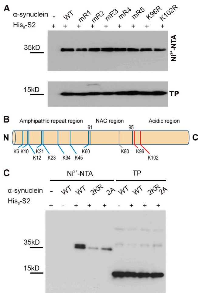
Figure 3. K96 and K102 are the major sumoylation sites of α-synuclein. (A) α-Synuclein is sumoylated at multiple lysine residues. Sumoylation of α-synuclein was analyzed in HEK293T cells by cotransfection of His 6 -SUMO2 with WT myc-tagged α-synuclein or one of the indicated lysine-to-arginine mutants (mR1: K6, 10, and 12R; mR2: K21 and 23R; mR3: K32 and 34R; mR4: K43 and 45R; and mR5: K58, 60R, K96R, and K102R), followed by Ni 2+ -NTA chromatography. None of the mutations resulted in abolished α-synuclein sumoylation. Total protein (TP) levels of WT α-synuclein and the respective mutants are shown in the bottom panel. Samples were analyzed by immunoblotting with anti-myc antibody (9E10). (B) Summary of α-synuclein sumoylation sites. MS analysis of sumoylated α-synuclein (obtained upon sumoylation in bacteria; see Materials and methods) revealed 11 SUMO-conjugated lysine residues (8 lysines in the N-terminal amphipathic region, 1 lysine in the hydrophobic NAC region, and the 2 lysines in the C-terminal acidic region; Fig. S2 and supplemental data). Nonconsensus lysines are depicted in blue, and the consensus and consensus sequence-related sites are in red. (C) The sumoylation levels of myc-tagged WT, 2KR (K96R and K102R), and 2A (D98A and E104A) mutants were compared using Ni 2+ -NTA chromatography. Elution samples and total lysates (TP) in A and C were run on a 4–12% NuPAGE Bis-Tris gel and analyzed by immunoblotting with myc antibody (clone 9E10). Sumoylated α-synuclein runs as a doublet band on gradient SDS-PAGE.
