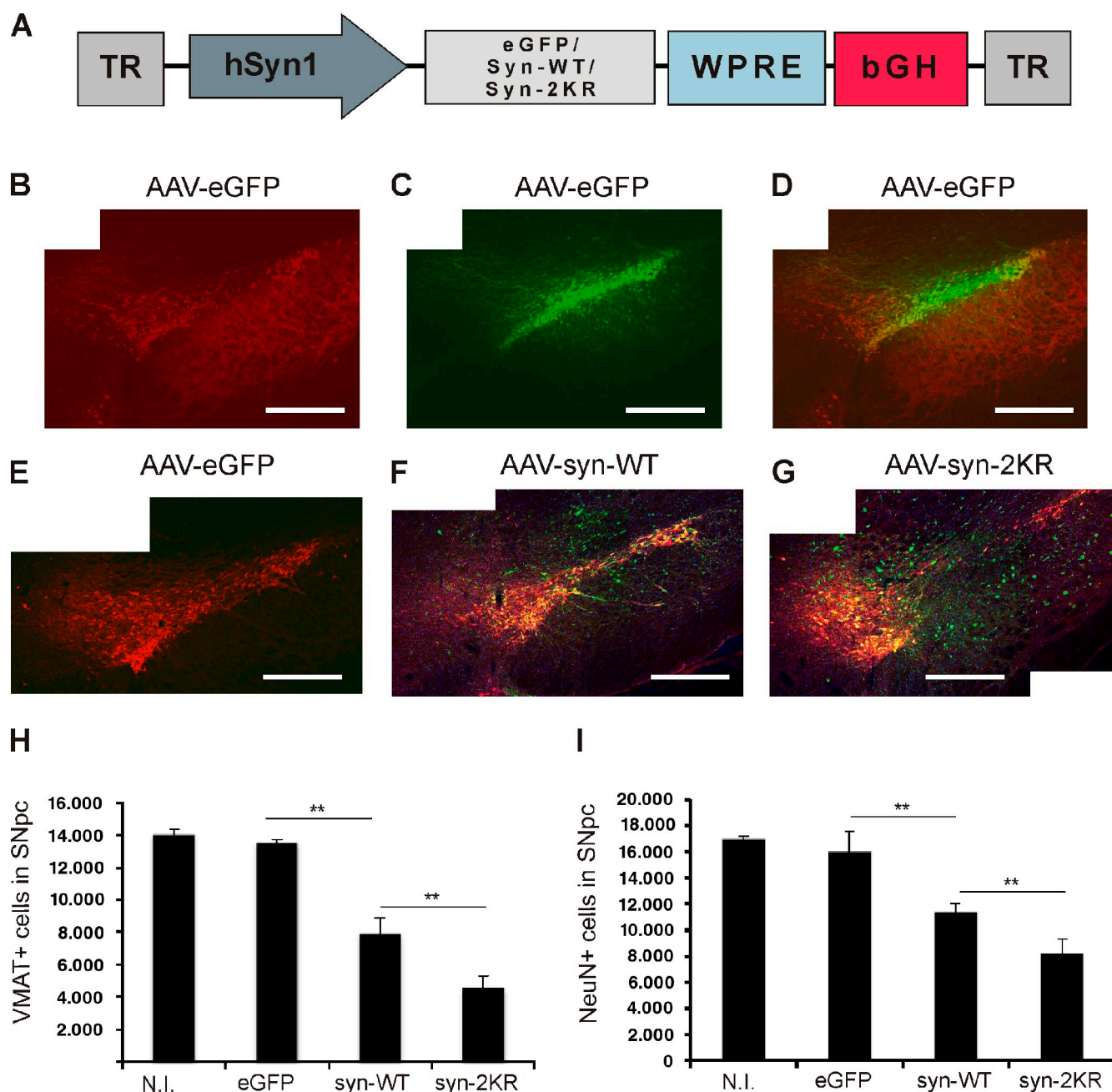
Figure 5. Reduced sumoylation exacerbates \alpha -synuclein neurotoxicity in vivo. (A) A schematic representation of vector genomes used in the in vivo rat model of PD. Recombinant adeno-associated viral vectors (AAV2) express either EGFP, WT \alpha -synuclein (syn-WT), or \alpha -synuclein K96R and K102R (syn-2KR) under the control of neuron-specific human synapsin 1 gene promoter (hSyn1). Vectors also encode inverted terminal repeats (TR) and small control elements woodchuck hepatitis virus posttranscriptional control element (WPRE) and bovine growth hormone (bGH)-derived polyadenylation site. (B) VMAT2-positive (VMAT2 + ) neurons (red) in the left SN. (C) rAAV2-mediated GFP transduction of SNpc. (D) Overlay of VMAT2 + and GFP-transduced neurons in the left SN. (E–G) Coimmunostaining of VMAT2 + (red) and human \alpha -synuclein (green). Survival of VMAT2 + neurons in SNpc of animals injected with rAAV2 vectors expressing EGFP (E), human WT \alpha -synuclein (F), or \alpha -synuclein-2KR (G). Panels B–G are each a composite of two separate fluorescent images (AxioPlan2 with a 5x objective and AxioVision 4.7). (H and I) Respective unbiased stereological quantification of surviving VMAT2 + (H) or NeuN + (I) cells in the transduced SNpc. The graphs display VMAT2 + or NeuN + cell numbers in animals injected with rAAV2 expressing EGFP, WT \alpha -synuclein (syn-WT), and \alpha -synuclein-2KR (syn-2KR). N.I., contralateral noninjected side. n = 6 –8 per experimental group. Results are mean \pm SEM. **, P < 0.01 , Student's t test. Bars, 0.5 mm.
