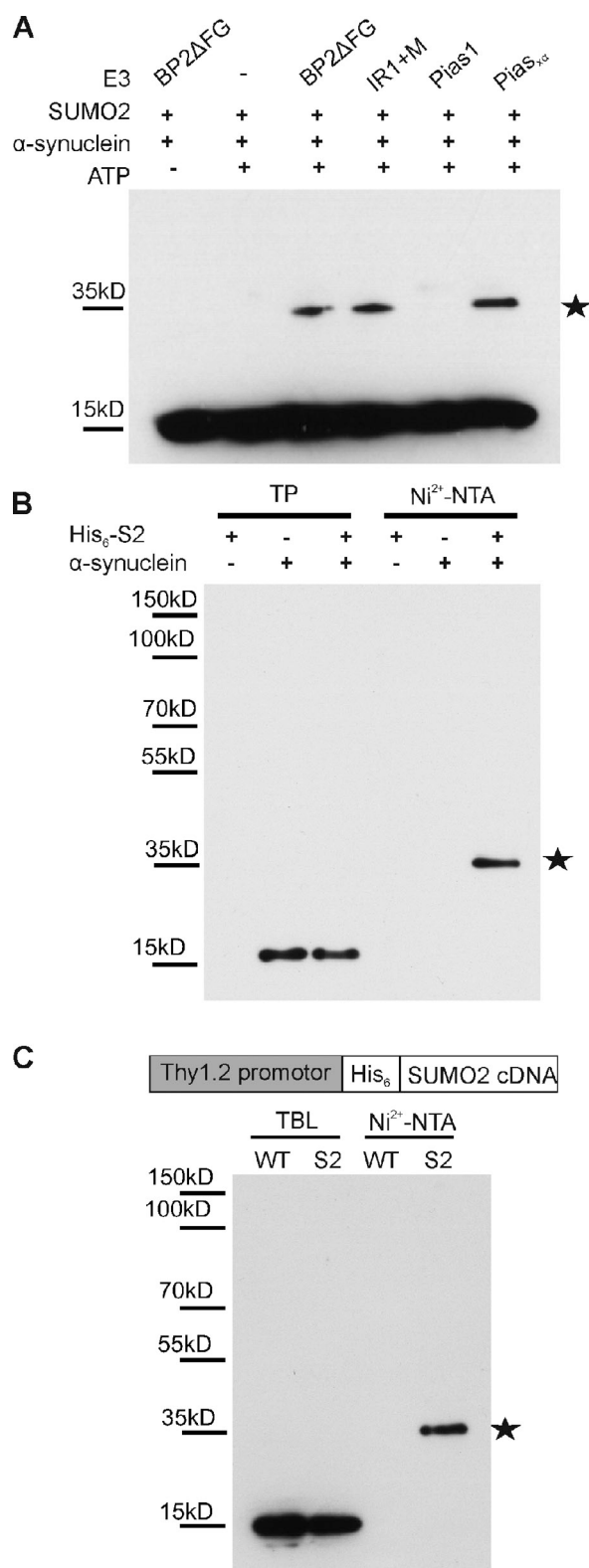
Figure 1. α-Synuclein sumoylation in vitro in cells and in mouse brain. (A) α-Synuclein is SUMO2 modified in vitro. 500 ng α-synuclein, 500 ng SUMO2, 150 ng Aos1/Uba2, 200 ng Ubc9, and 5–10 ng E3 ligase fragments were incubated for 30 min at 30°C with and without ATP in a volume of 20 μl. Reactions were stopped with SDS sample buffer before analysis by SDS-PAGE and immunoblotting with mouse monoclonal anti-α-synuclein antibody (Syn211; Invitrogen). (B) α-Synuclein modification by SUMO2 in HEK293T cells. Plasmids encoding His 6 -SUMO2 (His 6 -S2) or/and α-synuclein were transfected in HEK293T cells. SUMO substrates were purified by
