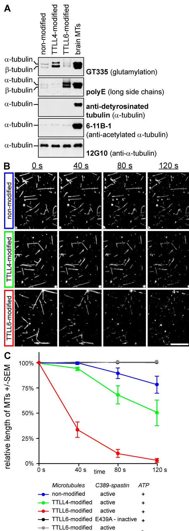
Figure 4. Microtubule polyglutamylation activates spastin-mediated severing in vitro. (A) Immunodetection of modification levels on purified tubulin that was copolymerized with 6.5% rhodamine-labeled brain tubulin. GT335 detects glutamylation irrespective of the side chain length, whereas
