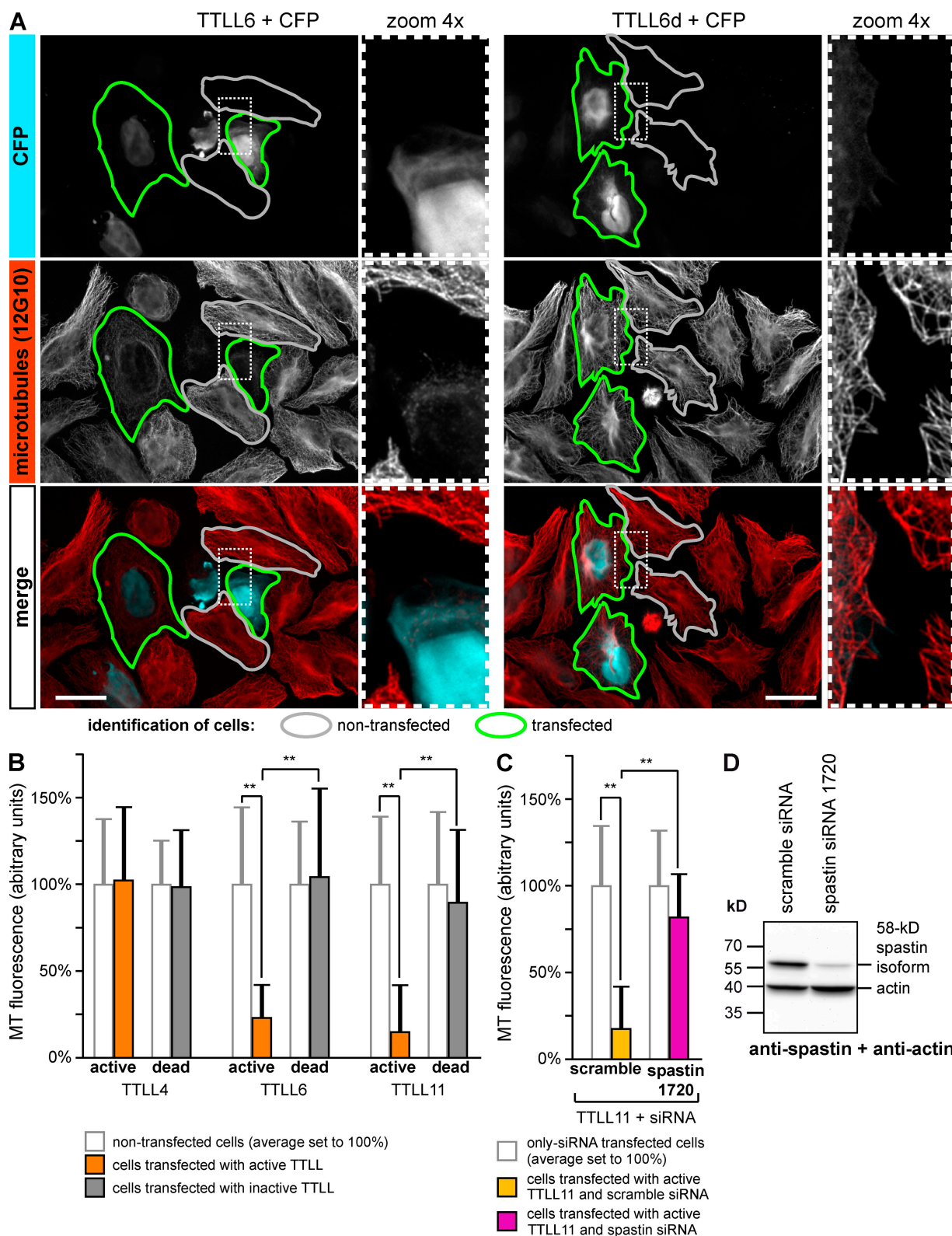
Figure 1. Polyglutamylation induces microtubule severing in HeLa cells. (A) MT morphology in HeLa cells expressing either active TLL6 or an inactive mutant (TLL6d). Transfected cells (green contours) were identified by CFP, which was coexpressed from the same plasmid (Fig. S2). Cells were stained with the general tubulin antibody 12G10, which detects \alpha -tubulin in a glutamylation-independent manner (not depicted). Gray contours indicate examples of untransfected cells. Bar, 20 \mu m. (B) Quantification of MT mass in cells expressing active and inactive TLL4, 6, and 11. Mean 12G10 fluorescence intensity was measured as indicated by contours in A for >30 cells per experimental condition and plotted as normalized to the mean of nontransfected cells (100%). Error bars indicate SD. Statistical significance was determined by two-tailed Student's t test. All P values (**) are below 10^{-10} . (C) Quantification as in B after expression of TLL11 in cells transfected with nonsilencing control (scramble) or spastin-specific siRNA 1720 (transfection scheme of siRNA; see Materials and methods). (D) Validation of spastin siRNA. HeLa cells were transfected with scramble and spastin siRNA, and actin and spastin levels were detected on the same blot with specific antibodies. The siRNA 1720 reduces the levels of spastin to 13.2%.
