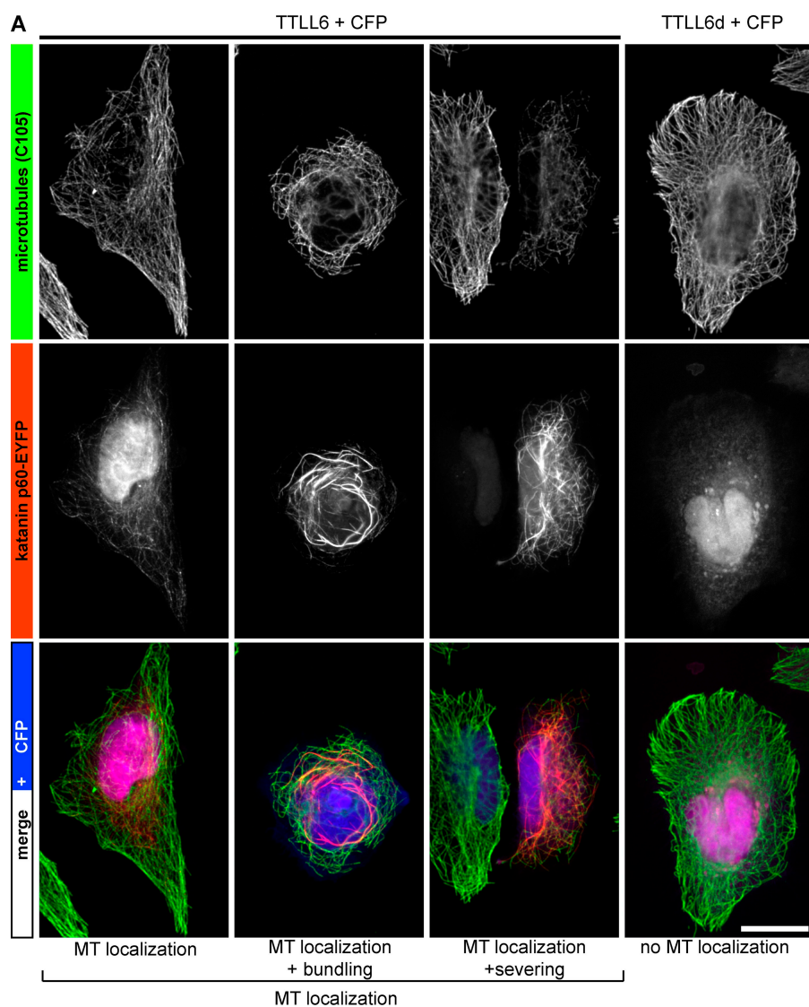
Figure 5. Effects of differential microtubule glutamylation on katanin p60. (A) U2OS cells were cotransfected with katanin p60-EYFP and either active TLL6 or an inactive mutant (TLL6d), with CFP as transfection control. Activation of katanin leads to MT localization of katanin p60, and sometimes to MT bundling and/or severing. Bar, 20 \mu m. (B) Fraction of cells showing colocalization of katanin p60-EYFP with MTs (all phenotypes as shown in A were compiled). A minimum of 200 cells was analyzed in three independent experiments. Error bars indicate SD.
