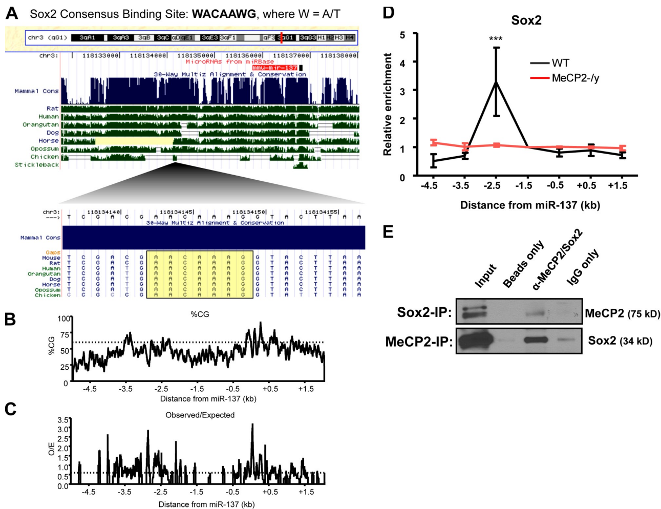
Figure 3. Transcriptional regulation of miR-137 involves coregulation by Sox2. (A) Schematic showing the miR-137 genomic locus and the location of a conserved Sox2 consensus-binding site within the 2.5-kb upstream region of miR-137 with which MeCP2 was also found to interact by ChIP. (B and C) Genomic structure and CpG content surrounding the miR-137 genomic locus. (B) Percentage of CG content across a 7-kb region surrounding miR-137, with a threshold indicated at 60%. (C) Ratio of observed CpG dinucleotides to the number of CpGs expected with a normal distribution across the same 7-kb region surrounding miR-137. A threshold is indicated at a ratio of 0.6 (dotted line). Data for both plots were generated using EMBOSS CpG plot with a 100-nt window size and a 1-nt window shift increment (Larsen et al., 1992). (D) Sequences 2.5 kb upstream of miR-137 enriched in a Sox2-specific ChIP relative to IgG only in WT aNSCs but not MeCP2-/y aNSCs, normalized to the directly adjacent 1.5-kb upstream region ( n = 3 , error bars indicate mean \pm SEM, two-way ANOVA, Bonferroni post-test; ***, P < 0.001 ). (E) MeCP2 and Sox2 could be coimmunoprecipitated. Either MeCP2 or Sox2 was immunoprecipitated and subjected to Western blots with anti-Sox2 or anti-MeCP2 antibodies, respectively. IP beads only and IP with normal IgG were used as negative controls.
