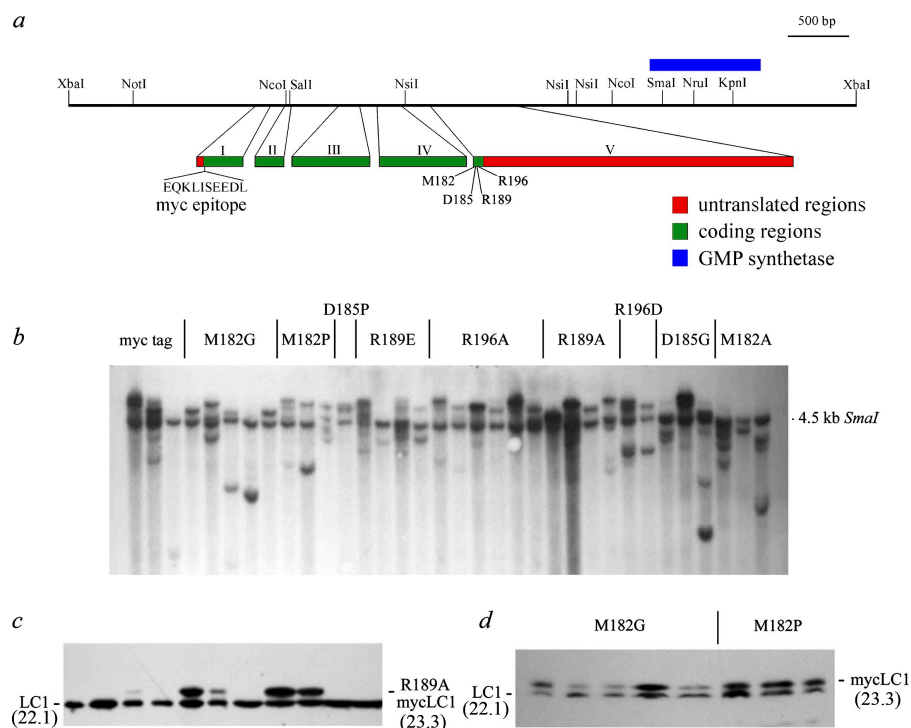
Figure 2. Expression of tagged mutant versions of LC1. (a) Map of the \sim 6.2 -kb LC1 genomic region, indicating the location of the five exons and the sites of myc tag insertion and mutagenesis. The genomic fragment also includes the gene for GMP synthetase. (b) Southern blot analysis of SmaI-digested genomic DNA from strains transformed with various mutant forms of LC1. The endogenous LC1 gene yields a SmaI fragment of \sim 4.5 kb (Benashski et al., 1999). The additional bands represent \geq 1 integrated copies of the tagged LC1 gene. (c) Immunoblot analysis of flagellar samples from 11 strains transformed with the R189A mutant LC1 gene. The myc-tagged LC1 protein is detectable in five strains. (d) Immunoblot analysis of selected M182G- and M182P-transformed strains. These strains were chosen for analysis, as they stably express approximately similar amounts of wild-type and mutant LC1 proteins.
